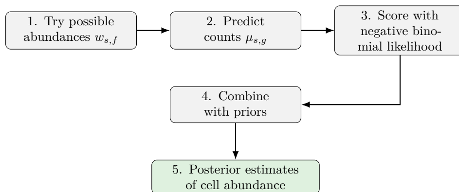
Figure 11: A beginner-level view of inference. The real algorithm is more advanced, but it follows this logic.
