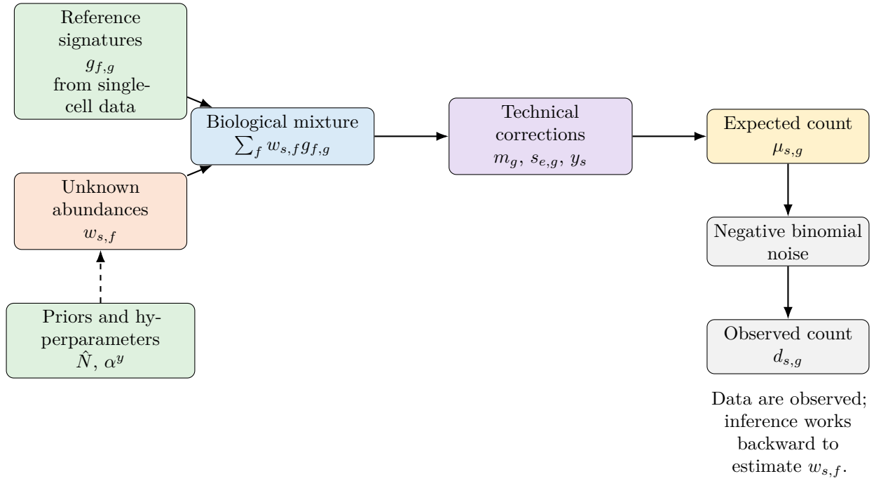
Figure 12: The cell2location model in one picture.
