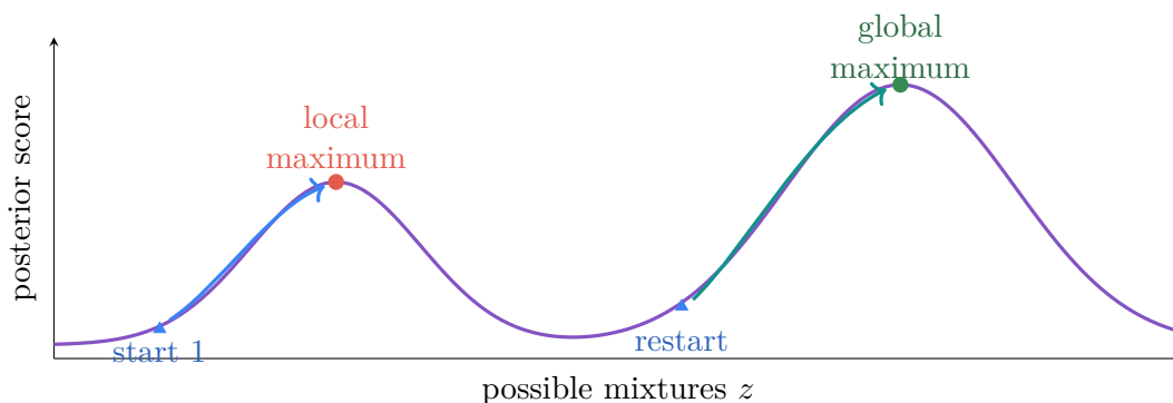
Figure 6: Schematic illustration: a slope-guided search can stop on the smaller hill. A different starting point may reach the higher hill. Real ShapeMix abundance space has one dimension per cell type, so its landscape cannot usually be drawn on paper.
