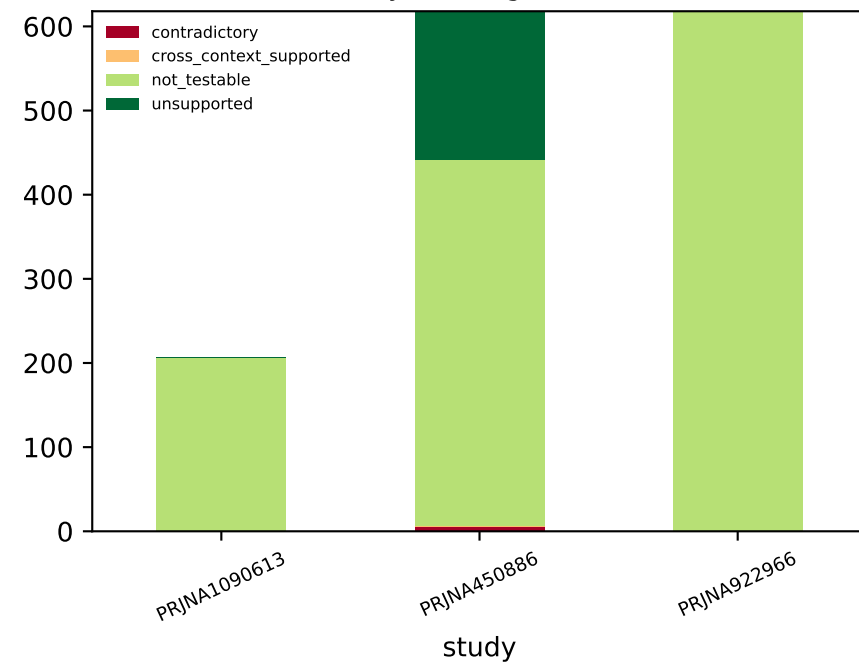
Cross-study frozen-gene outcomes
