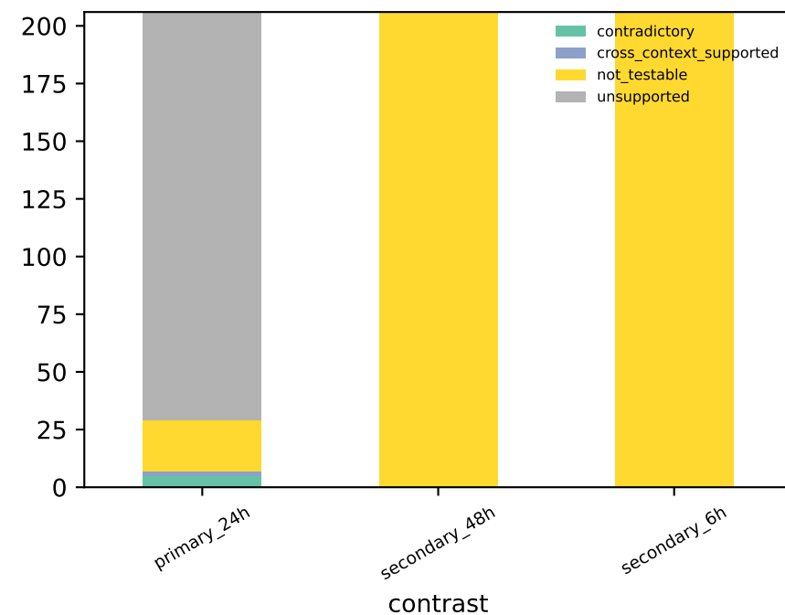
6/24/48-h evidence labels
