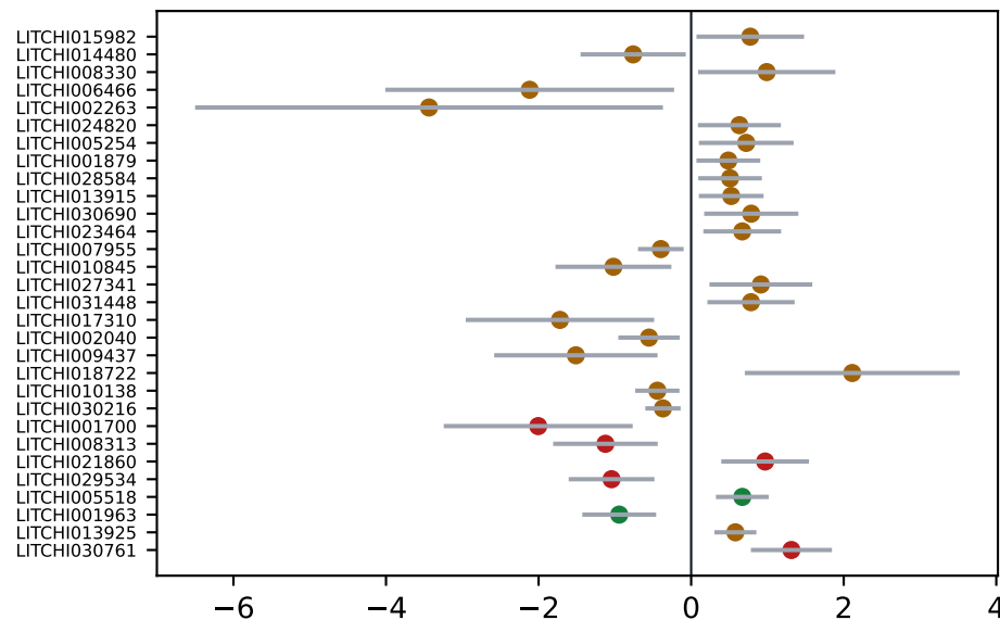
PRJNA450886 24-h frozen-gene forest
