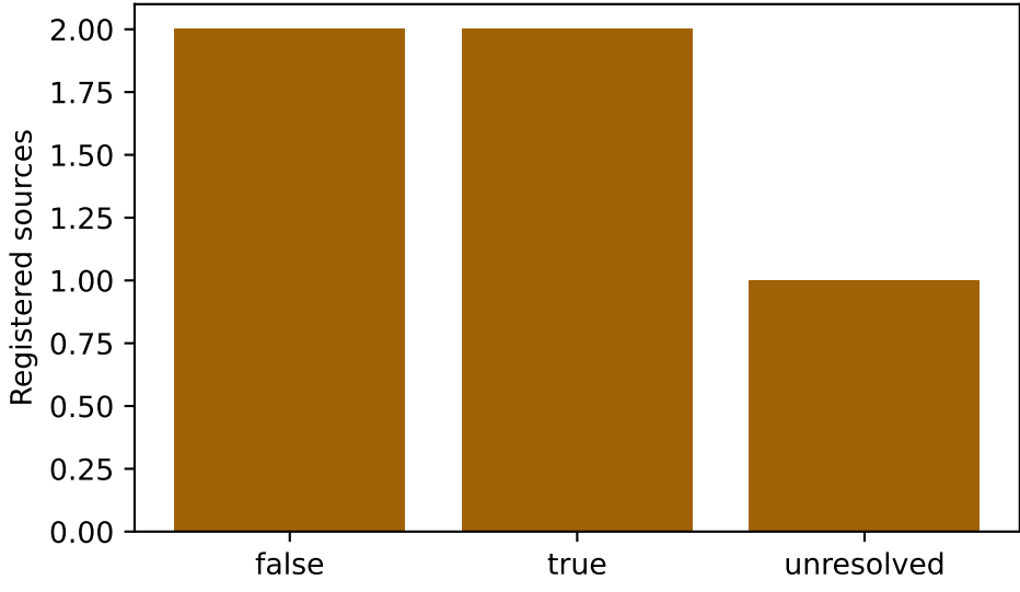
Published-evidence independence
