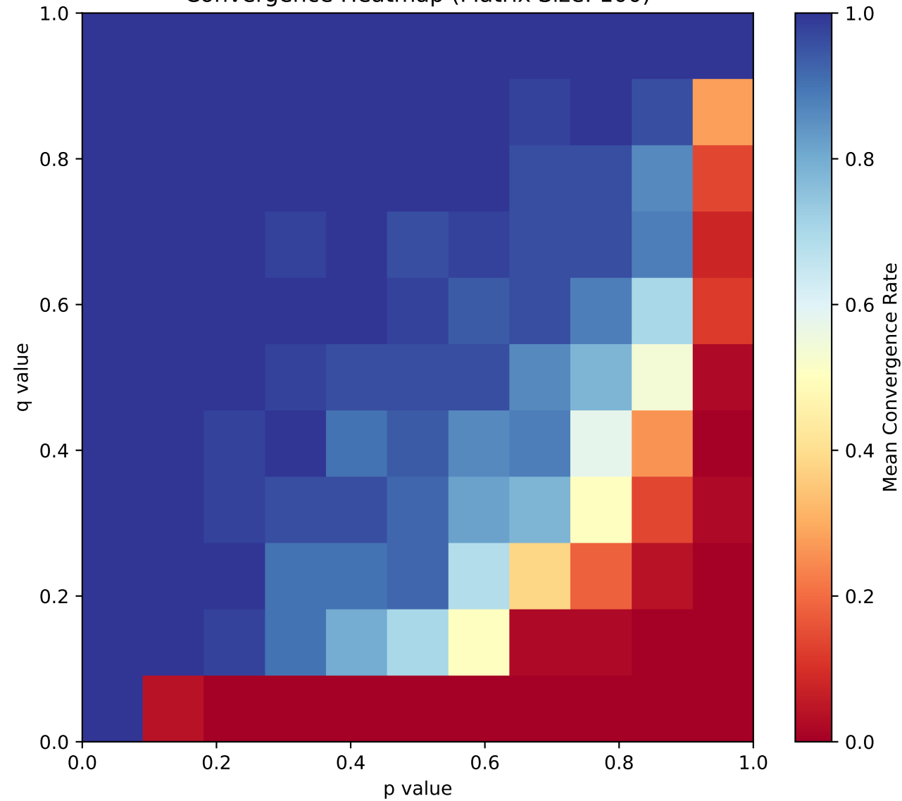
Convergence Heatmap (Matrix Size: 100)
