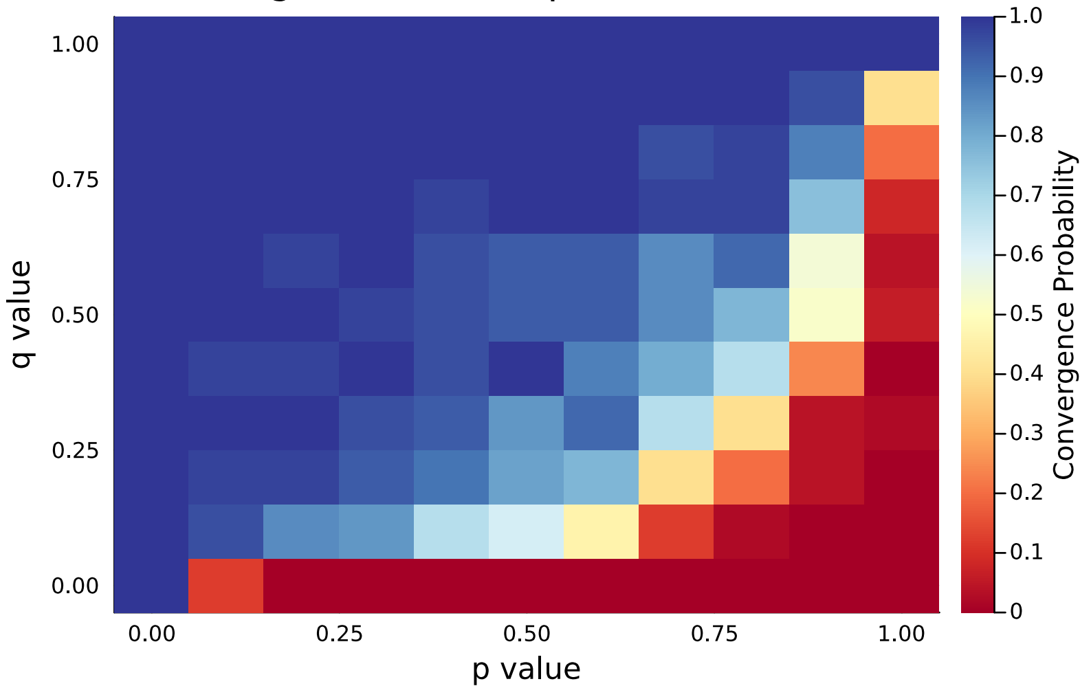
Convergence Heatmap (Matrix Size: 100)
