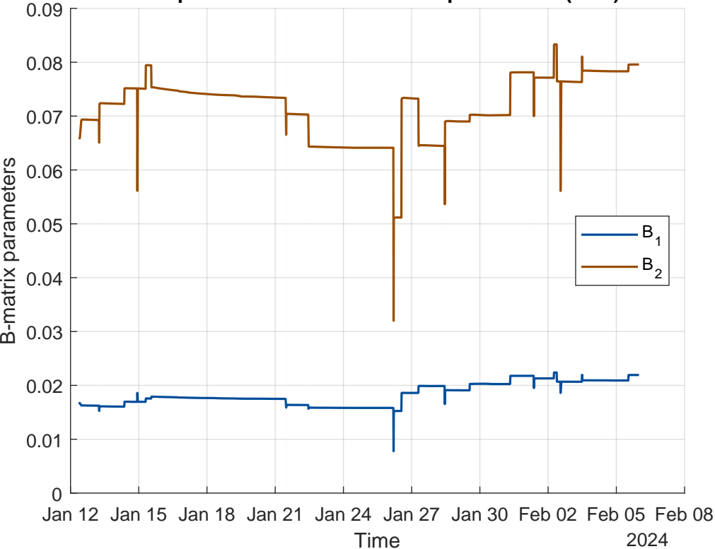
Temporal evolution of B-matrix parameters (RLS)
