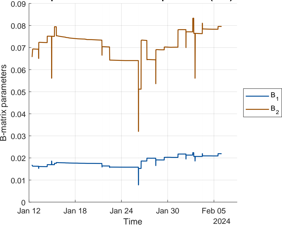
Temporal evolution of B-matrix parameters (RLS)
