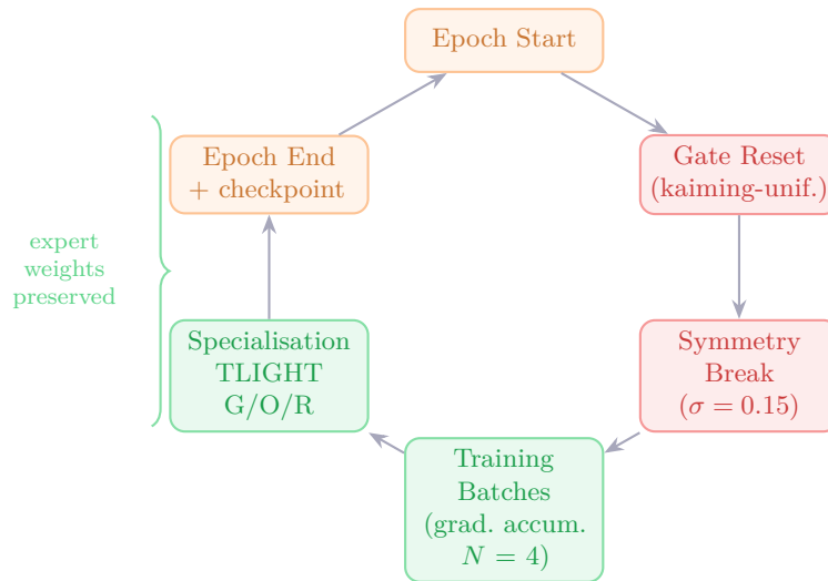
Figure 2: Epoch-Gated Routing Lottery lifecycle. All gate weights are reset to kaiming-uniform at every epoch boundary; Gaussian noise ( \sigma = 0.15 ) is applied to all 576 expert tensors to prevent dead-expert inertia. Expert weights are preserved throughout—only the routing map is redrawn. Gradient accumulation ( N=4 ) operates within the training phase.
