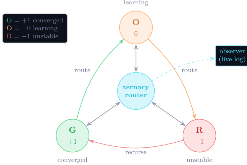
Figure 1: TLIGHT as recursive ternary routing . A central router dispatches each expert’s state through the balanced-ternary triad—G (+1, converged), O (0, actively learning), R (−1, unstable)—with bidirectional radial routing to the hub and a recursive cycle (+1 → 0 → −1 → +1) around the periphery; the observation layer reads the live (G, O, R) vector each step. Unlike a flat state machine, every state re-enters the ternary decision through the hub rather than only stepping to a neighbour.
