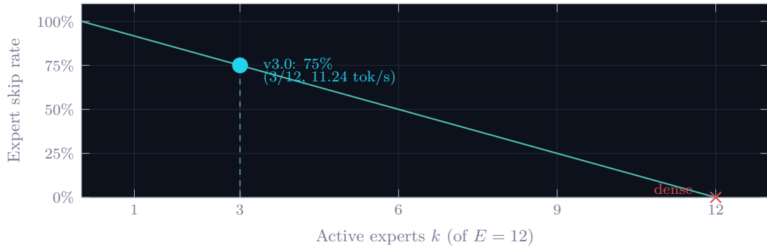
Figure 3: @sparseskip expert skip rate = 1 - k/E as a function of active experts k for E = 12 . The curve is exact—no approximation is introduced by skipping, since \text{mul}(a, 0) = 0 \forall a \in T (Eq. 3). The v3.0 operating point (Top-3, cyan marker) achieves 75% skip at 11.24 tok/s on a 2013 consumer CPU.
