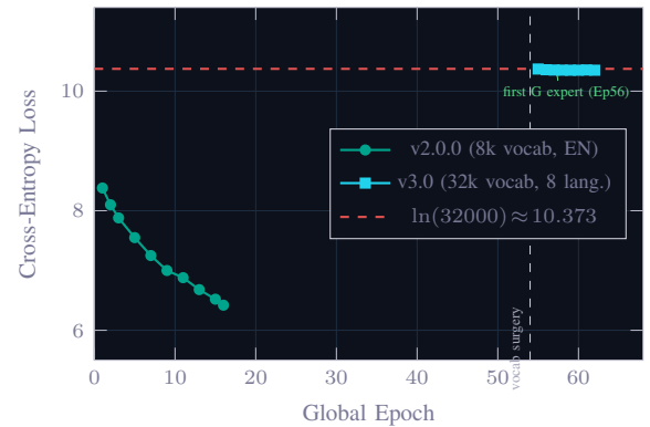
Fig. 4. Loss trajectories for v2.0.0 (English, 8k vocab, 16 epochs) and v3.0 (multilingual, 32k vocab, Global Epochs 55–62). The dashed line marks the 32k random baseline H_{\text{random}} = \ln(32000) \approx 10.373 ; the v3.0 plateau lies below it, confirming the model extracts multilingual structure despite the post-surgery vocabulary transfer regime. First Green expert (G state in TLIGHT) appears at Global Epoch 56.
