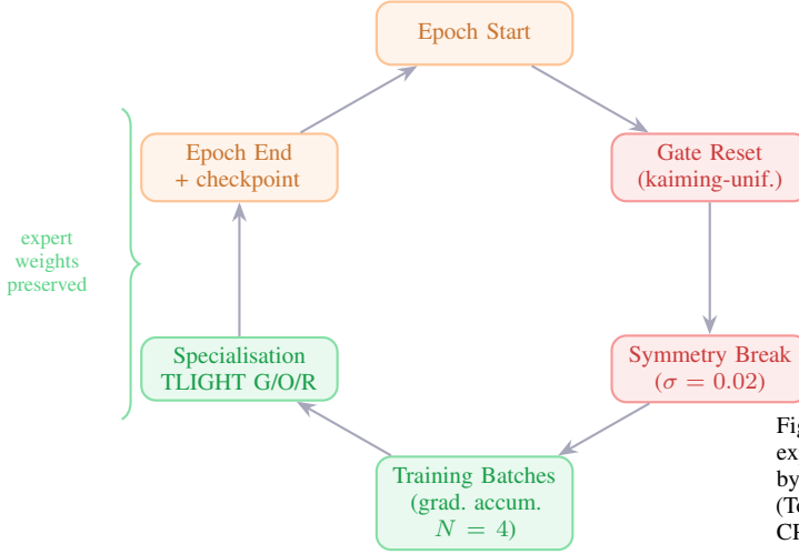
Fig. 2. Epoch-Gated Routing Lottery lifecycle. All gate weights are reset to kaiming-uniform at every epoch boundary; Gaussian noise ( \sigma = 0.02 ) is applied to all 576 expert tensors to prevent dead-expert inertia. Expert weights are preserved throughout—only the routing map is redrawn. Gradient accumulation ( N = 4 ) operates within the training phase.
