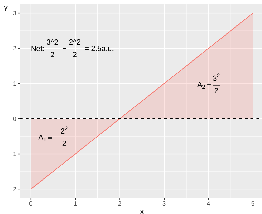
Figure 13.5: Area above and under the x -axis
