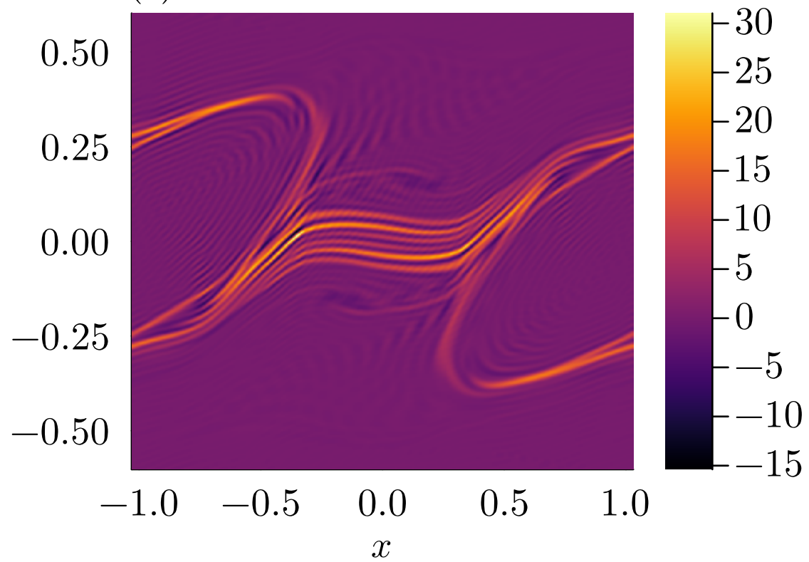
(c) \varepsilon = 10^{-7}
