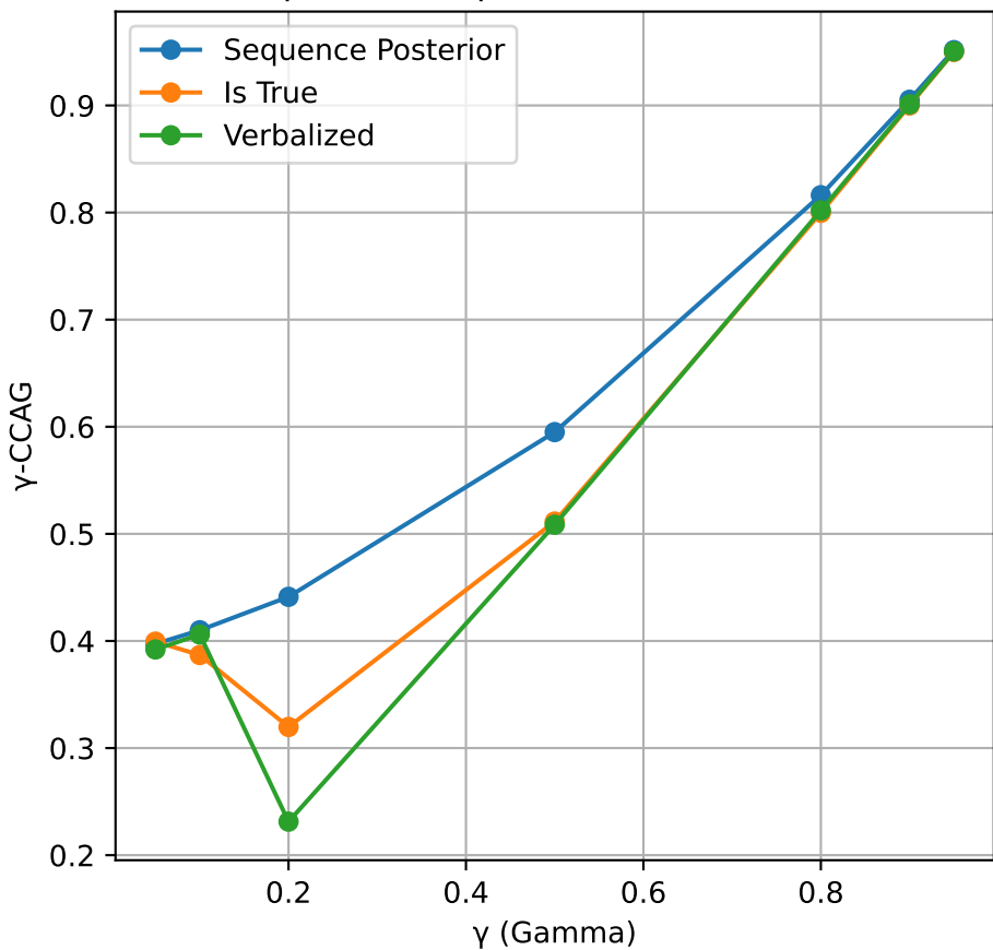
\gamma -CCAG vs \gamma for GLM-4.6V-Flash
