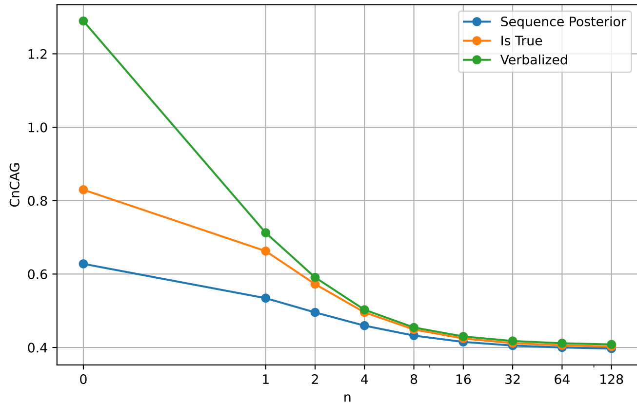
CnCAG vs n for GLM-4.6V-Flash
