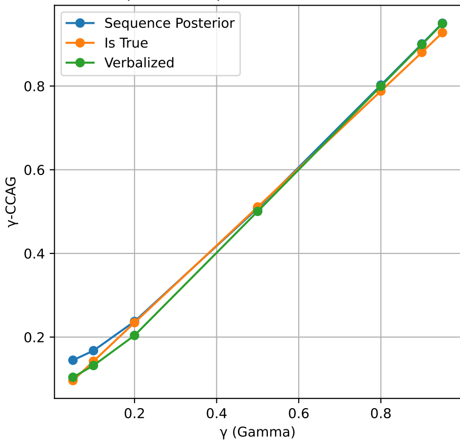
\gamma -CCAG vs \gamma for Gemini 2.5 Flash
