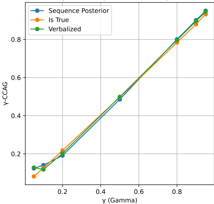
\gamma -CCAG vs \gamma for Gemini 2.5 pro
