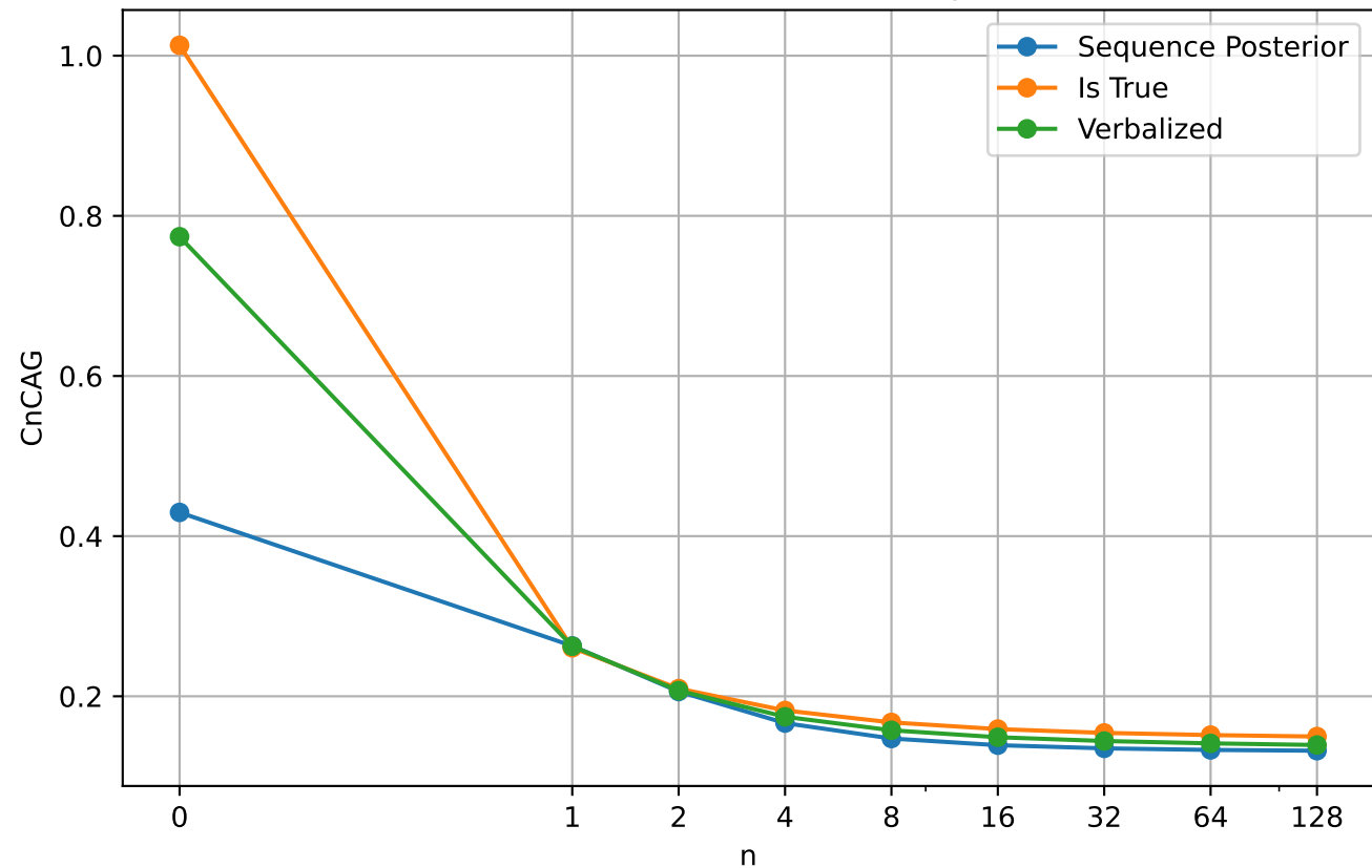
CnCAG vs n for Gemini 2.5 pro
