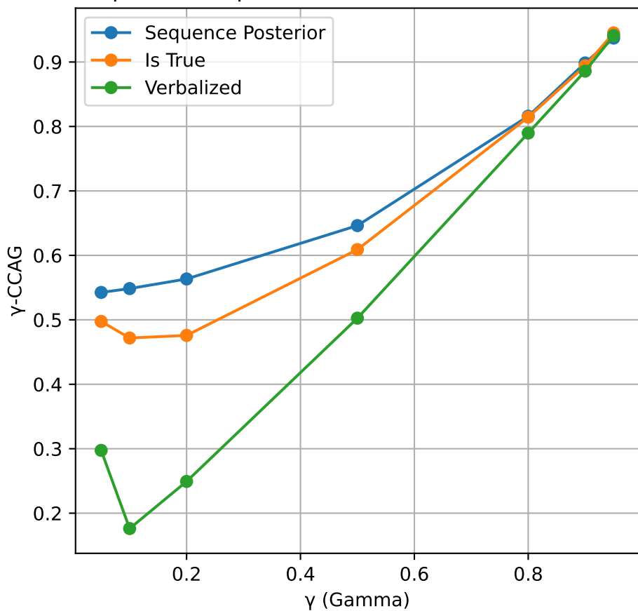
\gamma -CCAG vs \gamma for Ministral-3-8B-Instruct-2512
