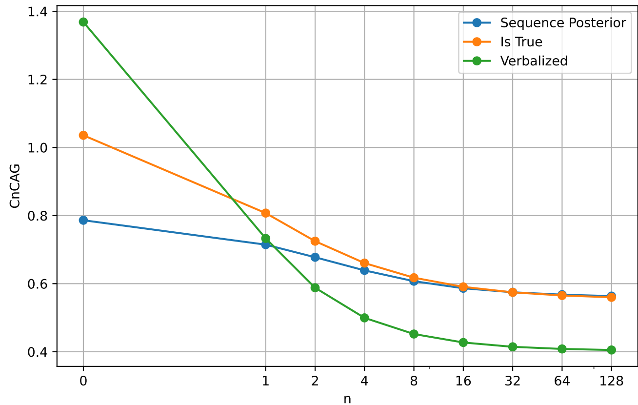
CnCAG vs n for Ministral-3-8B-Instruct-2512
