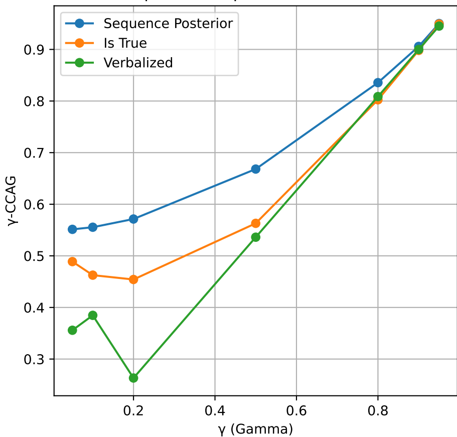
\gamma -CCAG vs \gamma for Qwen3.5 4B
