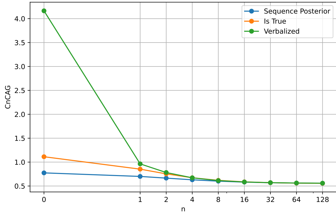
CnCAG vs n for Qwen3.5 4B
