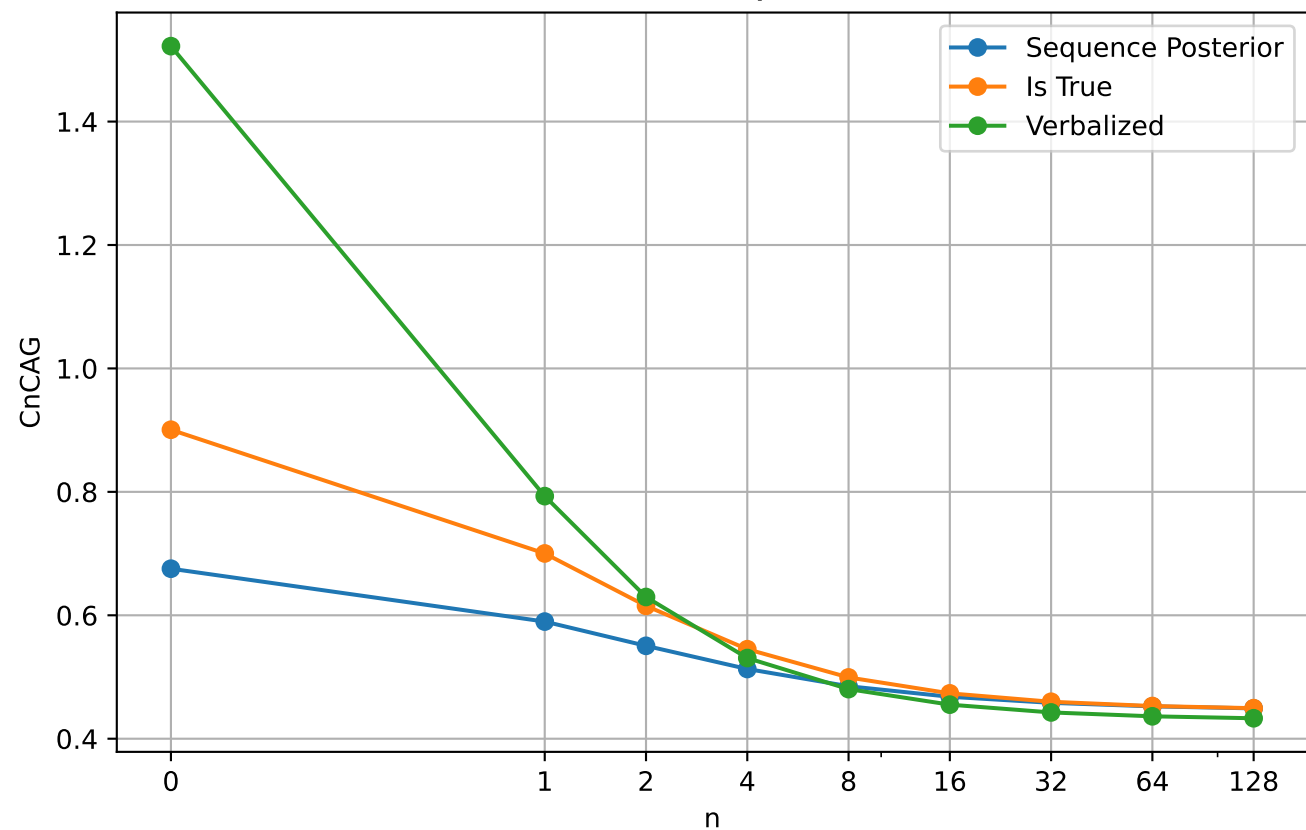
CnCAG vs n for Qwen3.5 9B
