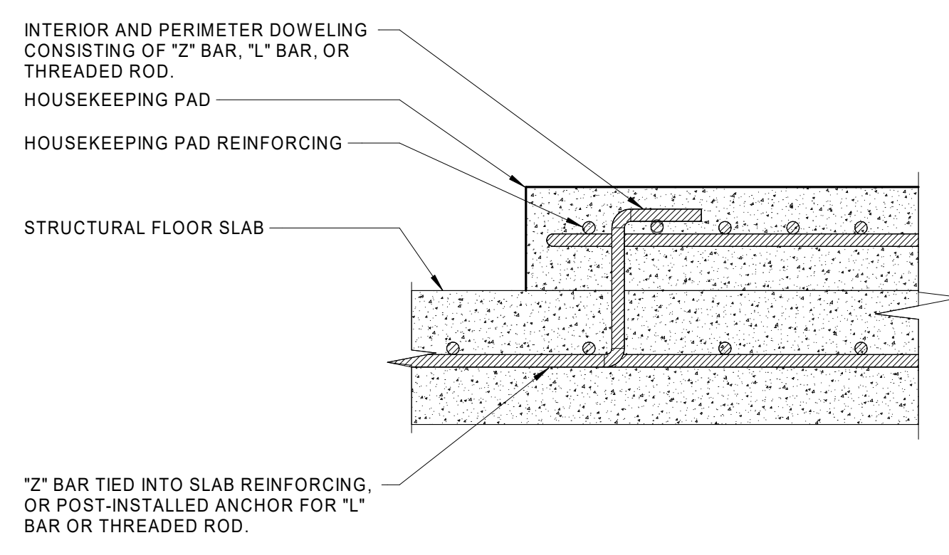
3 SEISMIC SUPPORT - HOUSEKEEPING PAD NO SCALE NOTES: 1. GENERAL REQUIREMENTS FOR SEISMIC HOUSEKEEPING PADS ARE SHOWN. SPECIFIC REQUIREMENTS, INCLUDING ATTACHMENT TO BUILDING STRUCTURE, SHALL BE DETERMINED BY THE SEISMIC RESTRAINT DESIGNER. REFER TO SPECIFICATIONS FOR ADDITIONAL REQUIREMENTS.
