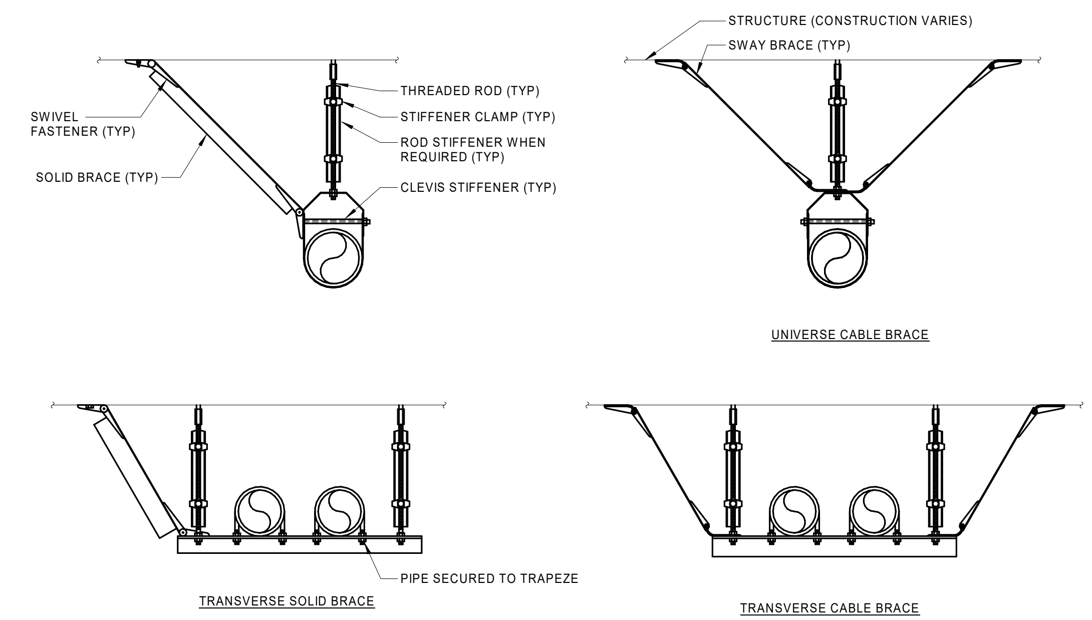
4 SEISMIC SUPPORT - PIPING BRACING NO SCALE NOTES: 1. GENERAL REQUIREMENTS FOR TRANSVERSE AND LONGITUDINAL BRACING OF PIPES ARE SHOWN. SPECIFIC REQUIREMENTS, INCLUDING ATTACHMENT TO BUILDING STRUCTURE, SHALL BE DETERMINED BY THE SEISMIC RESTRAINT DESIGNER. REFER TO SPECIFICATION FOR REQUIREMENTS. 2. REFER TO GENERAL PIPE SUPPORT DETAIL AND SPECIFICATION FOR INSULATED PIPING CONSIDERATIONS.
