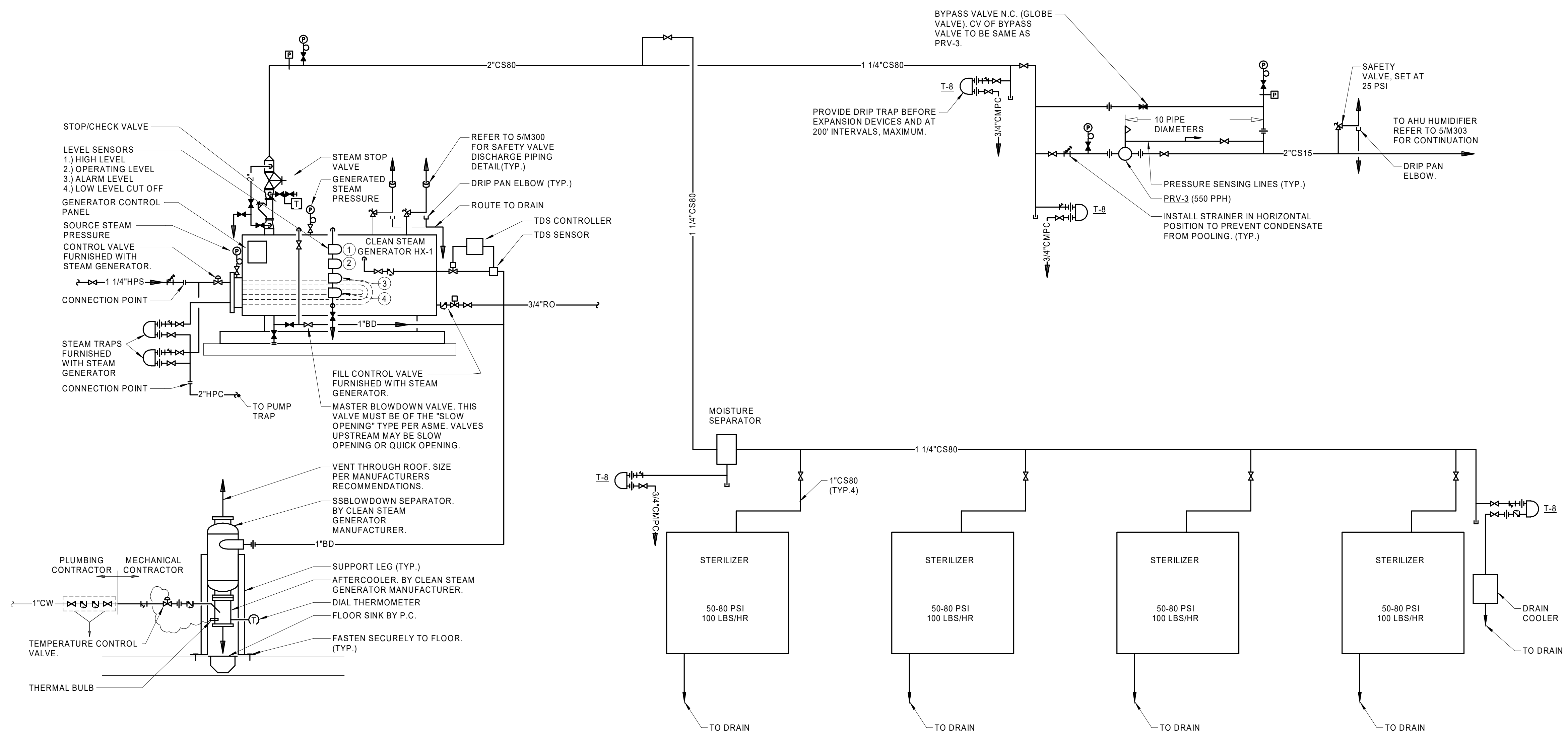
1 CLEAN STEAM FLOW DIAGRAM NO SCALE NOTES: 1. MAKE ALL TAPS FROM TOP OF STEAM PIPES.
