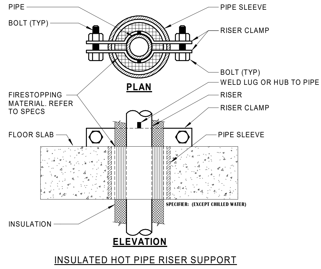
INSULATED HOT PIPE RISER SUPPORT
