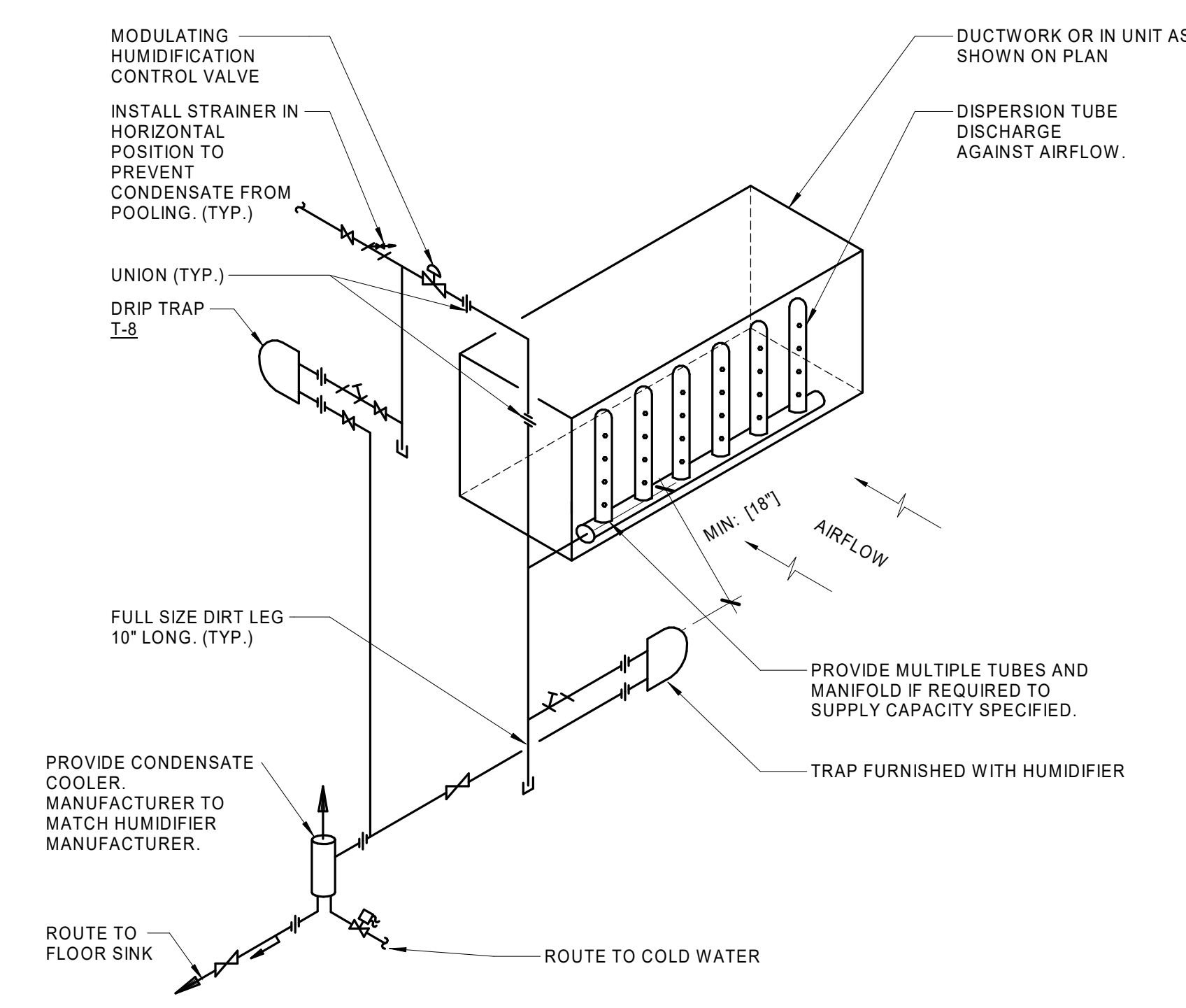
5 HUMIDIFIER PIPING 12" = 1'-0"
