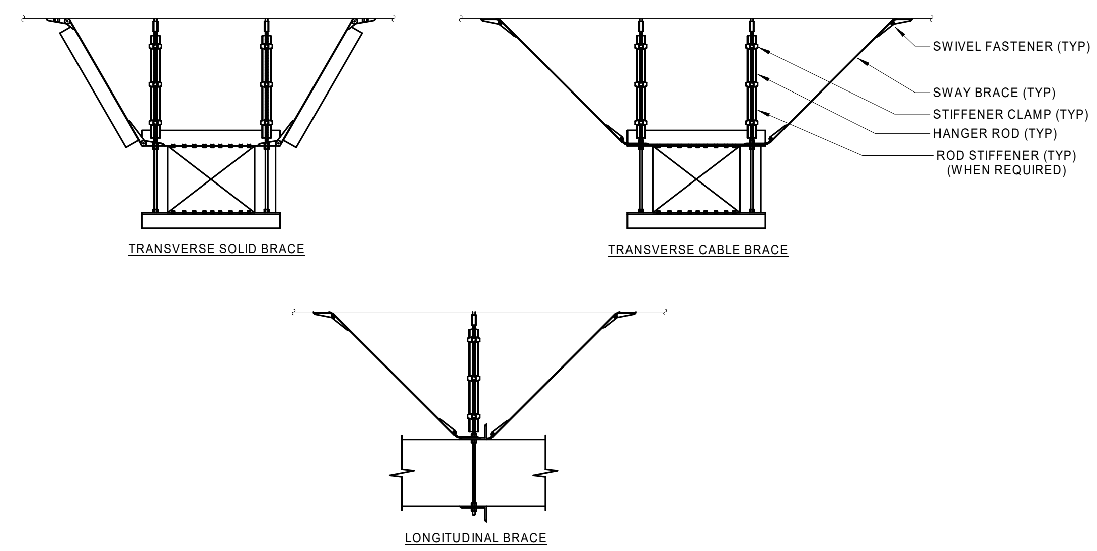
2 SEISMIC SUPPORT - DUCTWORK BRACING NO SCALE NOTES: 1. GENERAL REQUIREMENTS FOR SEISMIC RESTRAINT OF DUCTWORK ARE SHOWN. SPECIFIC REQUIREMENTS, INCLUDING ATTACHMENT TO BUILDING STRUCTURE, SHALL BE DETERMINED BY THE SEISMIC RESTRAINT DESIGNER. REFER TO SPECIFICATION FOR REQUIREMENTS.
