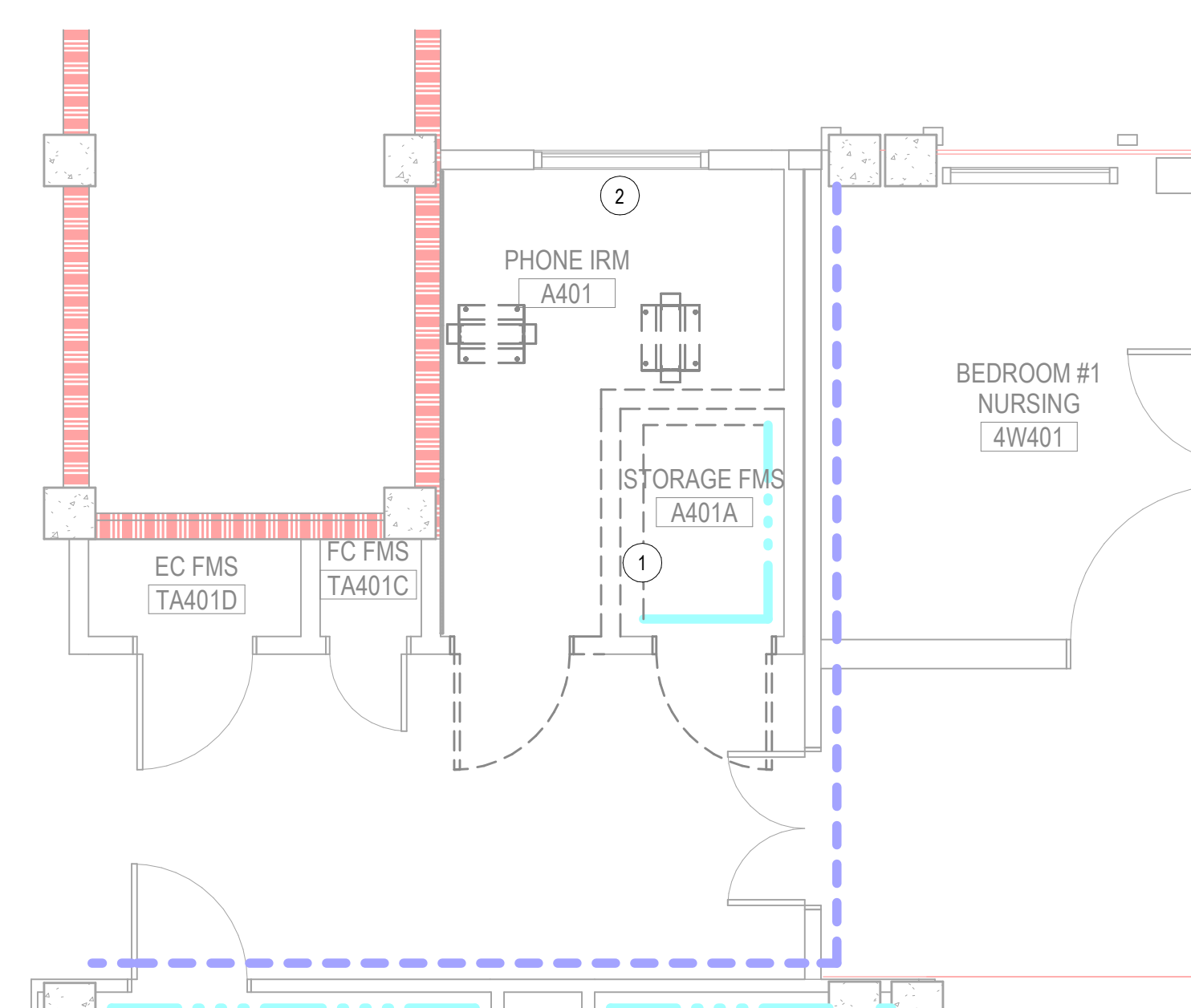
2 A401 - PLUMBING DEMOLITION PLAN 1/4" = 1'-0"
