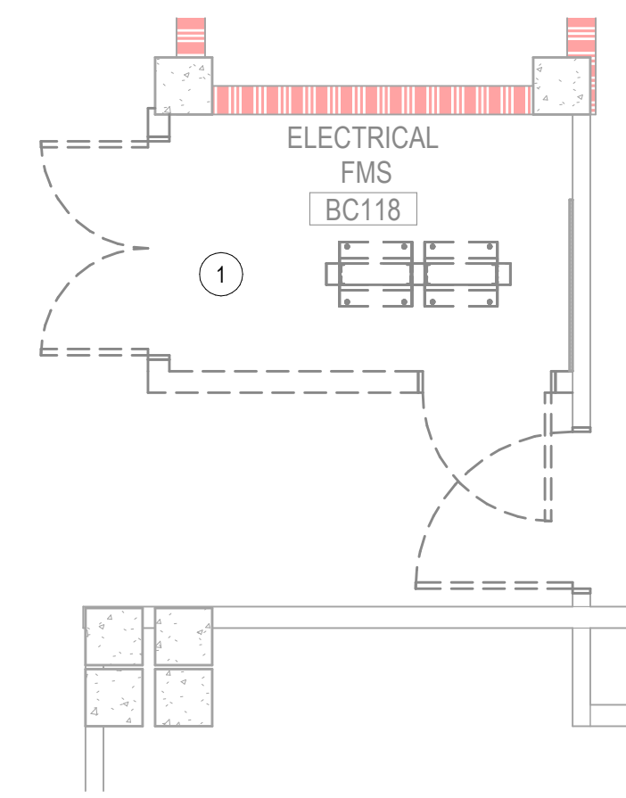
2 BC118 - PLUMBING DEMOLITION PLAN 1/4" = 1'-0"
