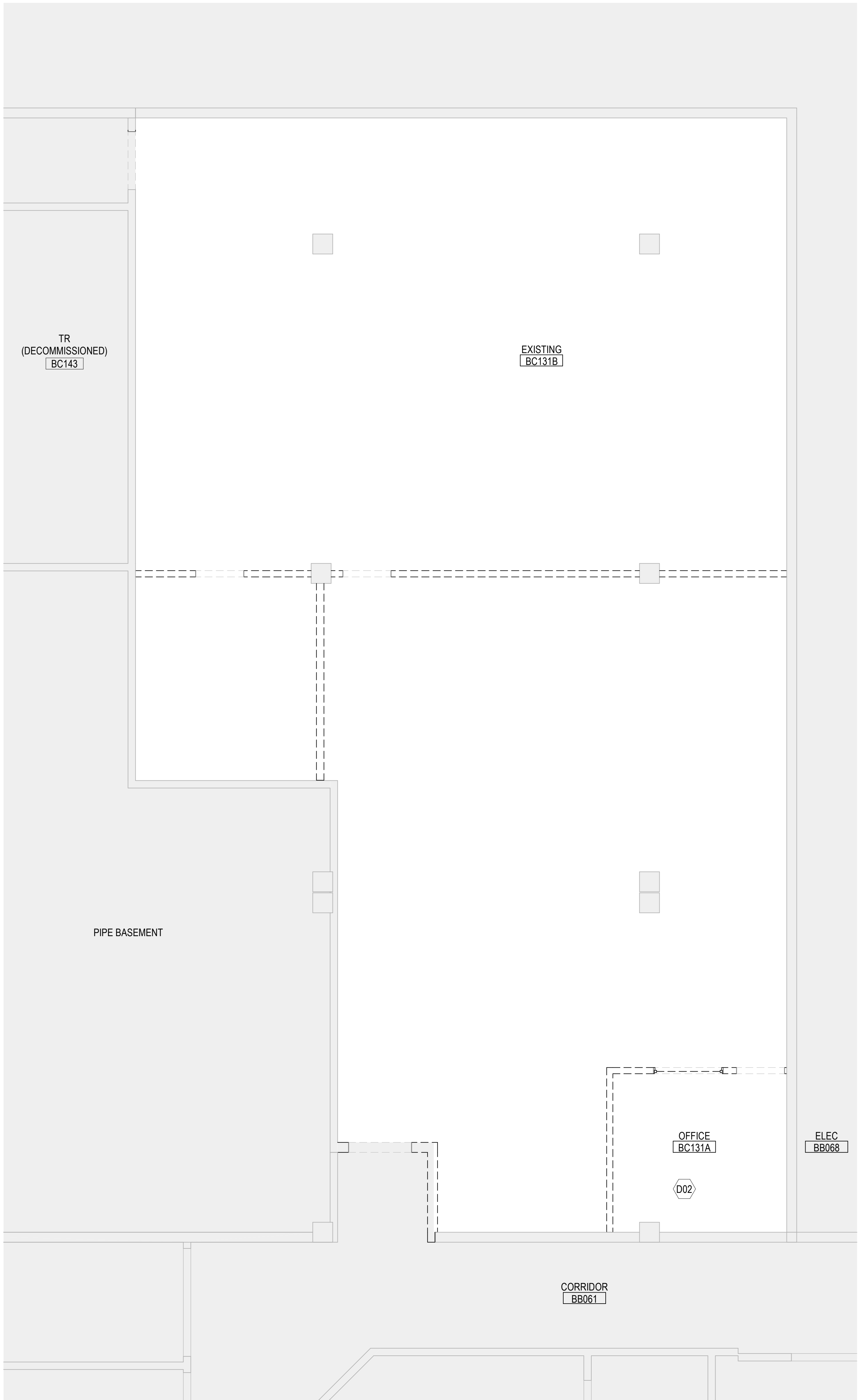
2 ENLARGED DEMO RCP - BASEMENT (BC131B) 1/4" = 1'-0"
