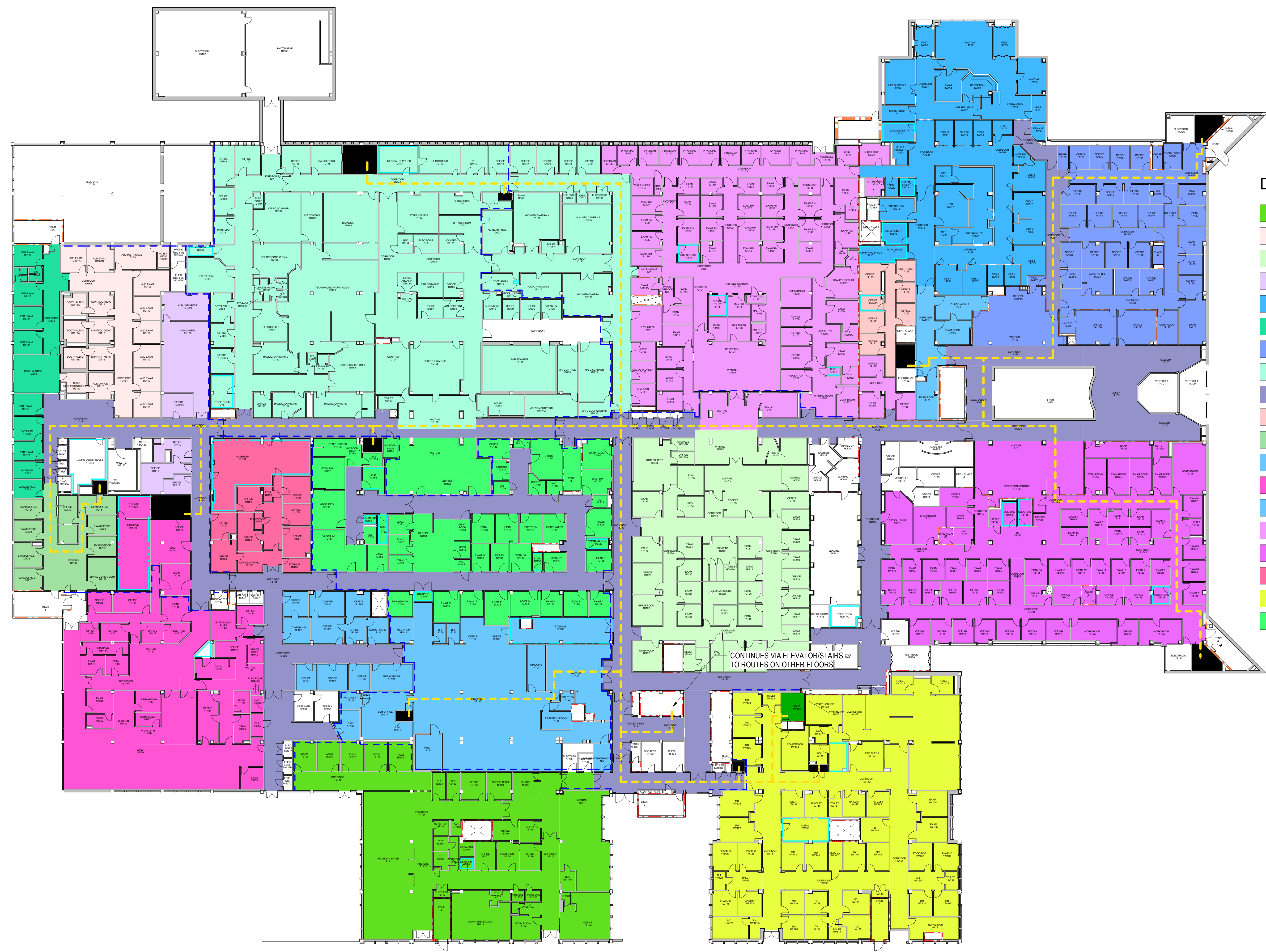
1 1ST FLOOR SEQUENCING PLAN 1" = 20'-0"
