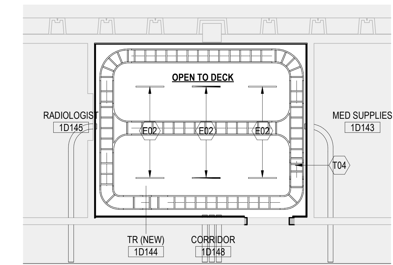
4 ENLARGED RCP - 1ST FLOOR (1D144) 1/4" = 1'-0"
