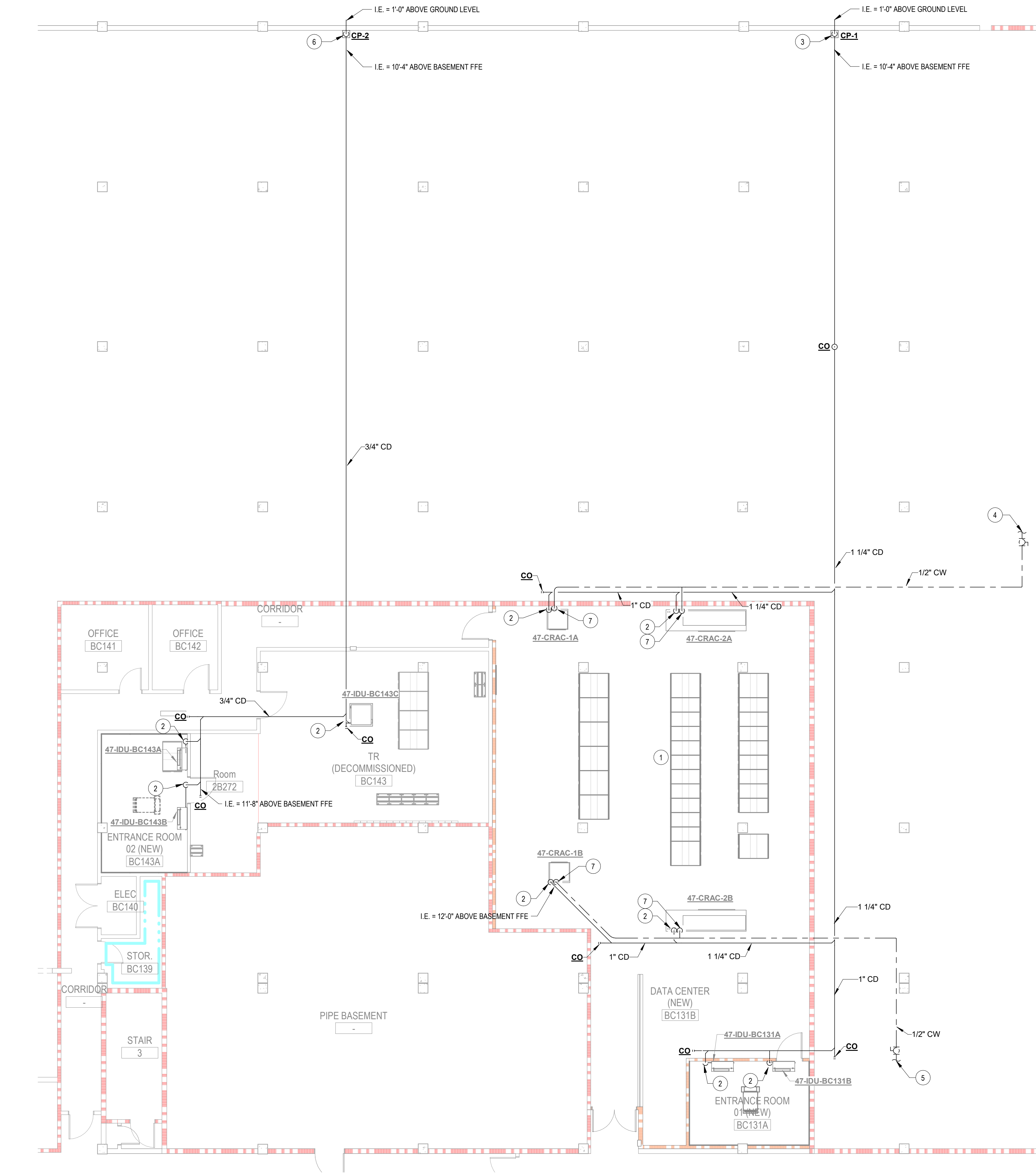
1 DATA CENTER - PLUMBING PLAN 1/8" = 1'-0"
