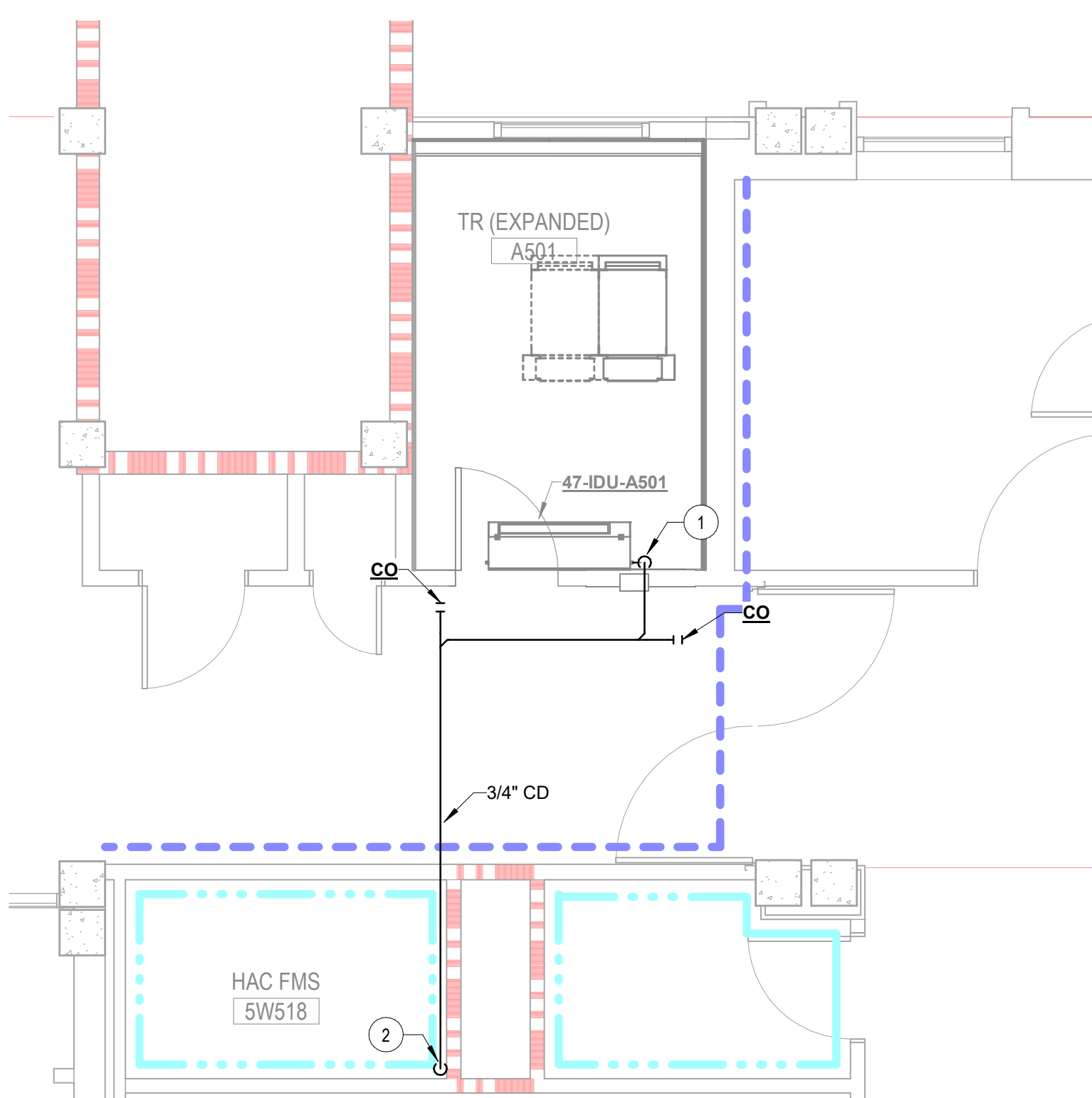
3 A501 - PLUMBING PLAN 1/4" = 1'-0"
