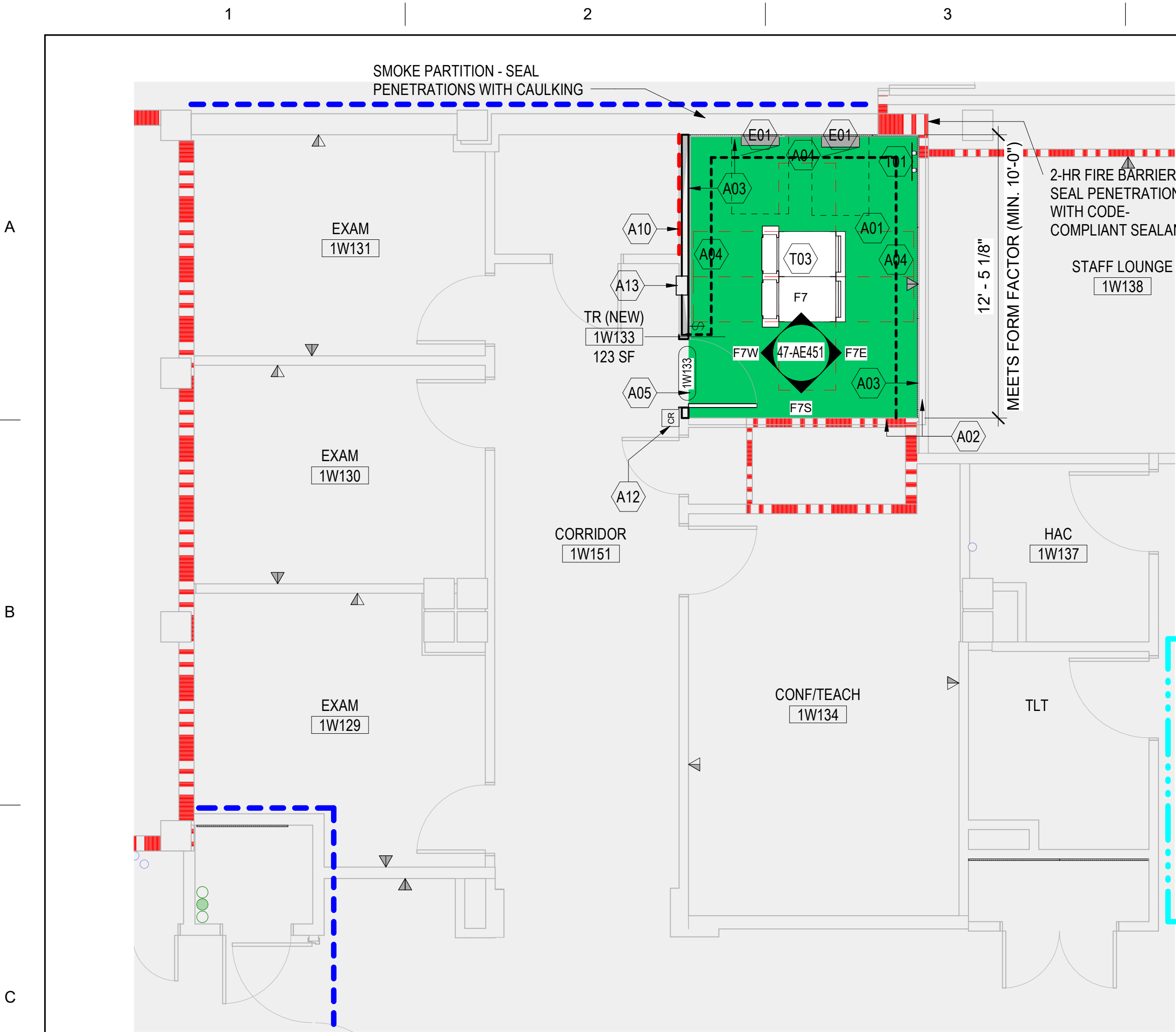
1 ENLARGED FLOOR PLAN - 1ST FLOOR (1W133) 1/4" = 1'-0"
