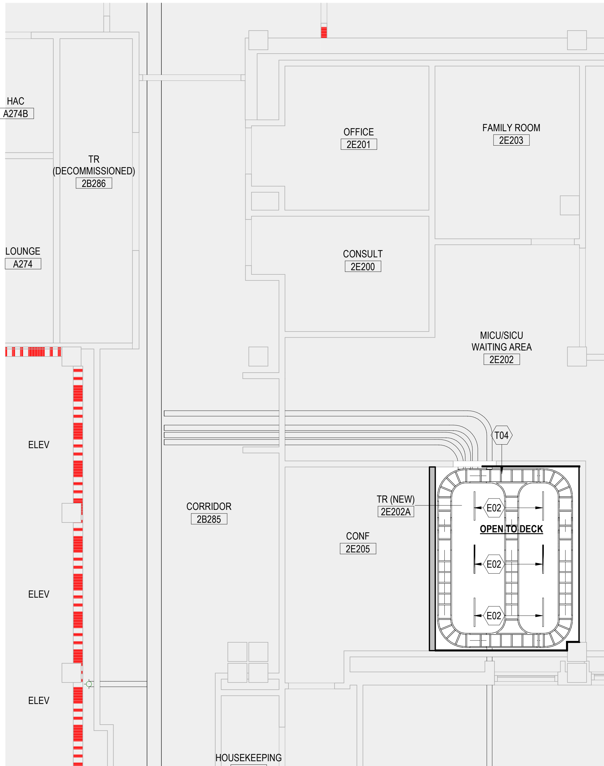
2 ENLARGED RCP - 2ND FLOOR (2E202A)
