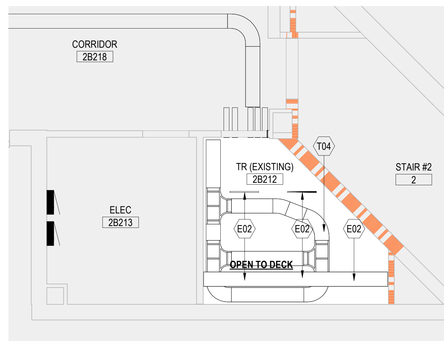
6 ENLARGED RCP - 2ND FLOOR (2B212)
