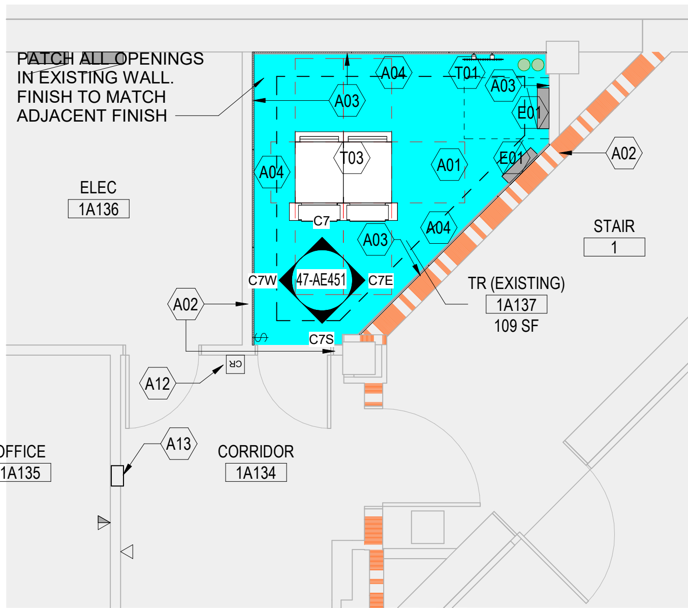
5 ENLARGED FLOOR PLAN - 1ST FLOOR (1A137) 1/4" = 1'-0"
