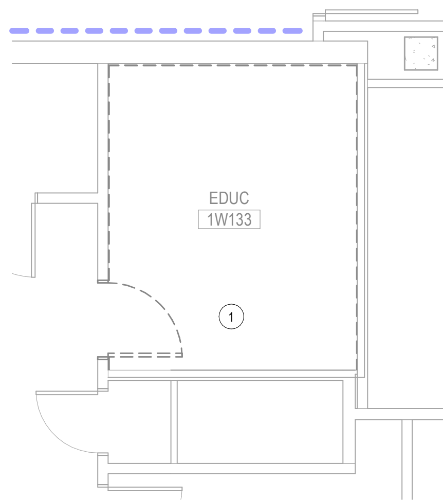
3 1W133 - PLUMBING DEMOLITION PLAN 1/4" = 1'-0"
