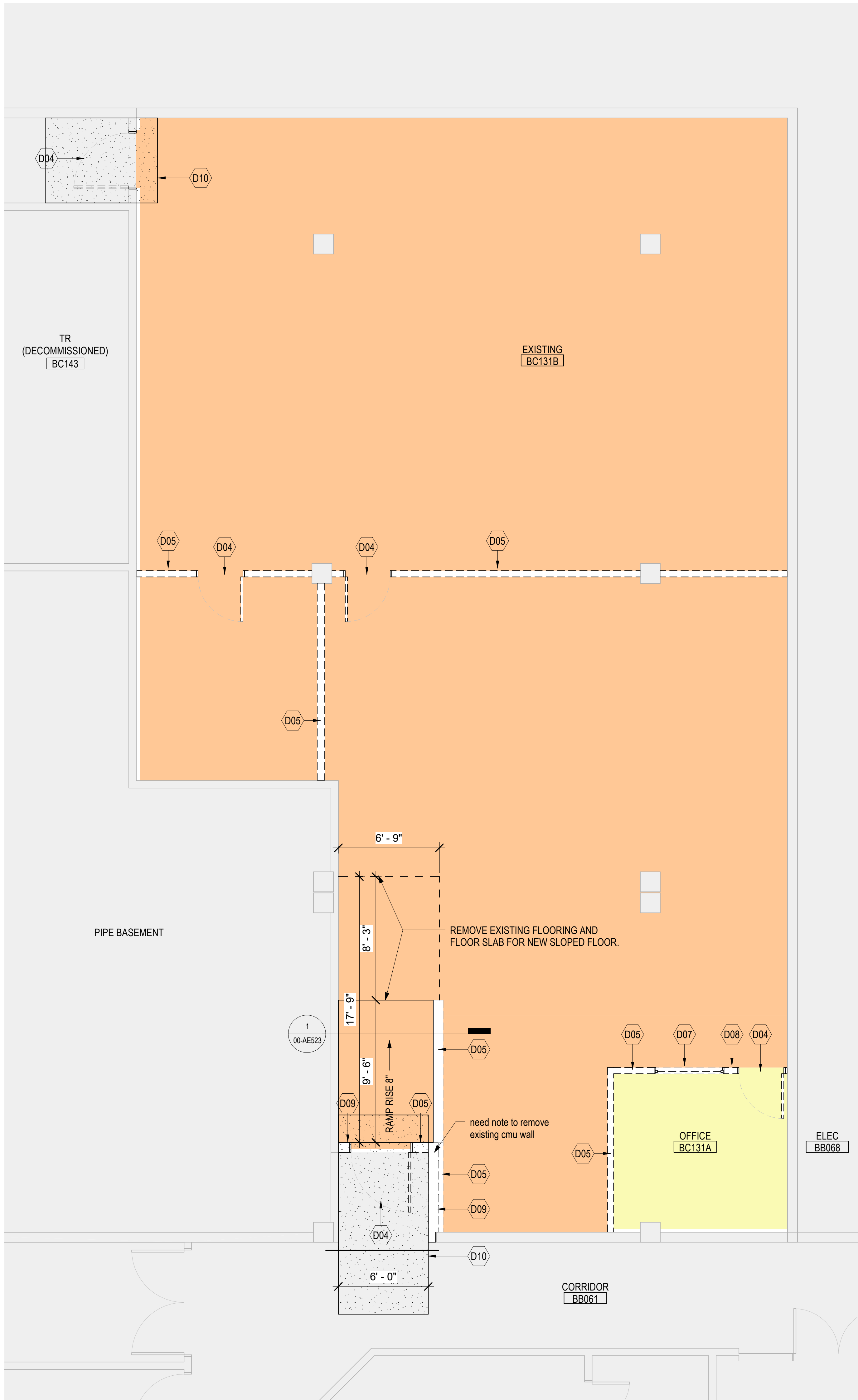
1 ENLARGED DEMO PLAN - BASEMENT (BC131B) 1/4" = 1'-0"
