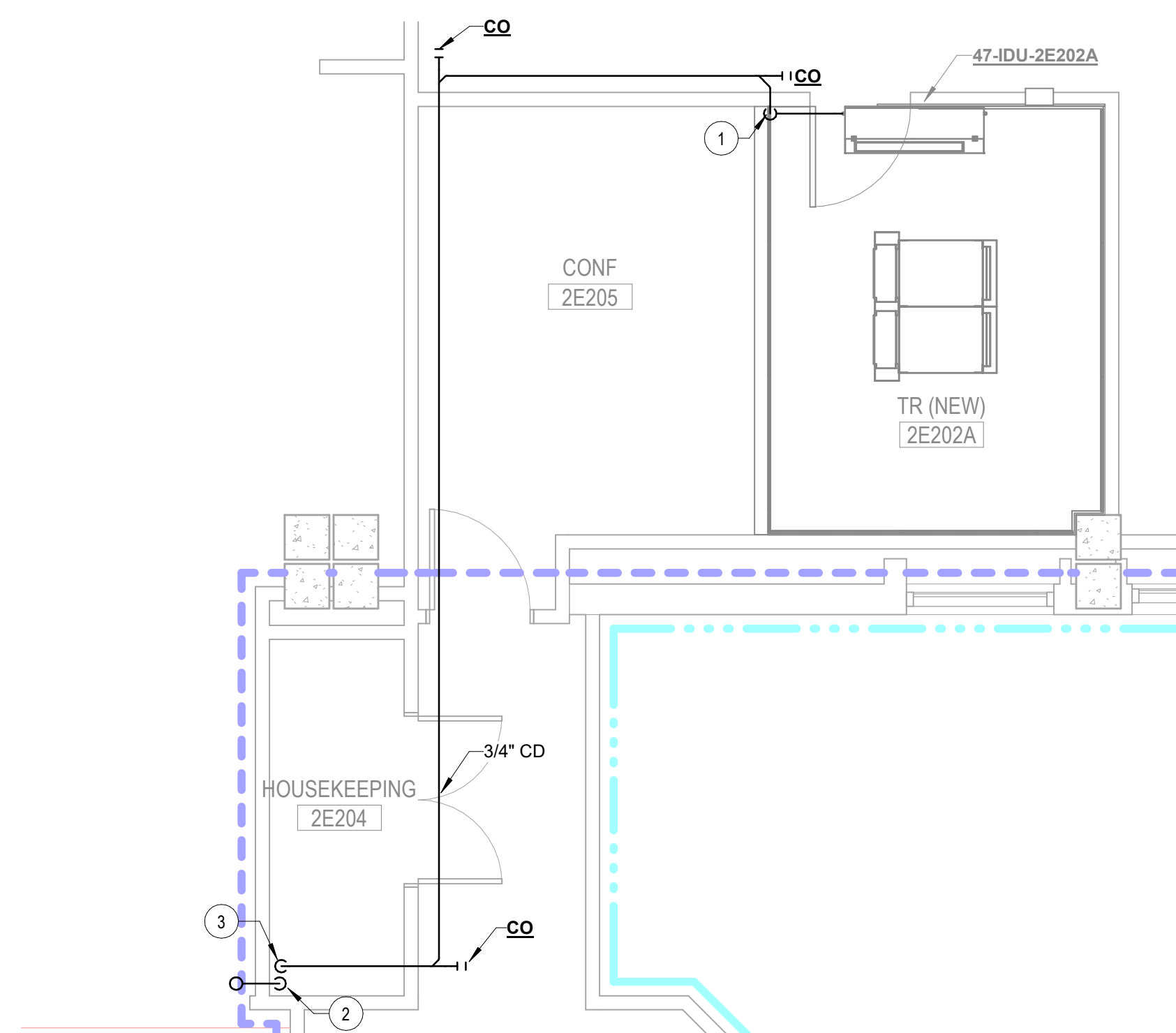
3 2E202A - PLUMBING PLAN 1/4" = 1'-0"
