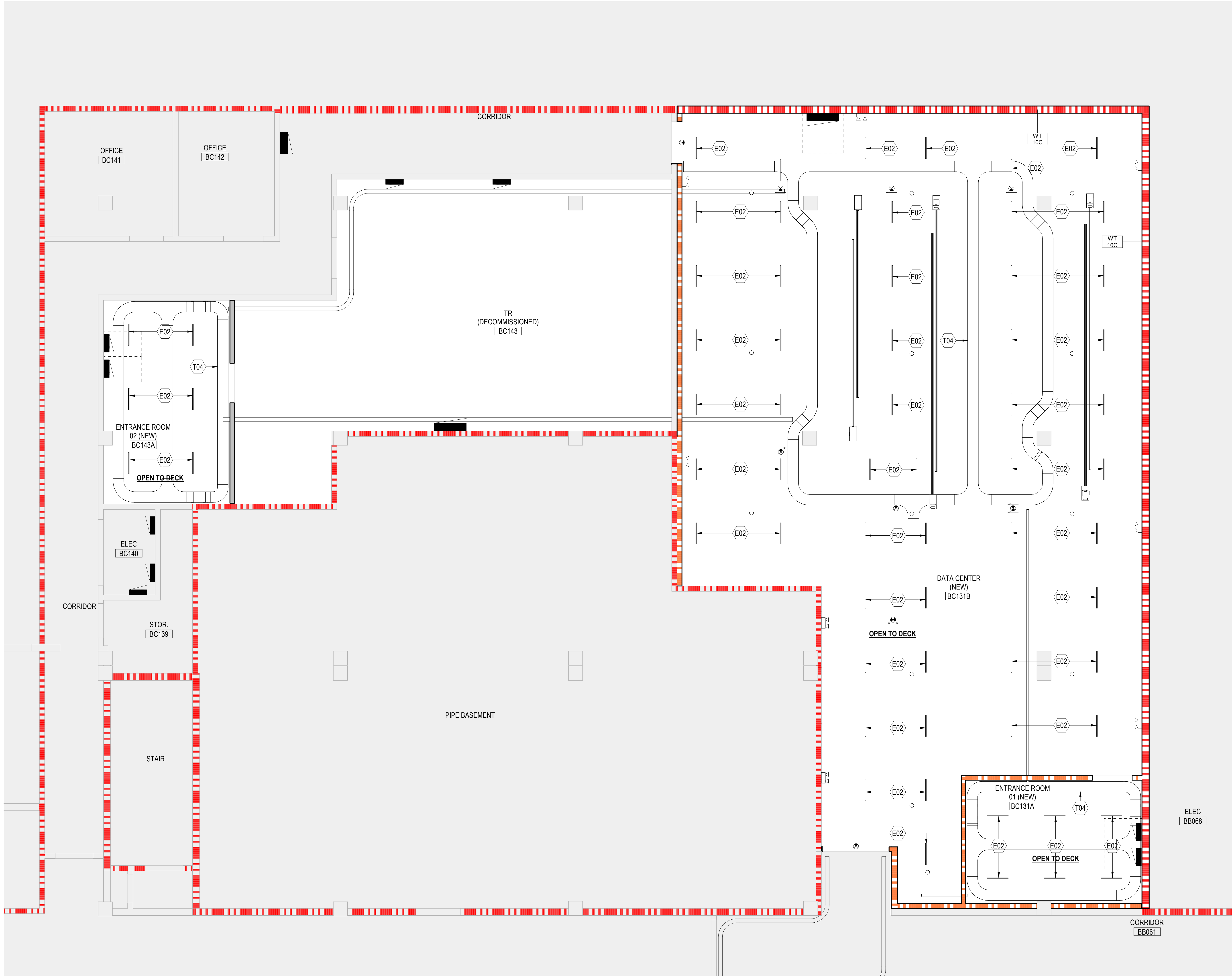
1 ENLARGED RCP - BASEMENT (BC131) 1/4" = 1'-0"
