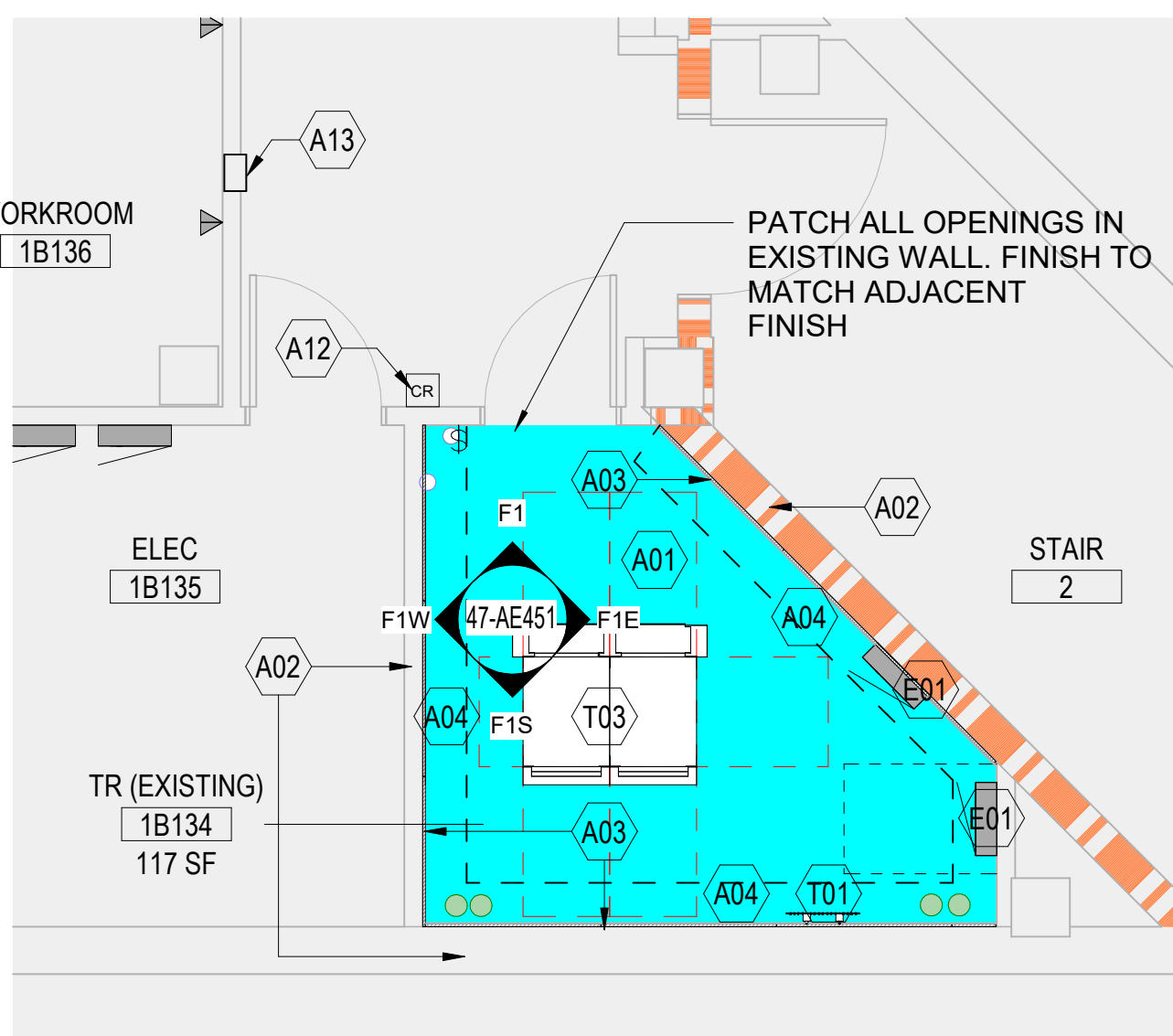
7 ENLARGED FLOOR PLAN - 1ST FLOOR (1B134) 1/4" = 1'-0"
