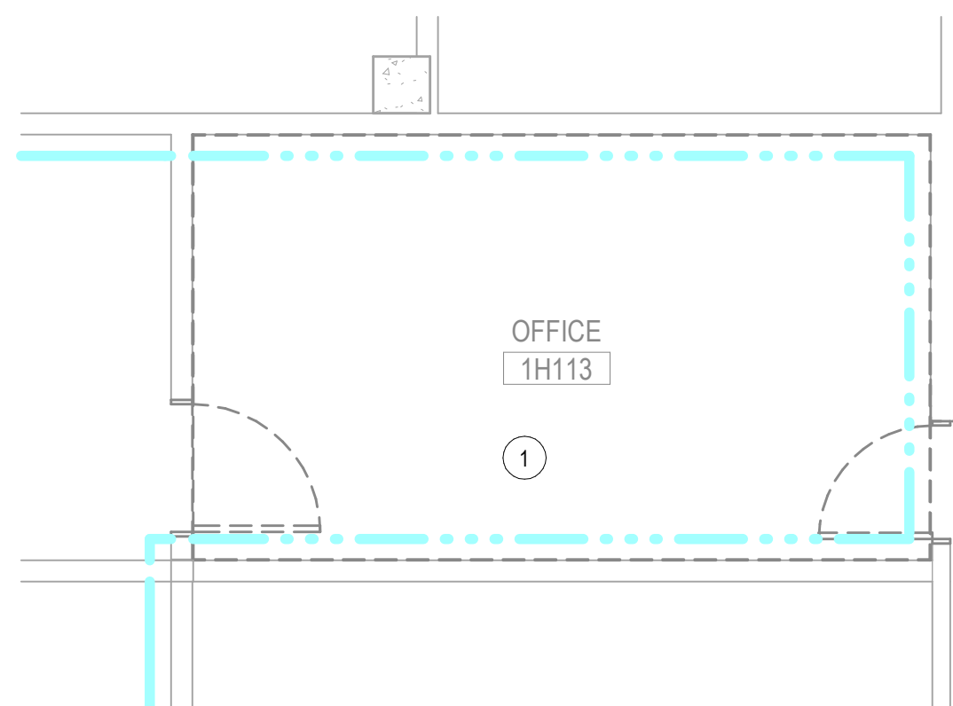
5 1H113 - PLUMBING DEMOLITION PLAN 1/4" = 1'-0"
