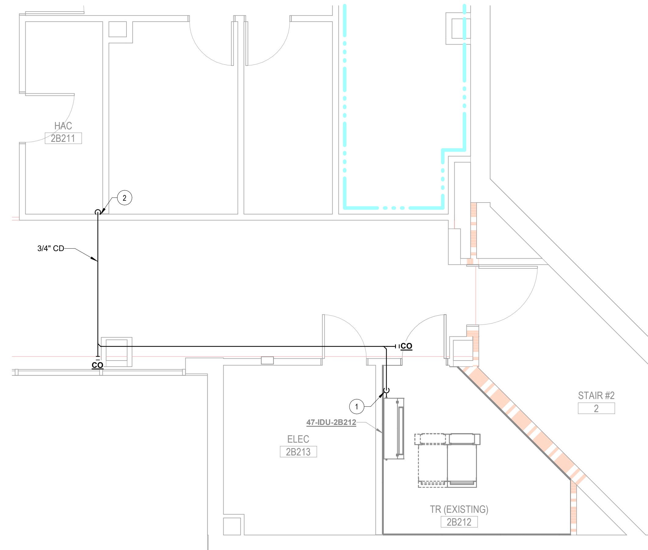
2 2B212 - PLUMBING PLAN 1/4" = 1'-0"
