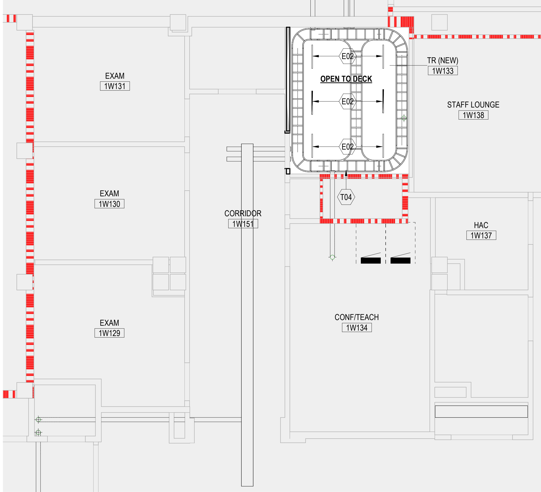
2 ENLARGED RCP - 1ST FLOOR (1W133) 1/4" = 1'-0"
