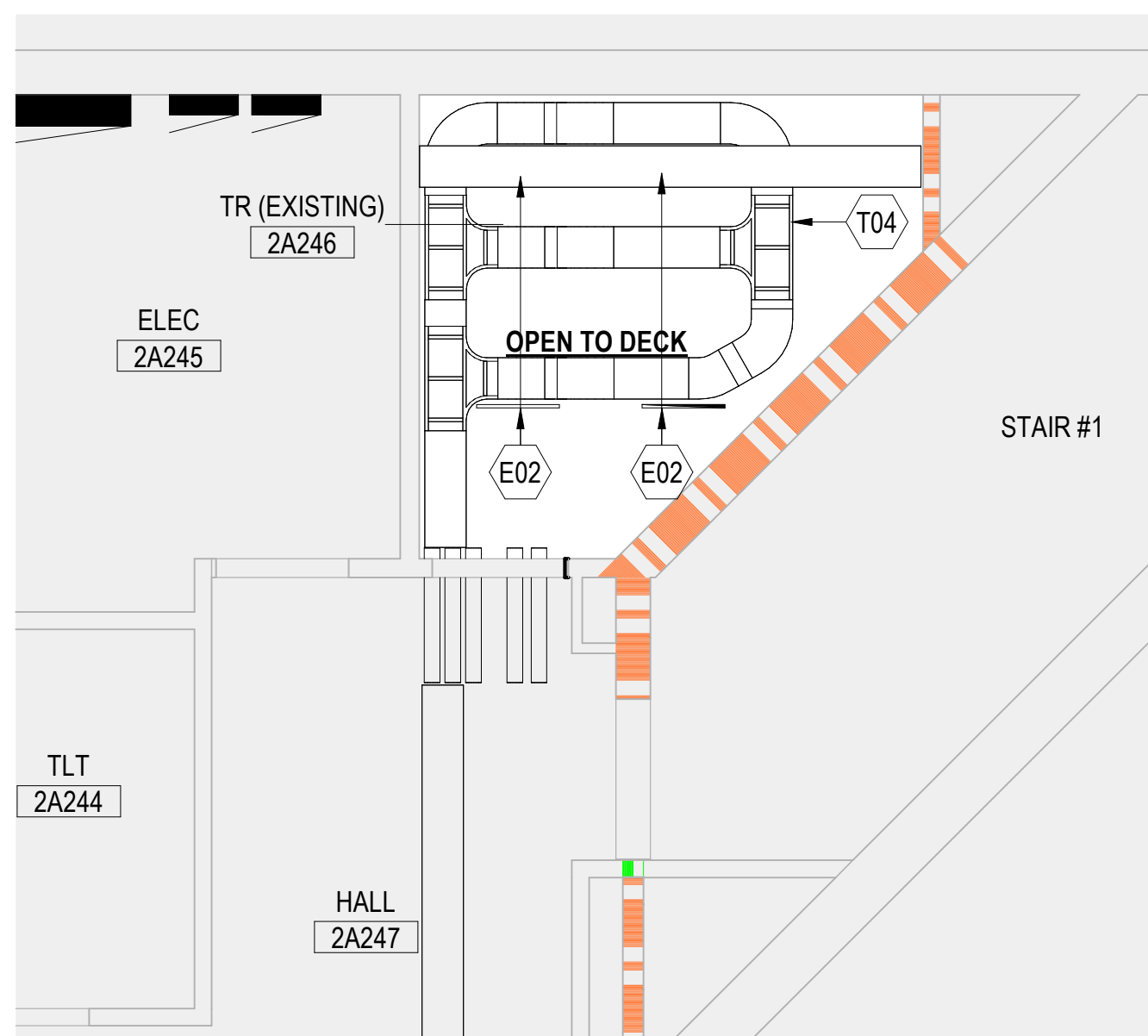
4 ENLARGED RCP - 2ND FLOOR (2A246)
