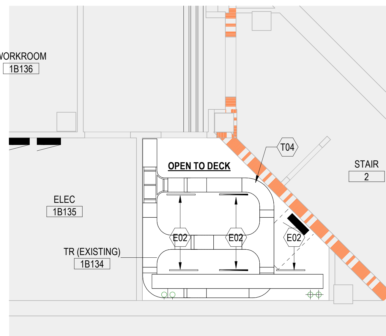
8 ENLARGED RCP - 1ST FLOOR (1B134) 1/4" = 1'-0"
