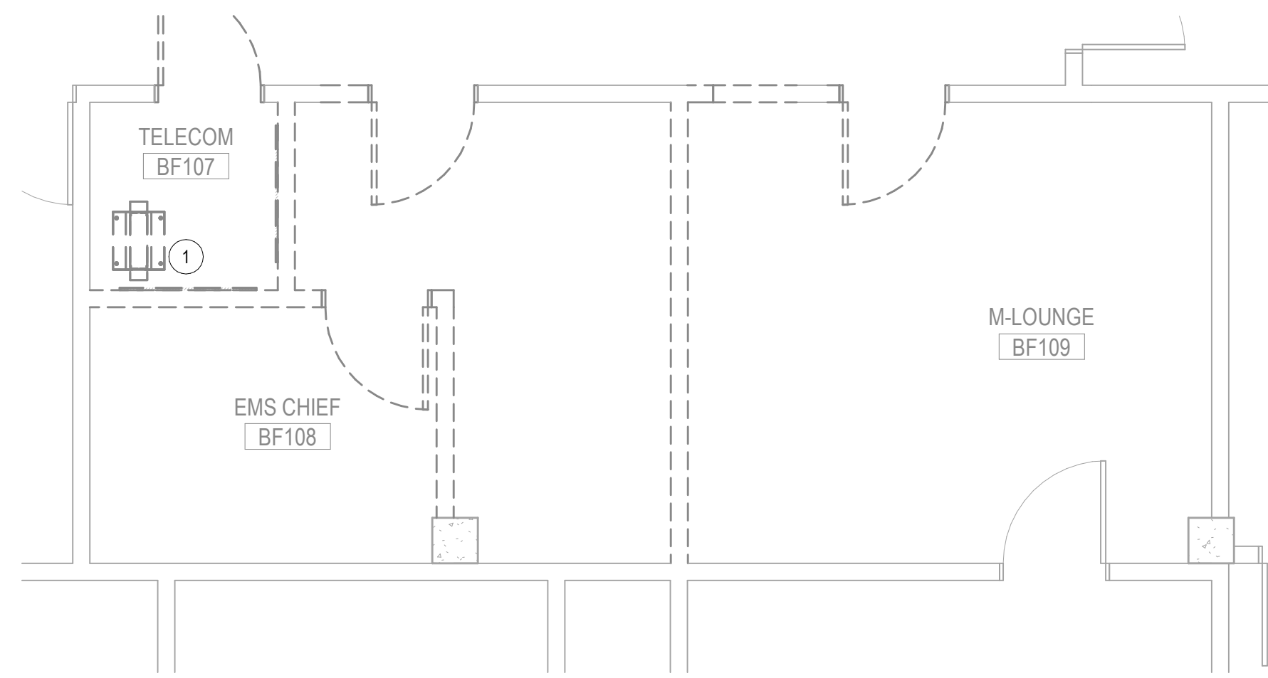
1 BF107 - PLUMBING DEMOLITION PLAN 1/4" = 1'-0"
