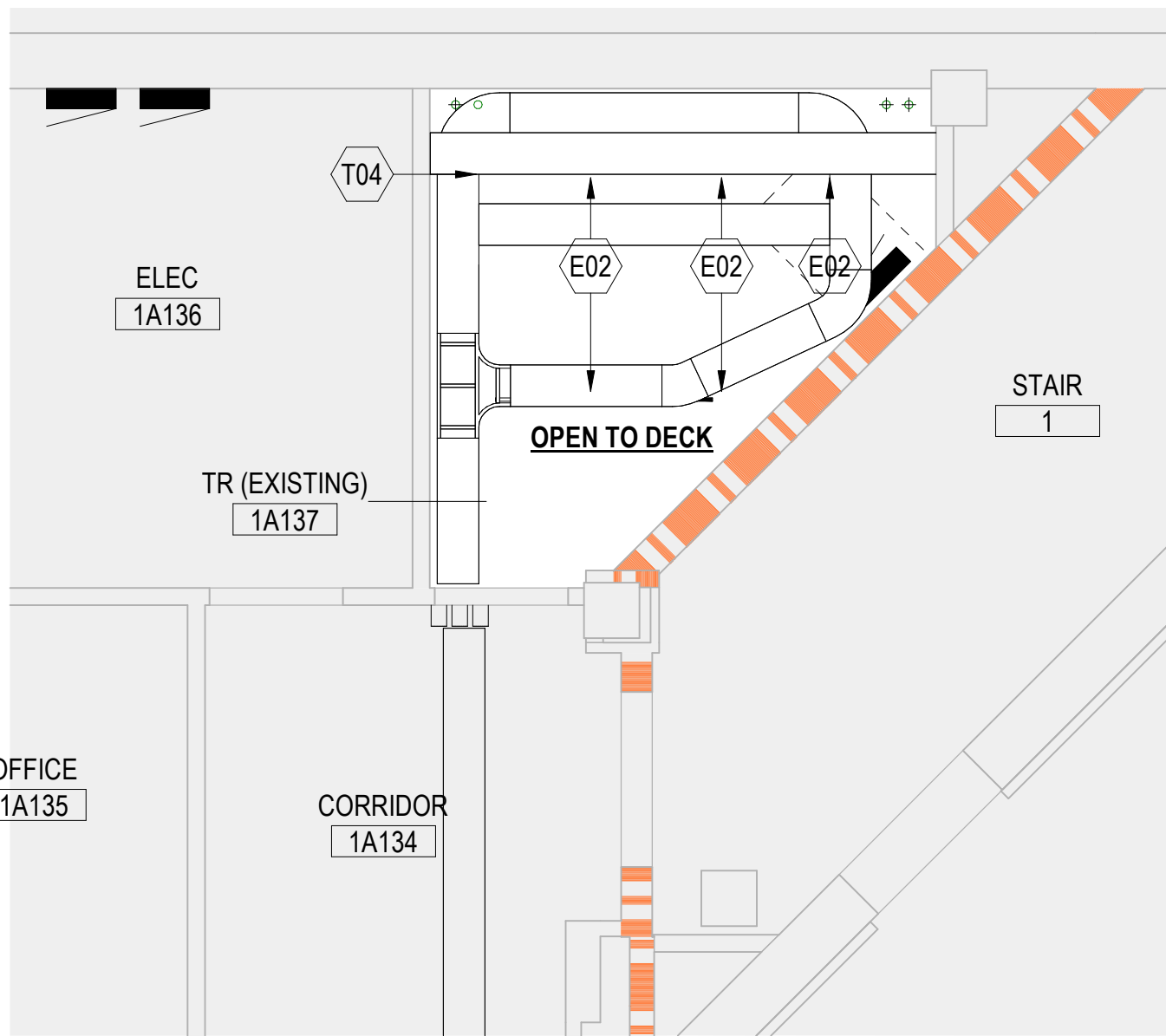
6 ENLARGED RCP - 1ST FLOOR (1A137) 1/4" = 1'-0"
