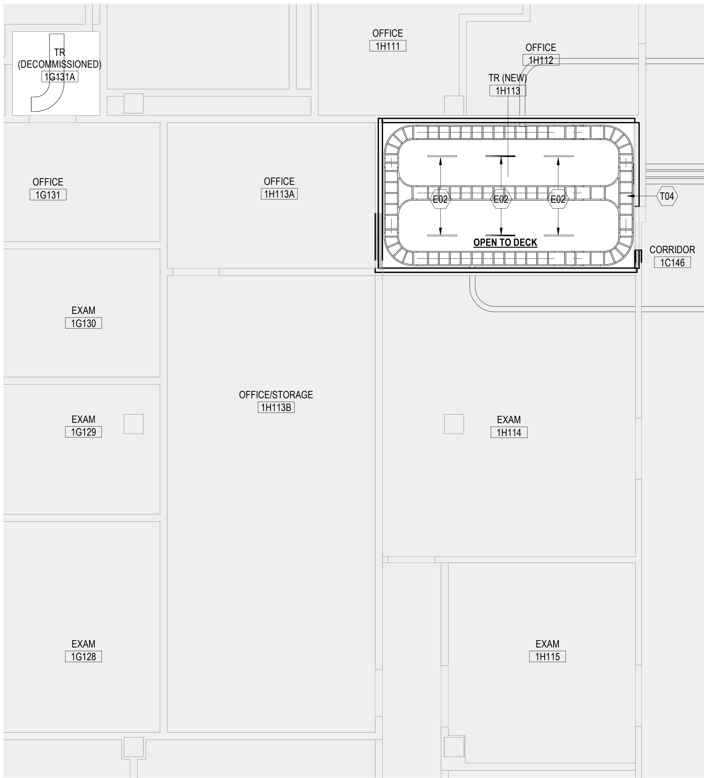
2 ENLARGED RCP - 1ST FLOOR (1H113) 1/4" = 1'-0"
