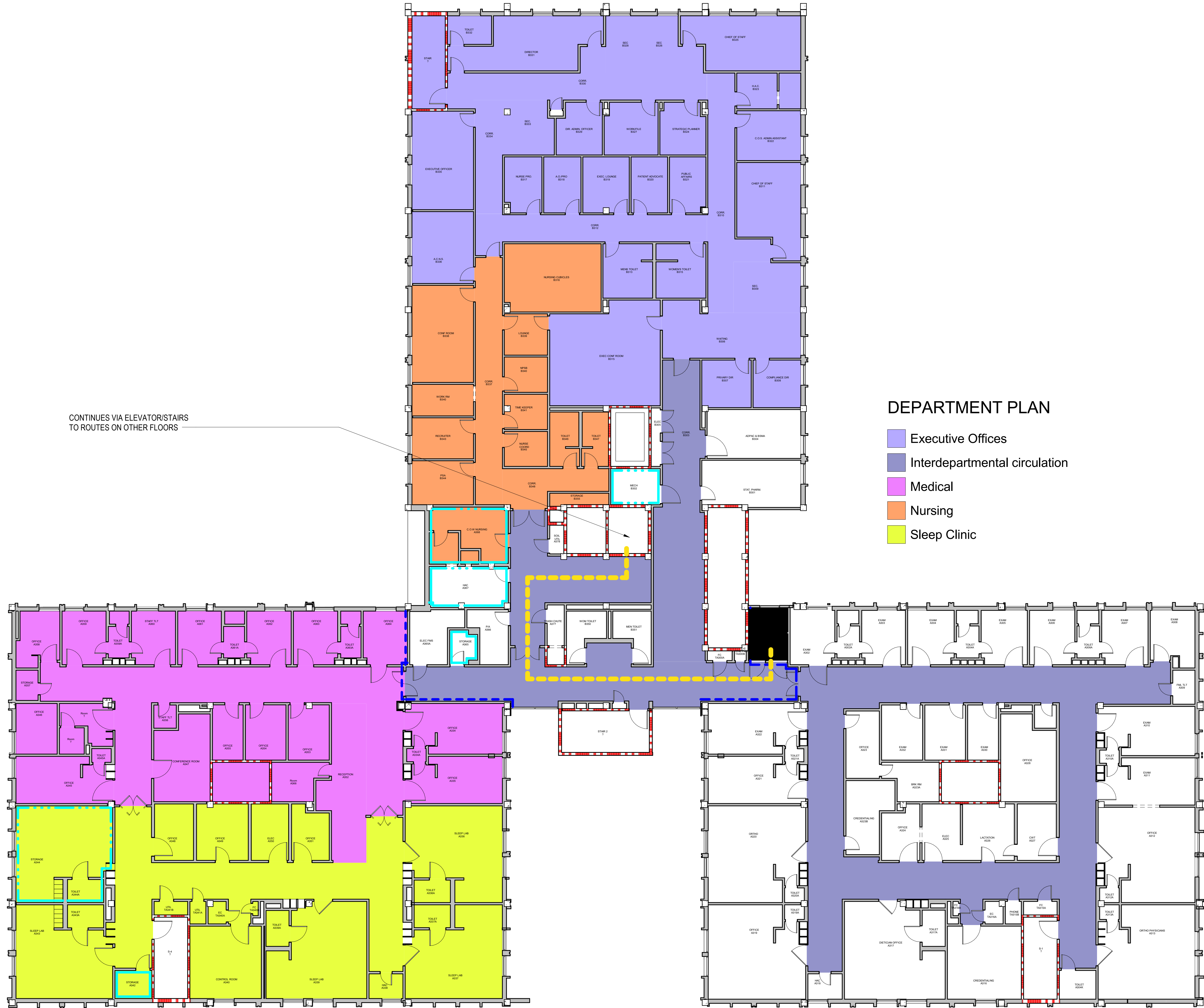
1 THIRD FLOOR PLAN - AREA B 3/32" = 1'-0"
