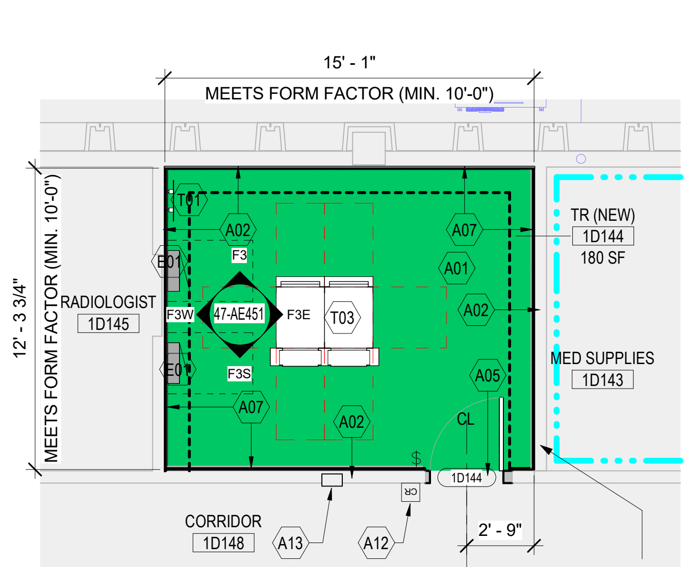
3 ENLARGED FLOOR PLAN - 1ST FLOOR (1D144) 1/4" = 1'-0"
