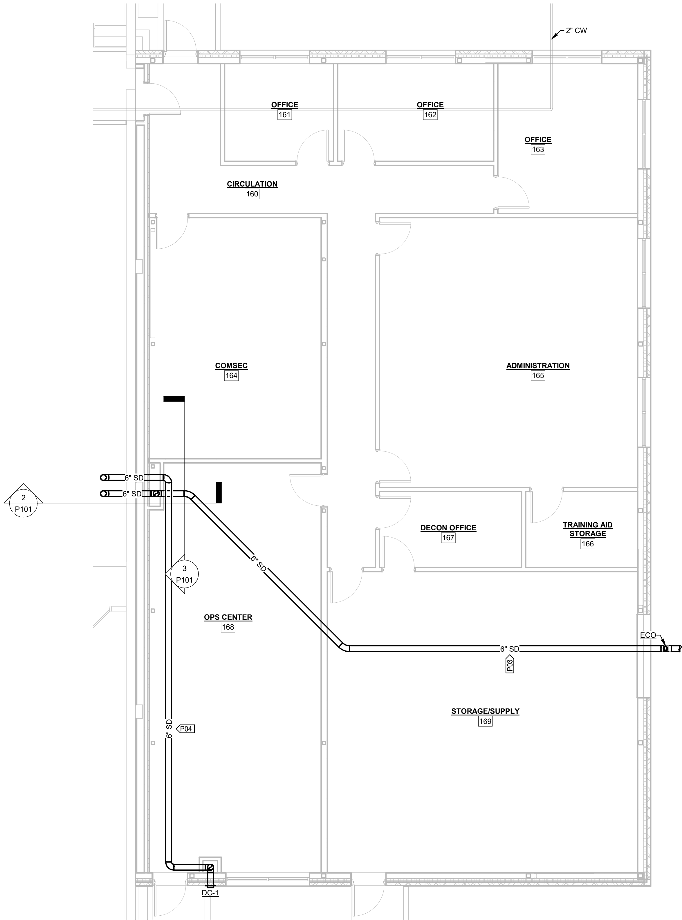
1 PLUMBING PLAN - NEW ADDITION 3/16" = 1'-0"
