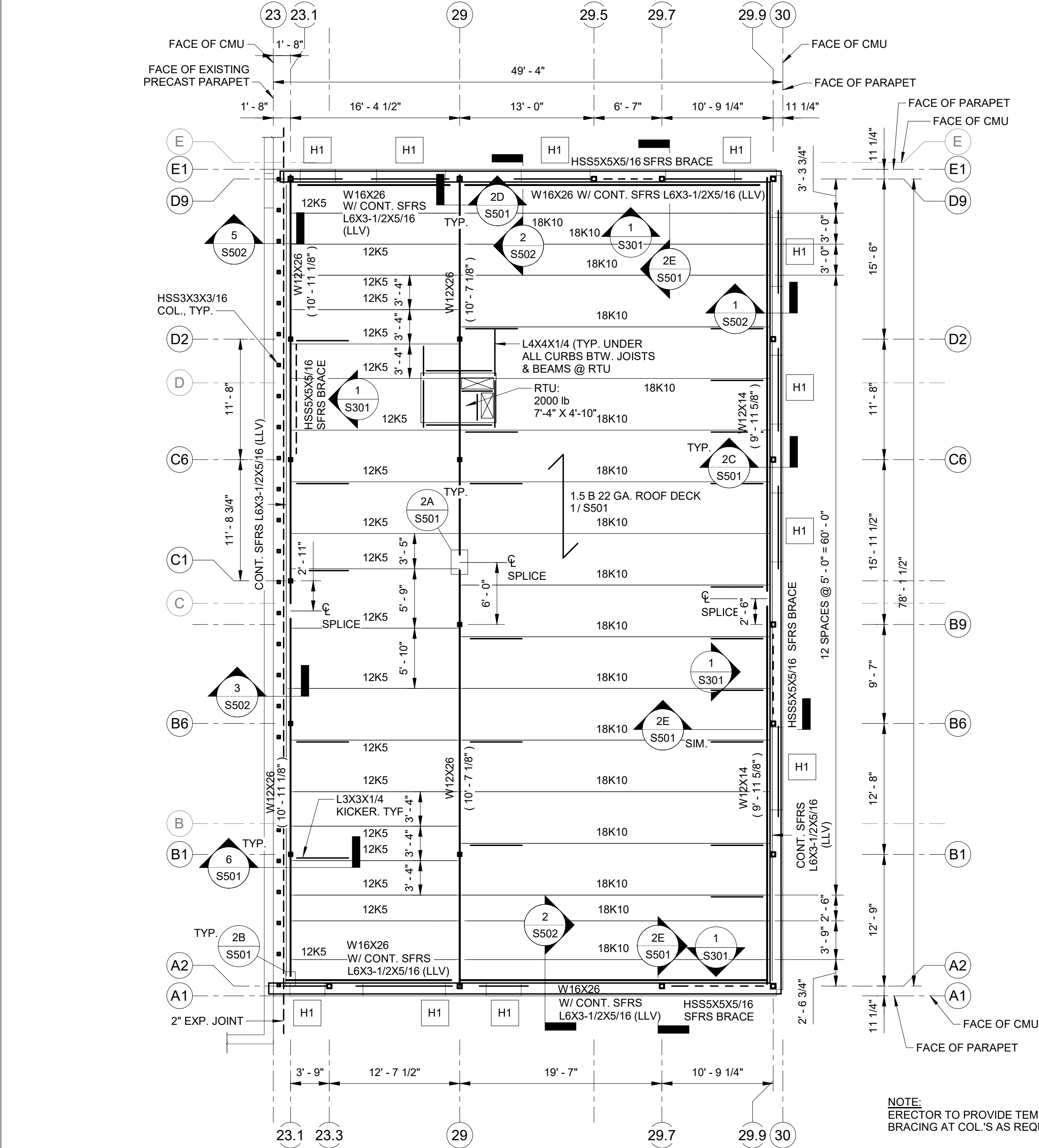
1 ROOF FRAMING PLAN 1/8" = 1'-0"
