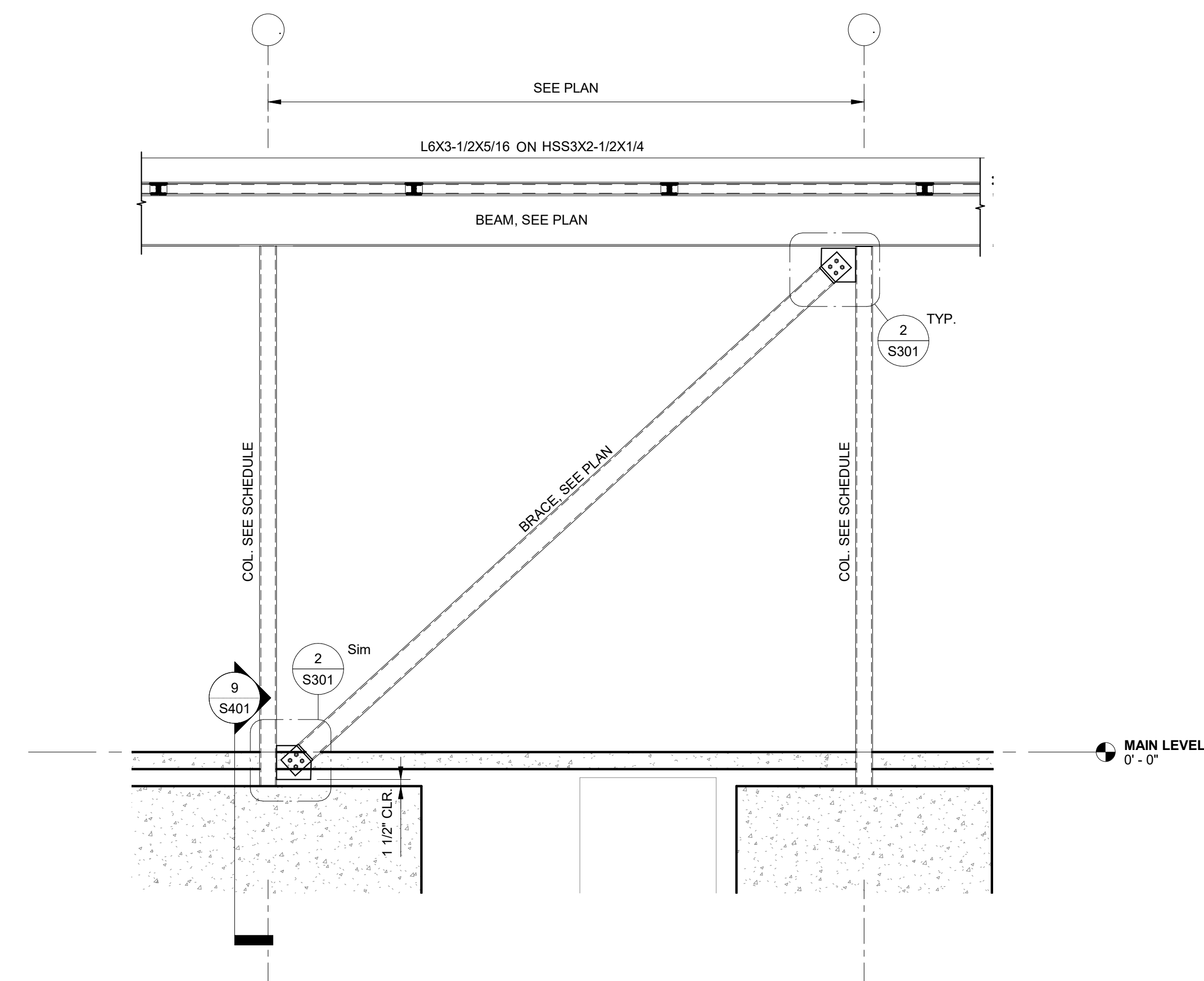
1 SFRS HSS BRACE 1/2" = 1'-0"
