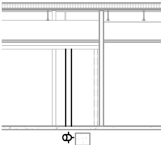
3 OPS CENTER 168 WEST SECTION 3/16" = 1'-0"
