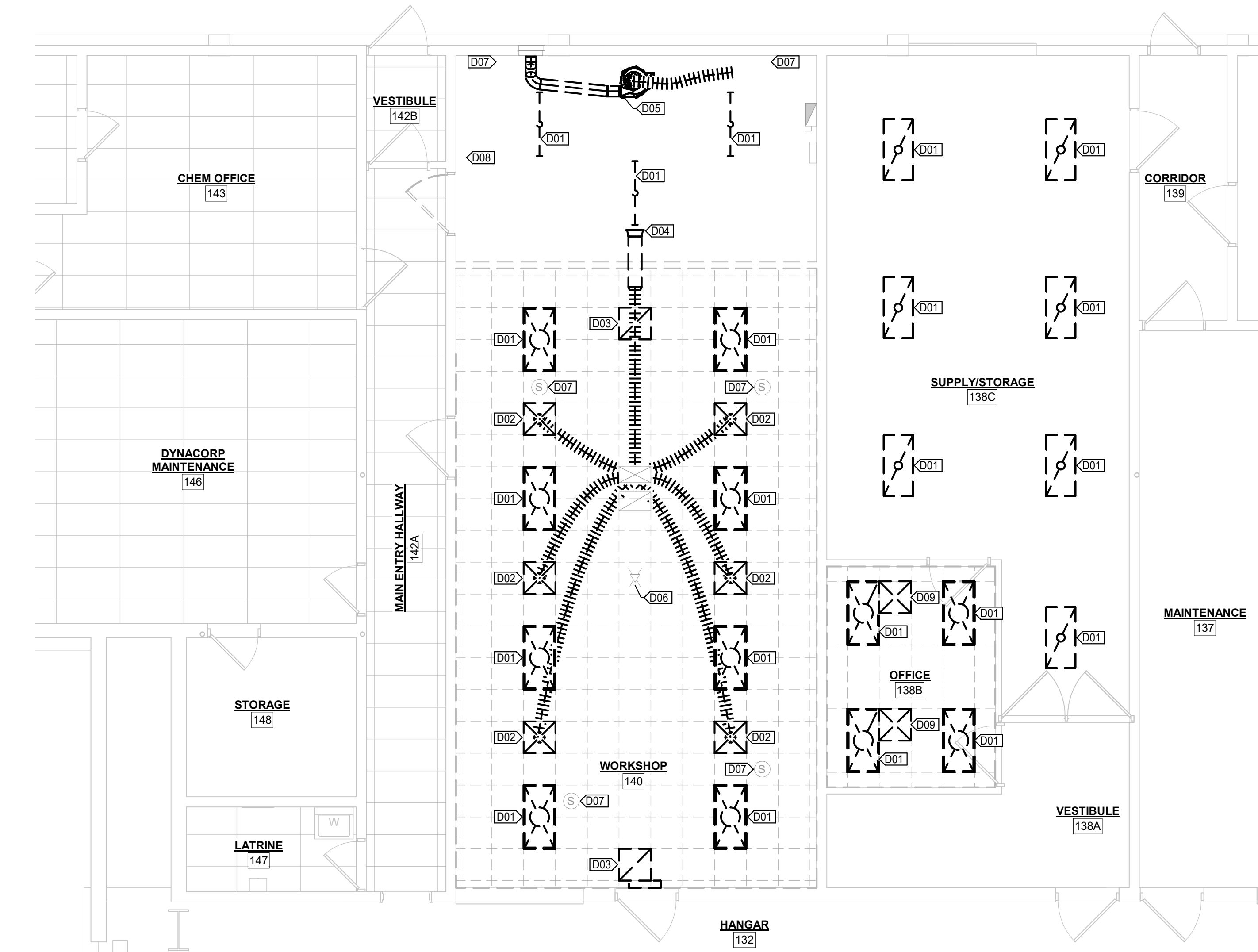
1 DEMOLITION PLAN - AREA A 3/16" = 1'-0"
