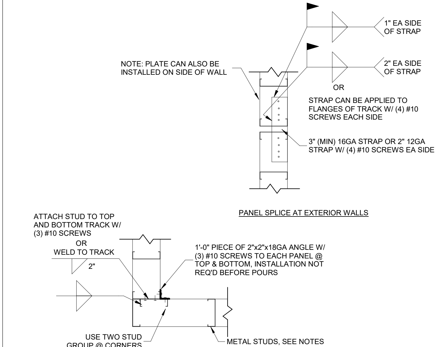
6 CORNER STUDS & PANEL SPLICE @ EXT WALL 1" = 1'-0"
