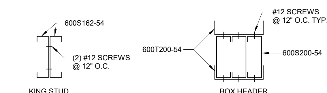
8 TYP. BUILD UP MEMBERS 1 1/2" = 1'-0"
