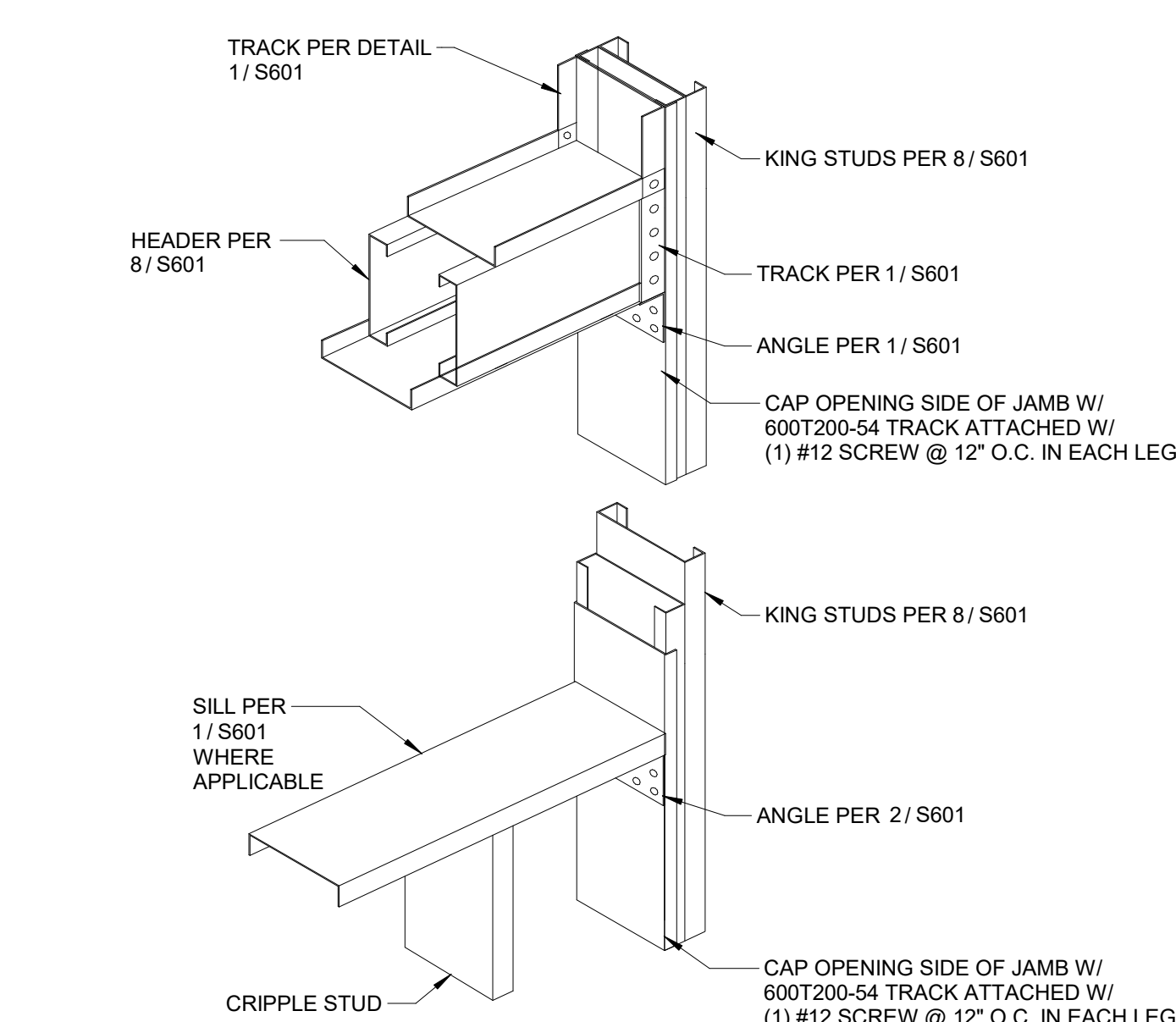
7 HEADER/SILL/KING CONNECTION 1" = 1'-0"
