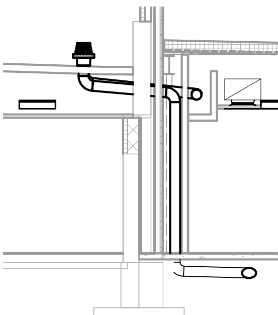
2 OPS CENTER 168 NORTH SECTION 3/16" = 1'-0"
