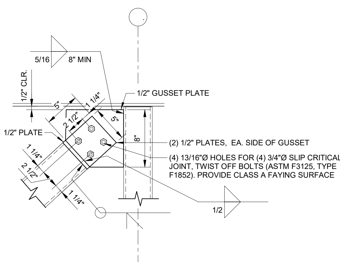
2 TYP. SFRS BRACE CONNECTION 1 1/2" = 1'-0"
