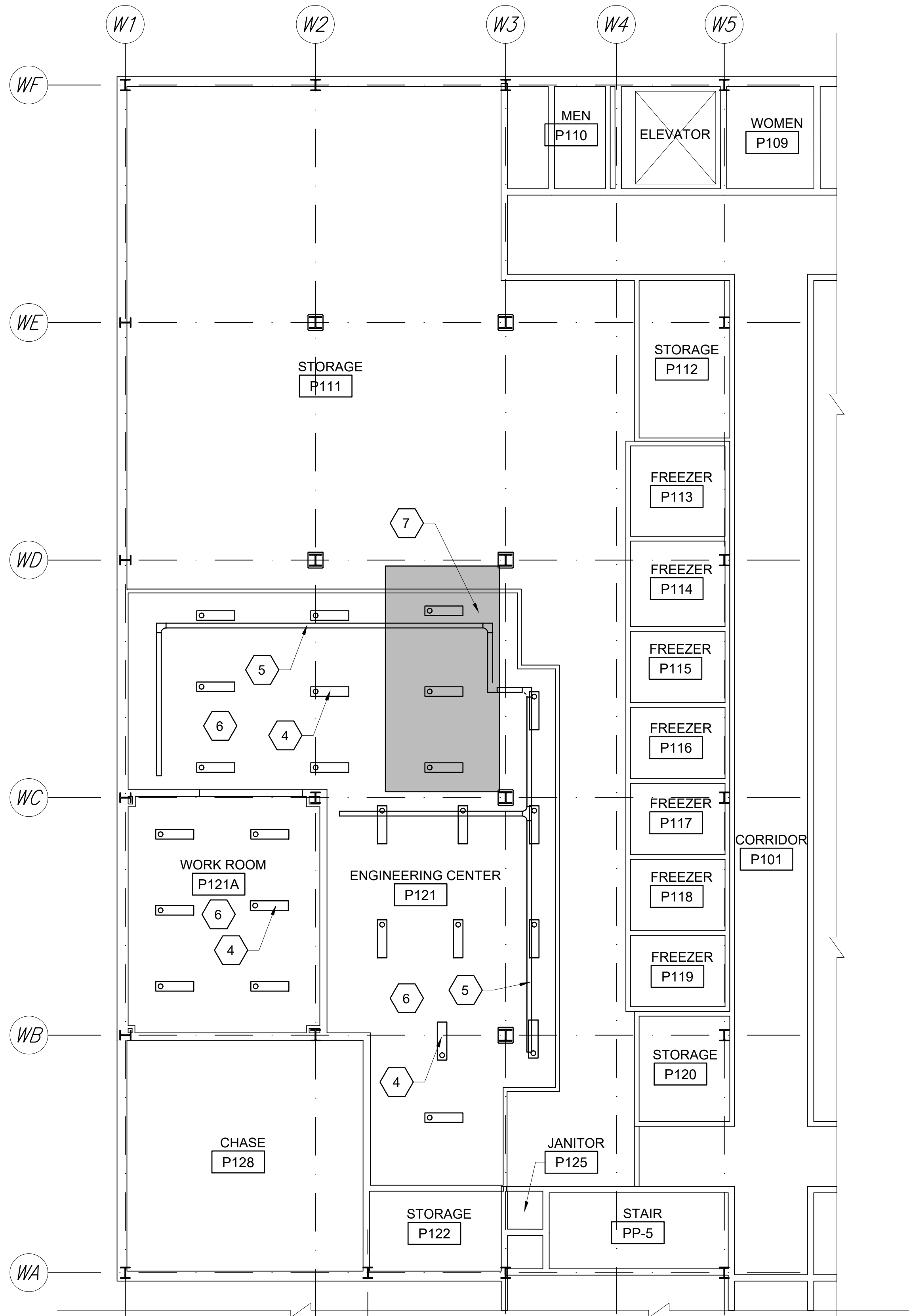
2 BUILDING 1 PARTIAL REFLECTED CEILING PLAN A-101 SCALE: 1/8"= 1'-0"
