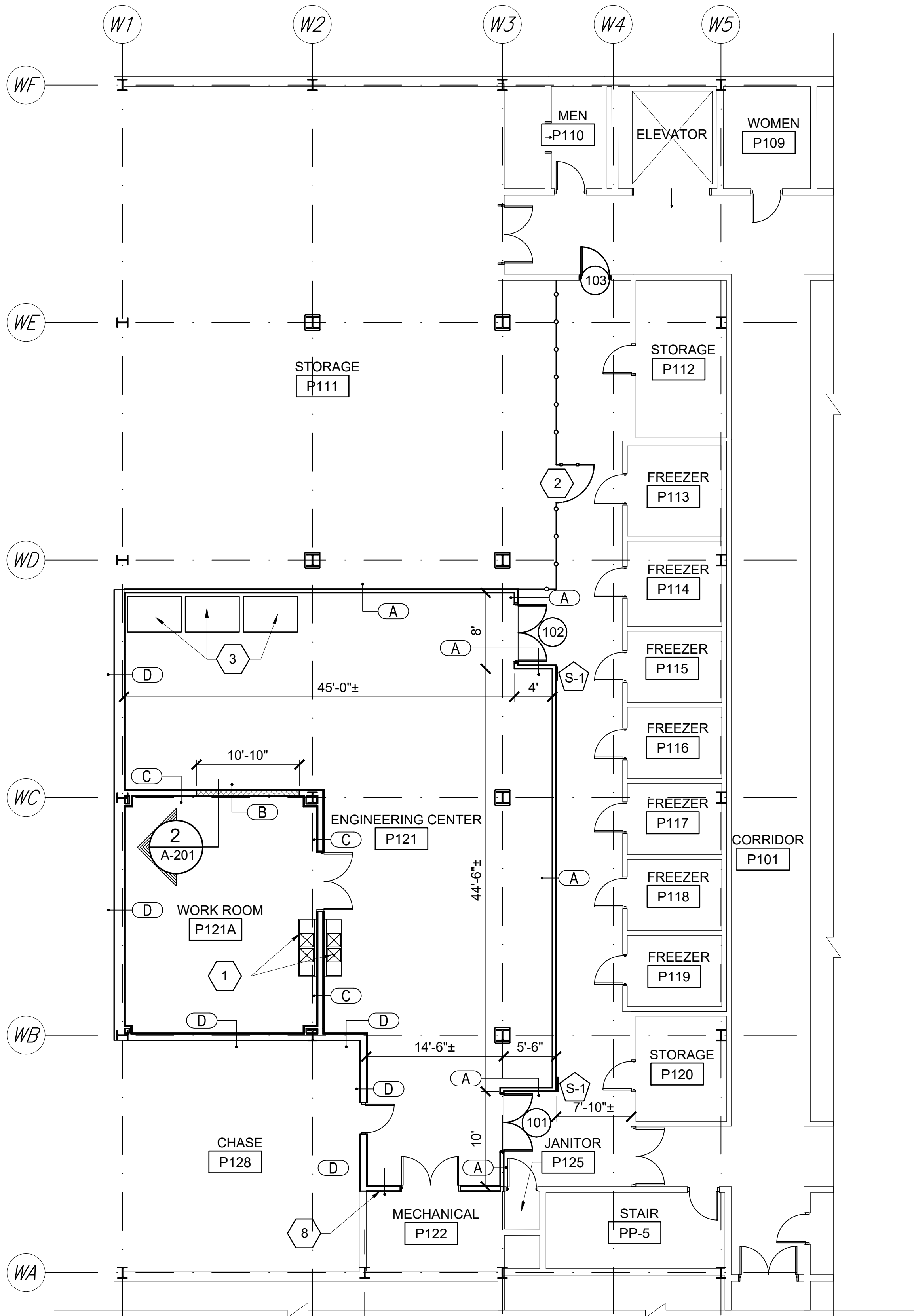
1 BUILDING 1 PARTIAL FLOOR PLAN A-101 SCALE: 1/8"= 1'-0"
