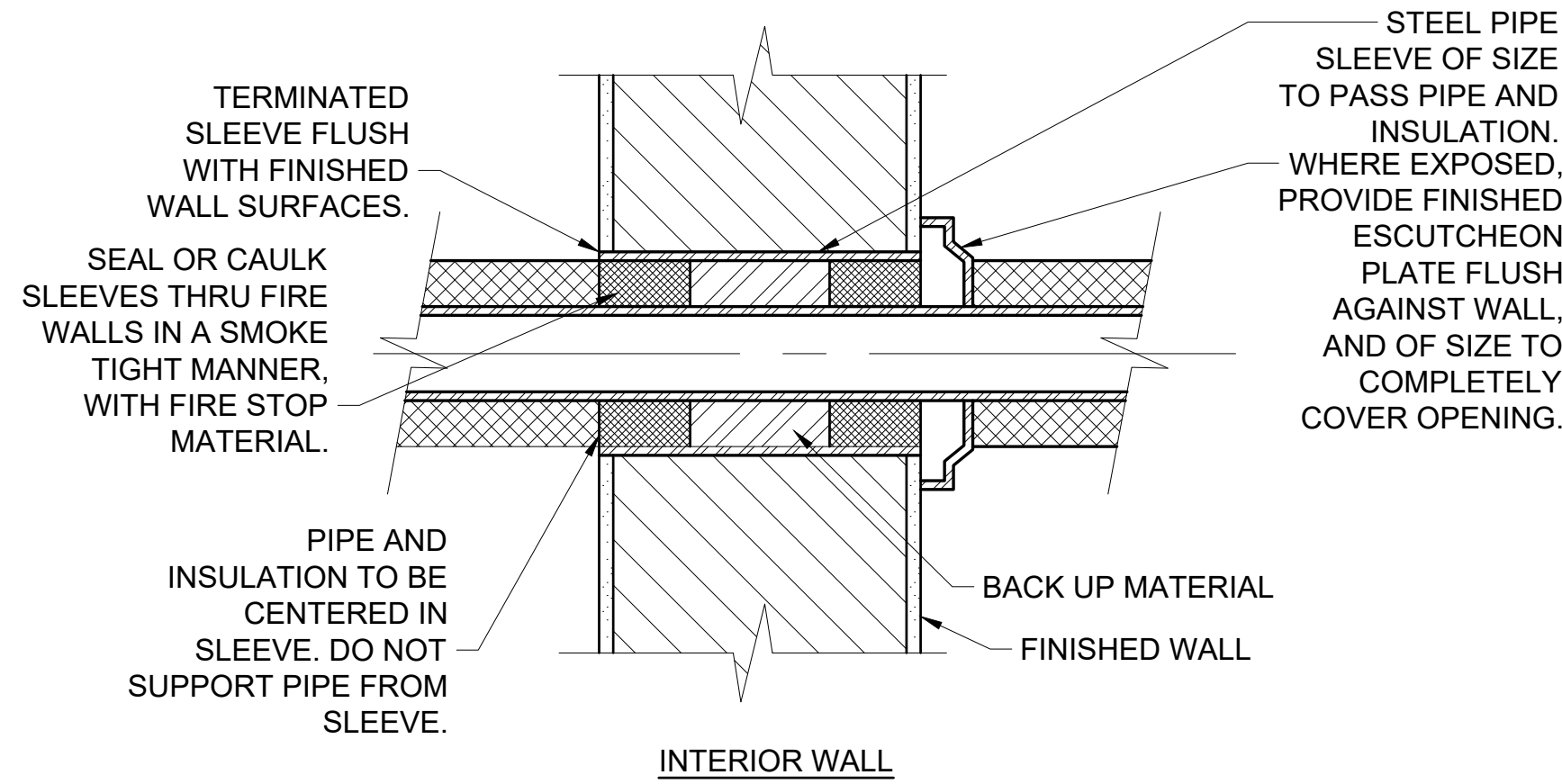
2 TYPICAL PIPE SLEEVES THRU WALLS P-601 SCALE: NOT TO SCALE
