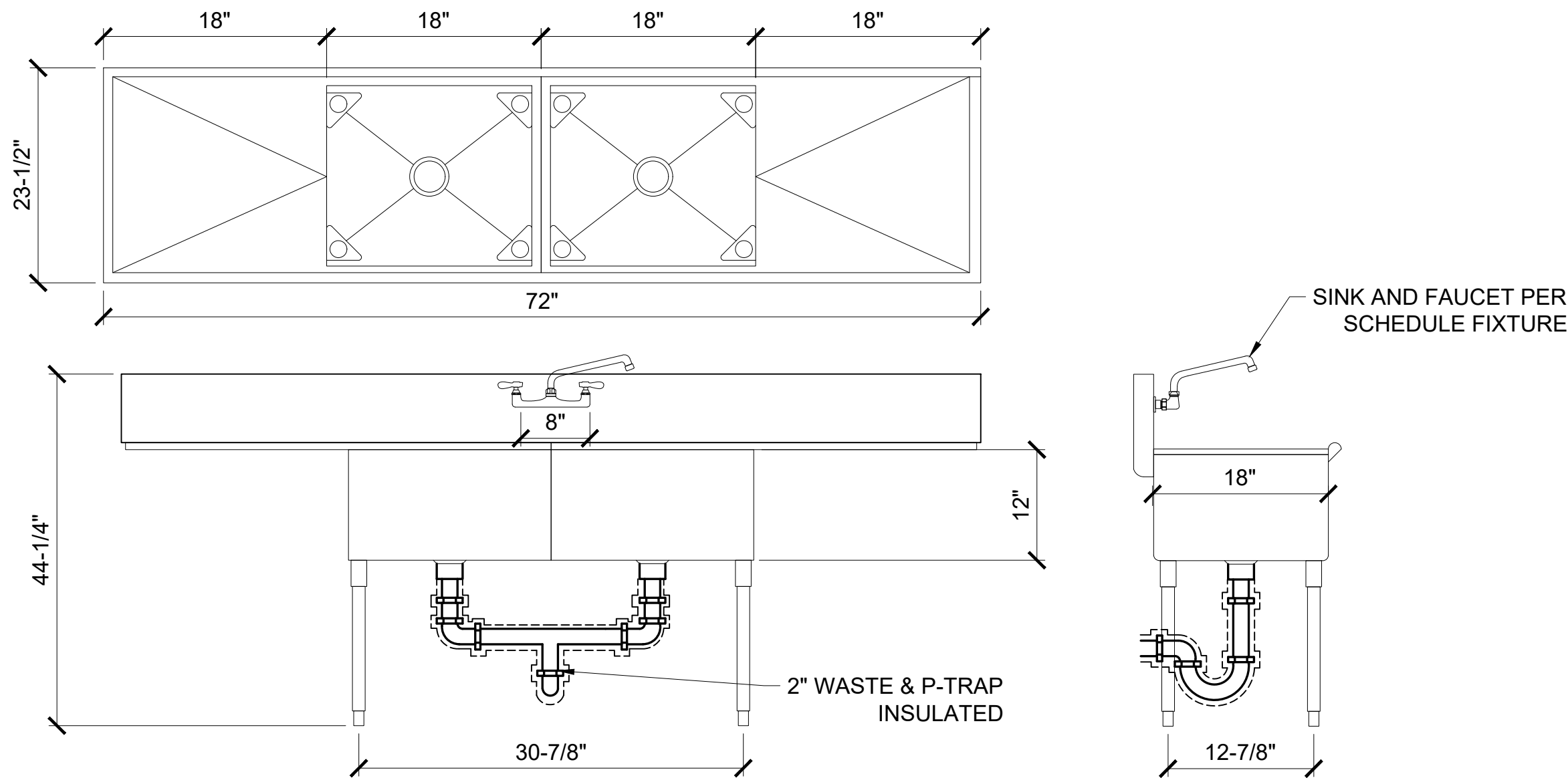
1 SERVICE SINK DETAIL P-601 SCALE: NOT TO SCALE
