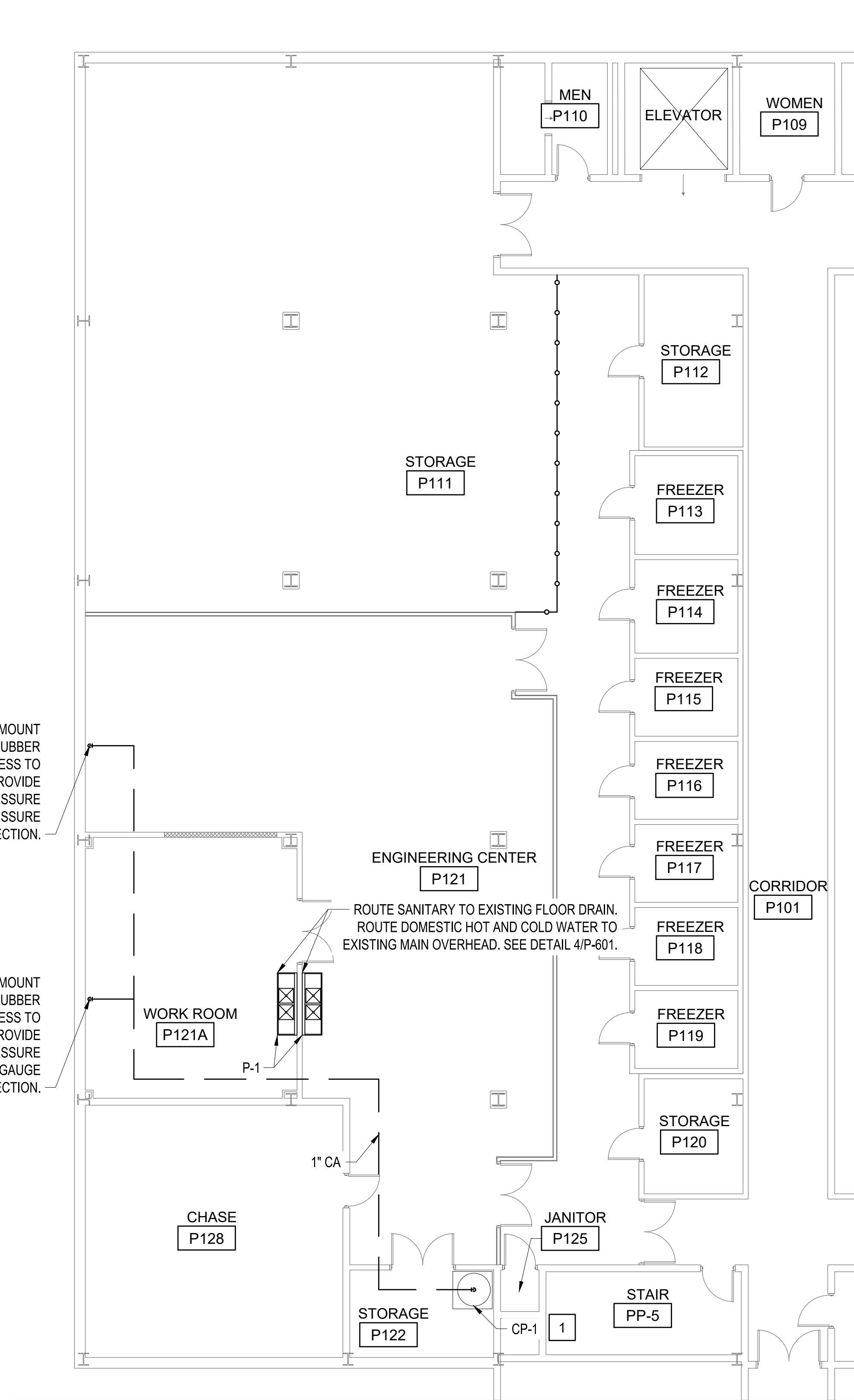
1 P-101 BUILDING 1 PARTIAL PLUMBING FLOOR PLAN SCALE: 1/8"= 1'-0"
