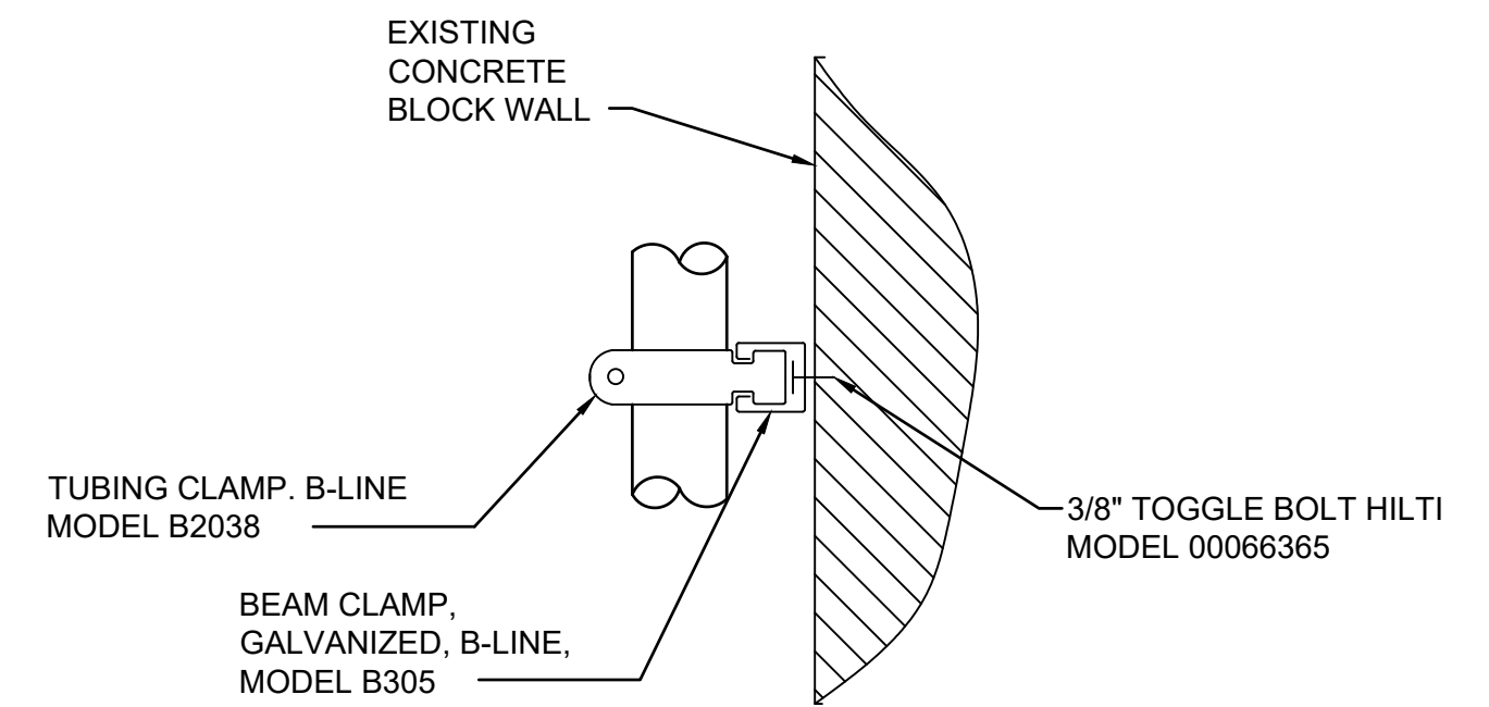
3 TYPICAL PIPE SUPPORT DETAIL P-601 SCALE: NOT TO SCALE
