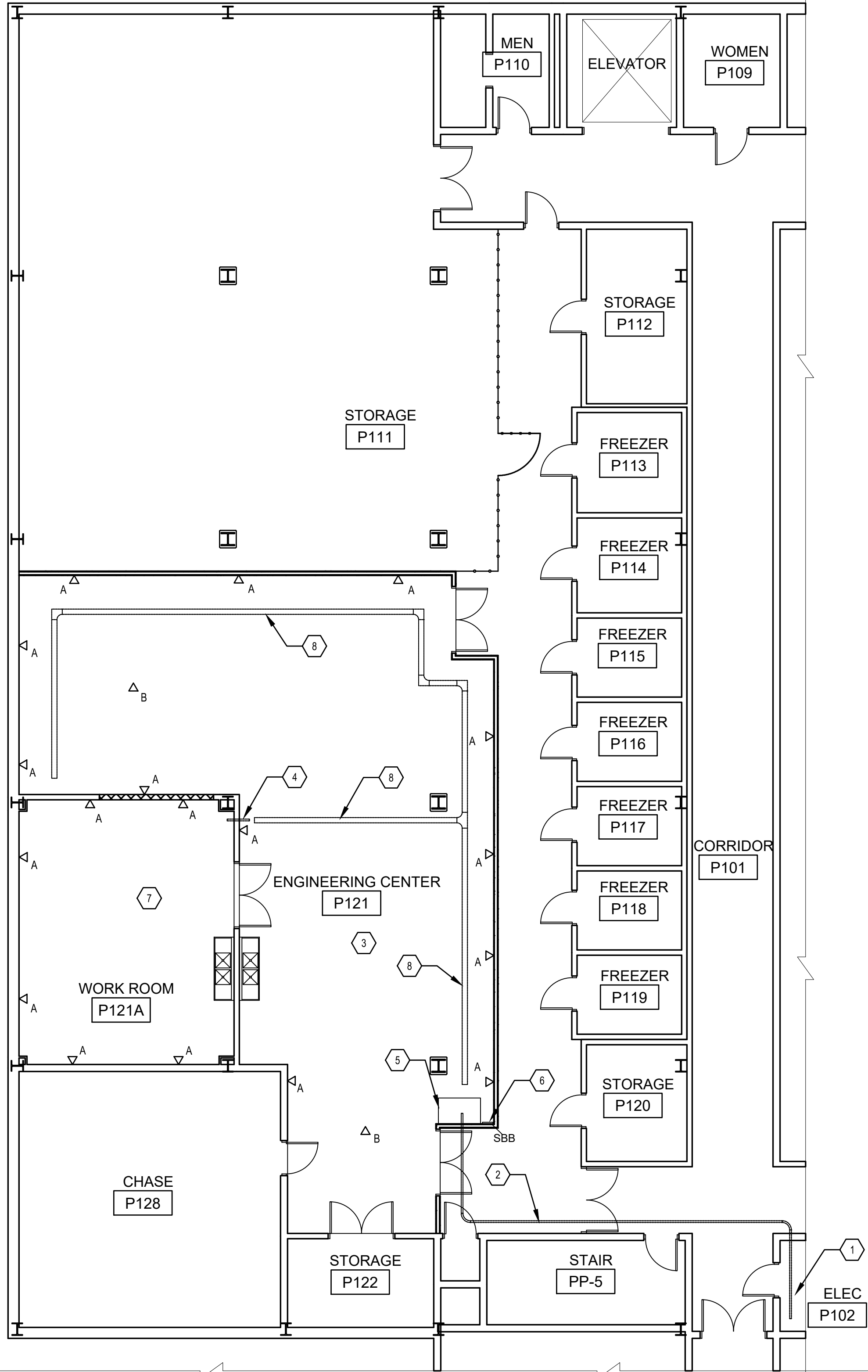
1 TELECOMMUNICATIONS PLAN T-101 SCALE: 1/8"= 1'-0"
