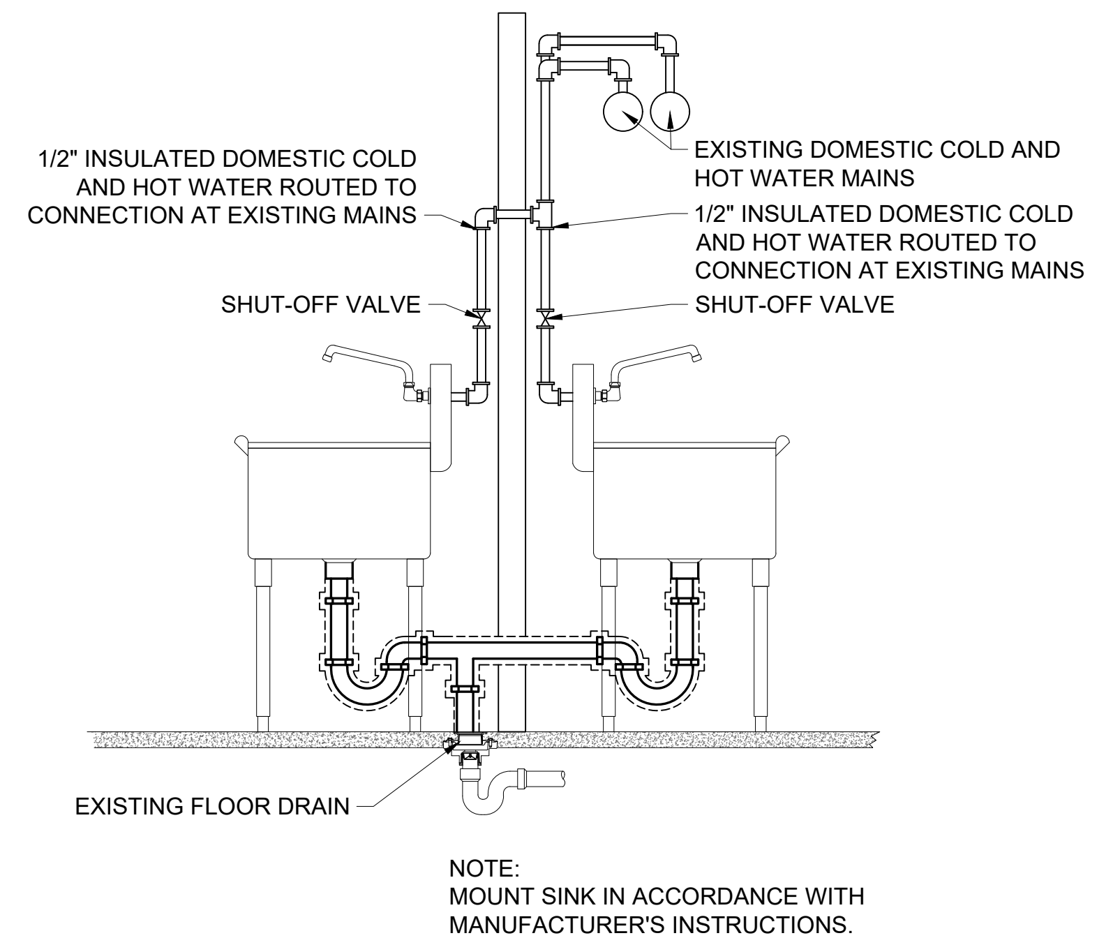
6 SERVICE SINK WASTE CONNECTION DETAIL P-601 SCALE: NOT TO SCALE
