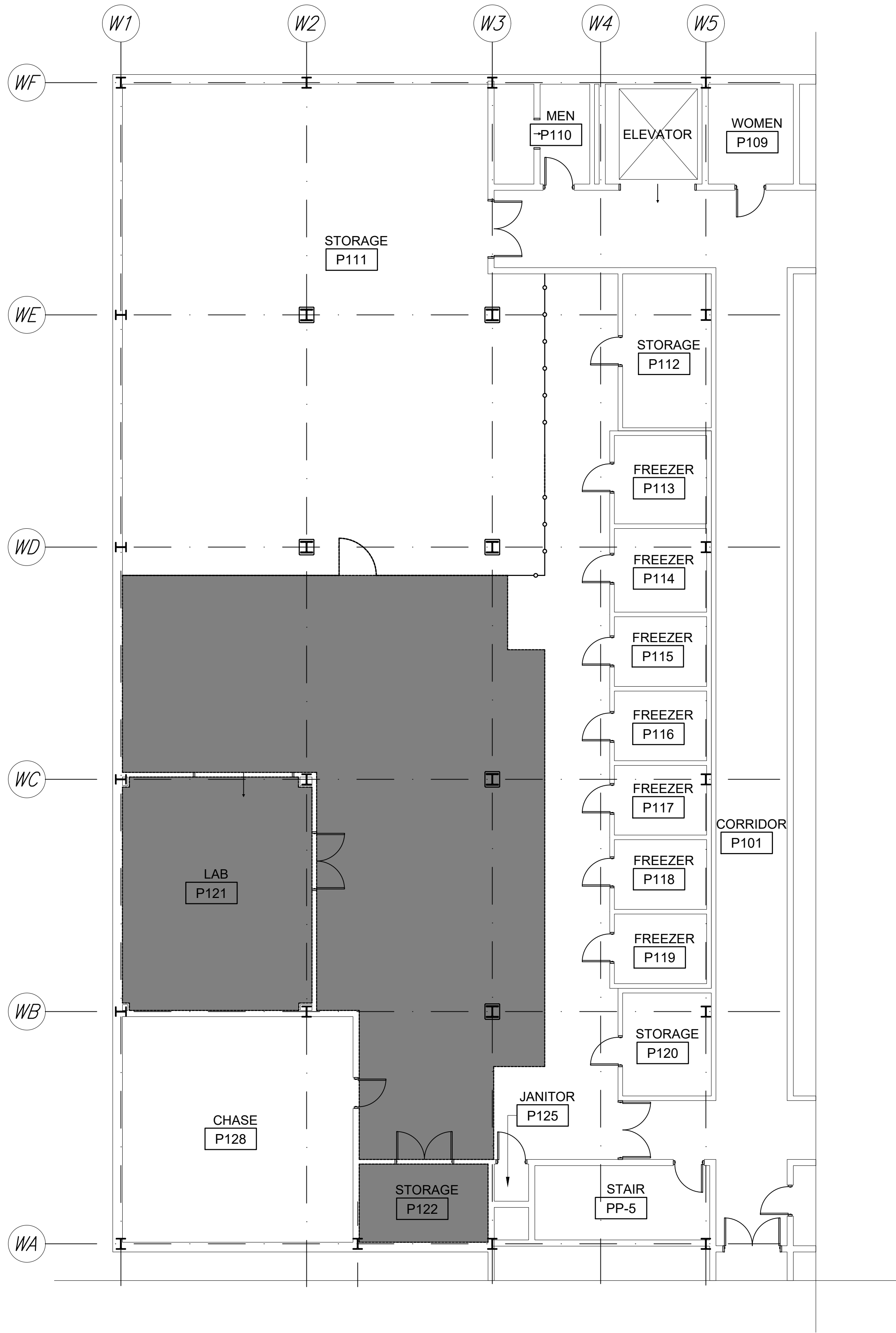
PARTIAL FIRST FLOOR PLAN - HAZARDOUS MATERIALS SCALE: 1/4"= 1'-0"
