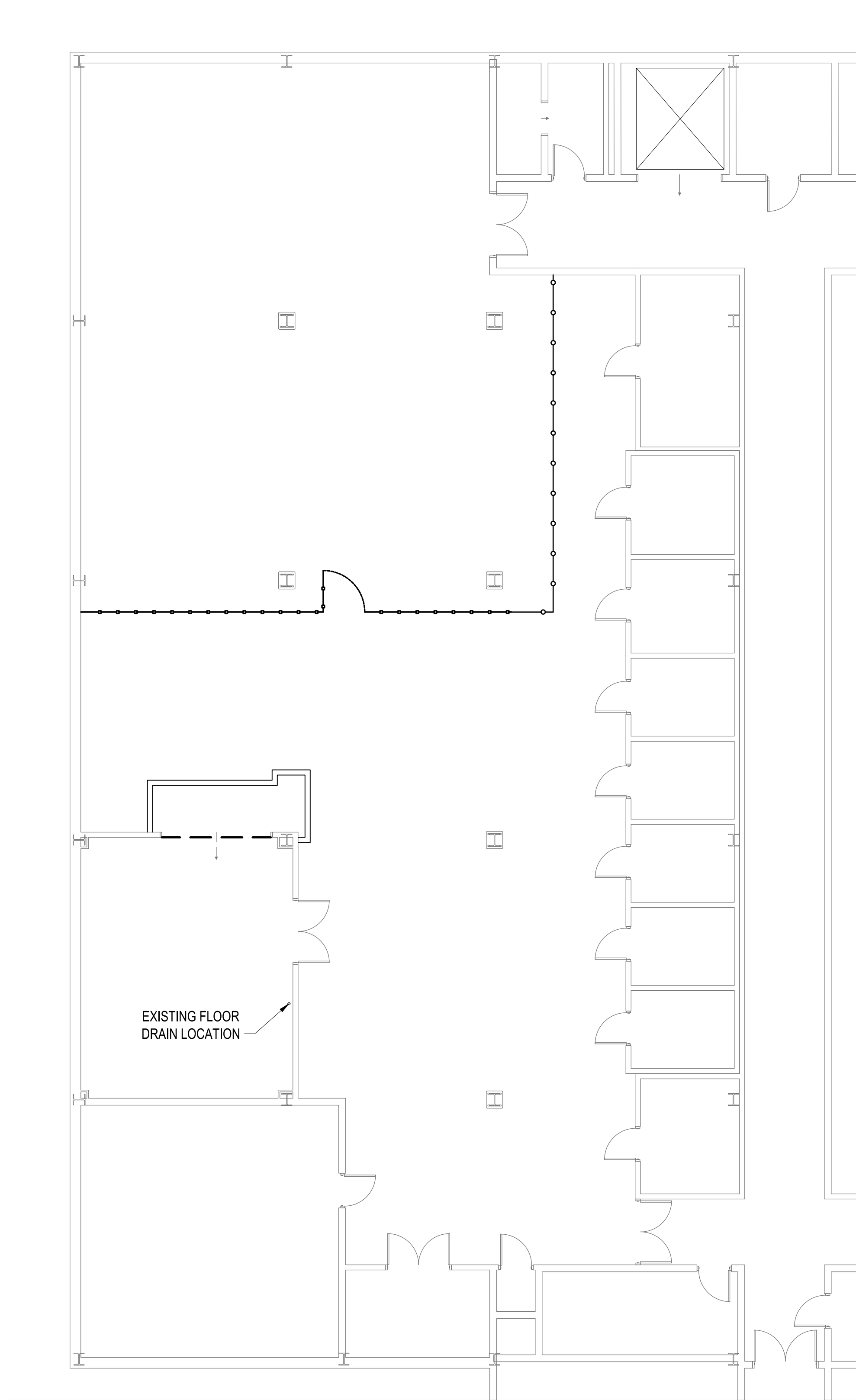
1 P-101 BUILDING 1 PARTIAL PLUMBING EXISTING FLOOR PLAN SCALE: 1/8"= 1'-0"
