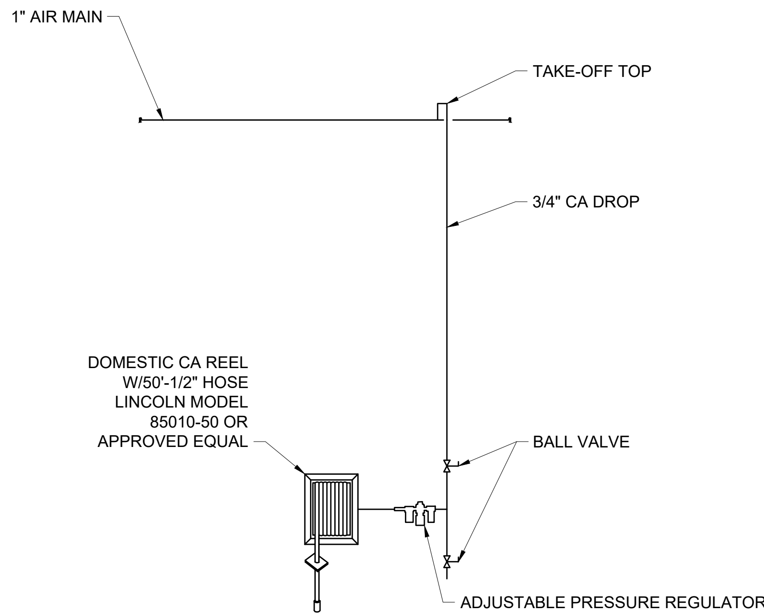
5 TYPICAL HOSE REEL INSTALLATION P-601
