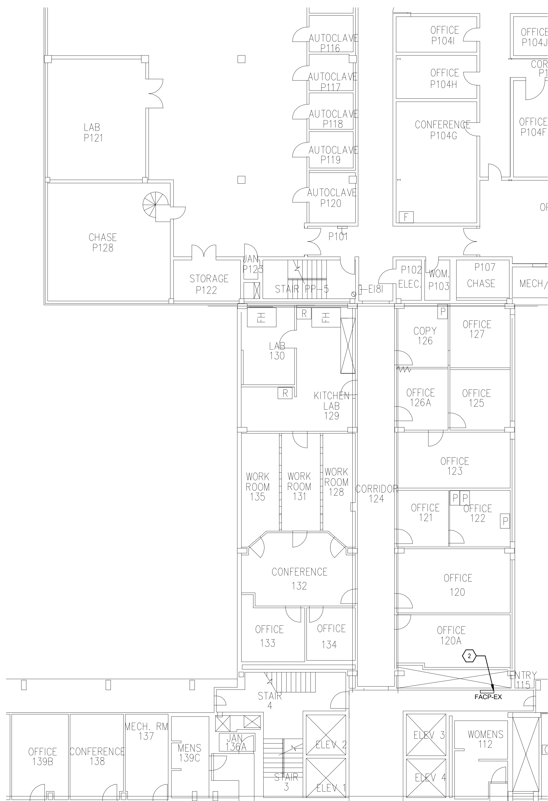
2 FIRE ALARM EXISTING FACP LOCATION F-102 SCALE: 3/32"= 1'-0"
