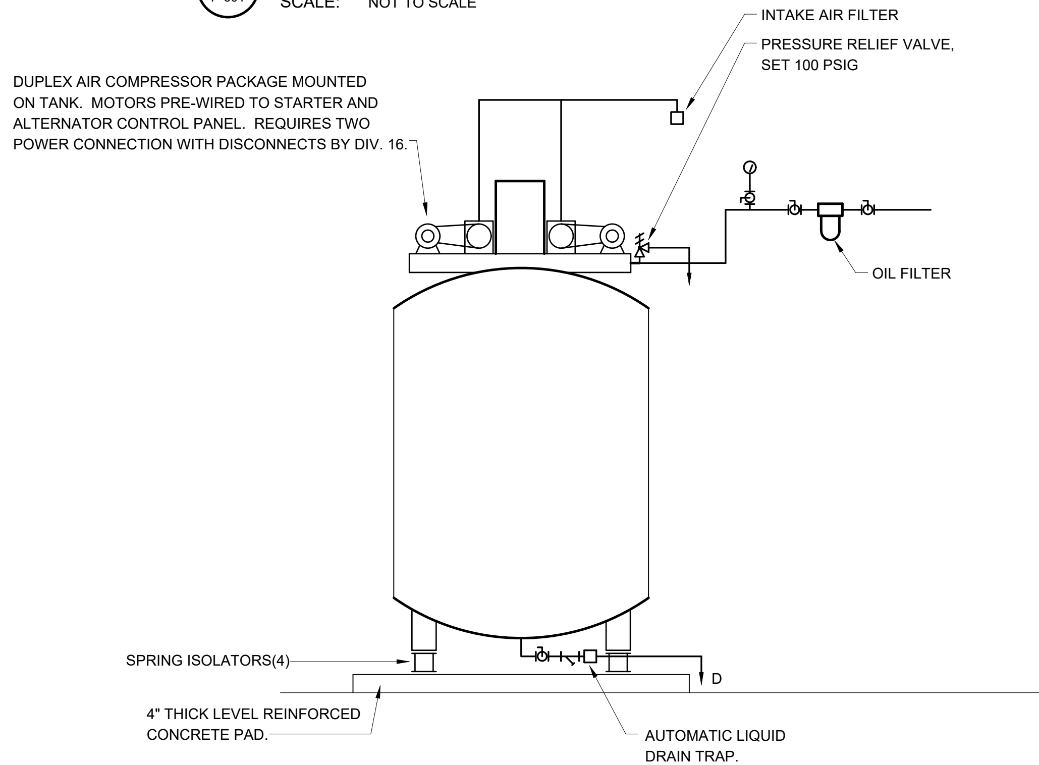
4 AIR COMPRESSOR DETAIL P-601 SCALE: NOT TO SCALE
