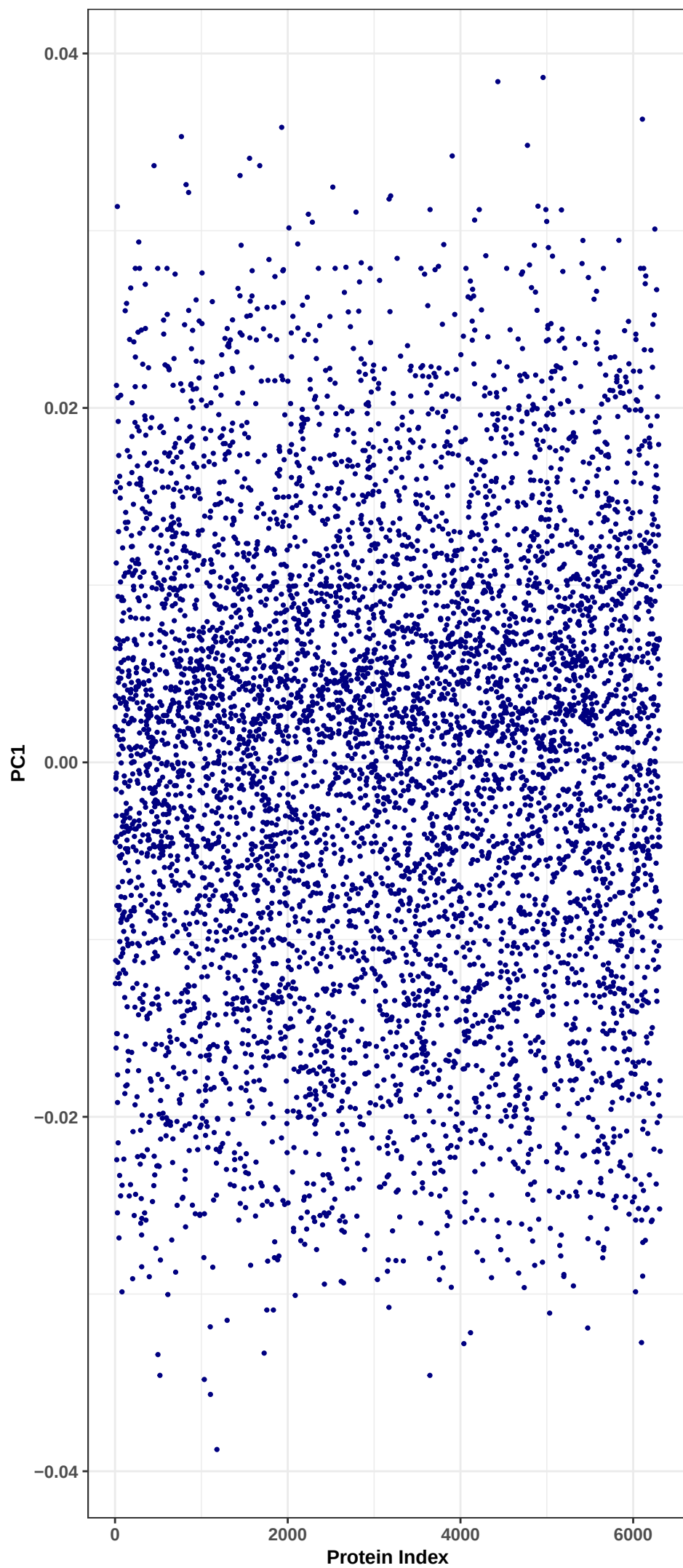
Distribution of PC1 from PCA of the Gaussian Spectral Embedding (k = 1; PC1
