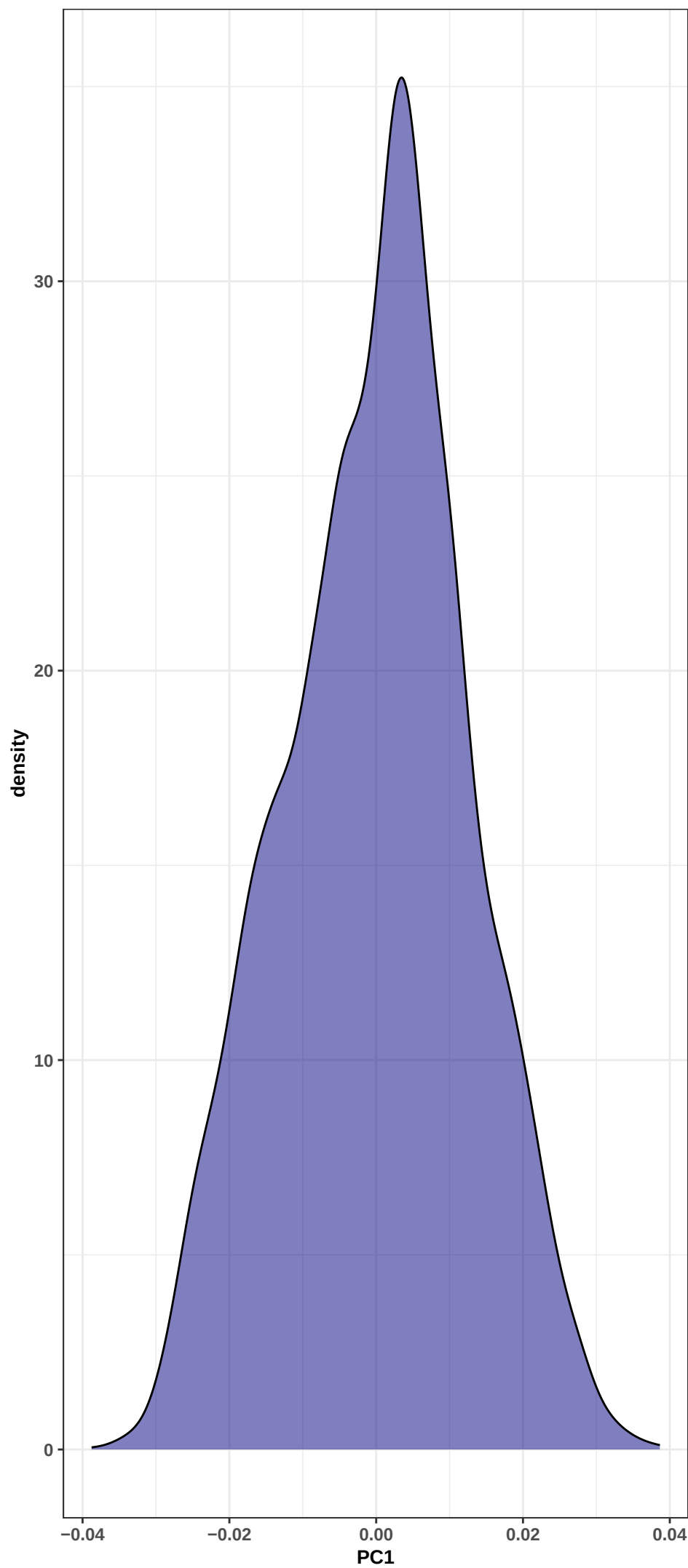
Density of Protein PC1 values from PCA of the Gaussian Spectral Embedding (k = 1; PC1)
