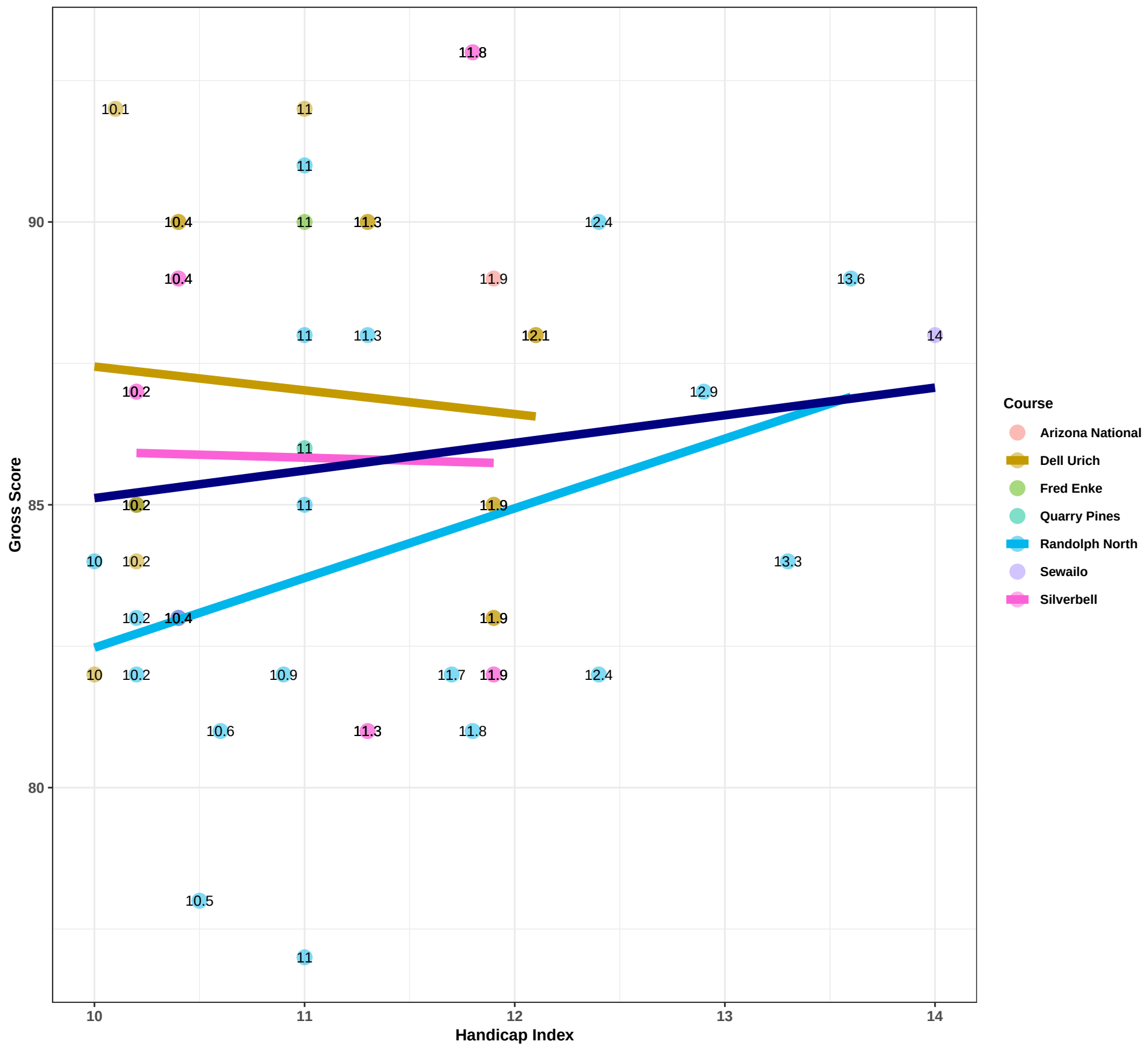
Gross Score vs Handicap Index from 2025-05-04 – present (removing outlier 72) as of 2026-07-21
