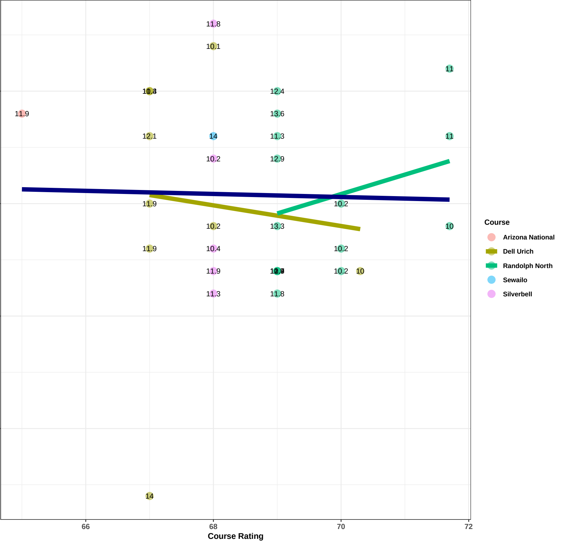
Gross Score vs Course Difficulty from 2025-05-04 – present as of 2026-05-09
