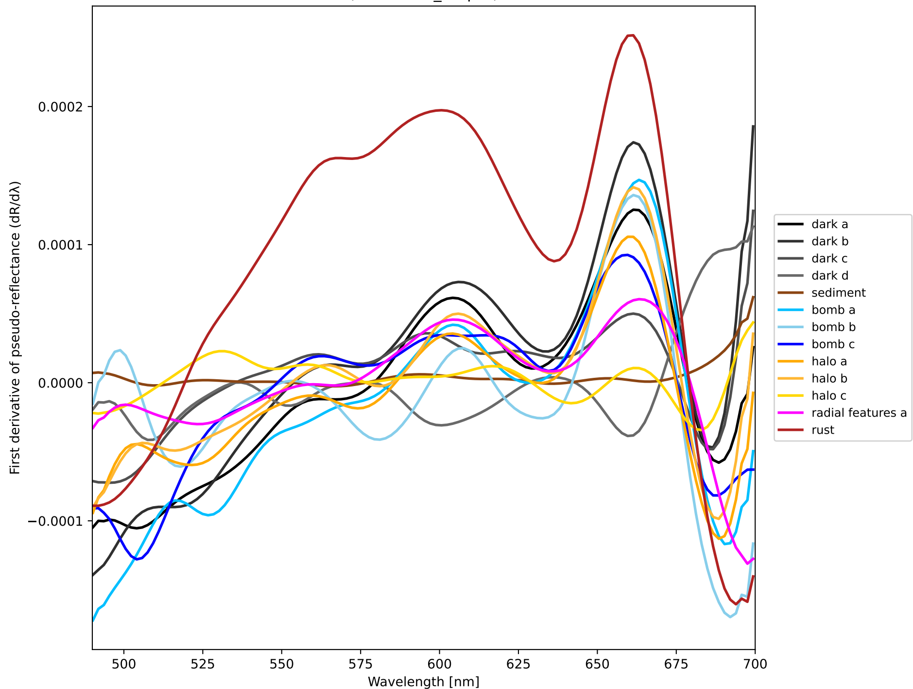
Corrected ROI Spectra (490-700nm) [1st Derivative] (L2) (MA: 2) (Combined_output)
