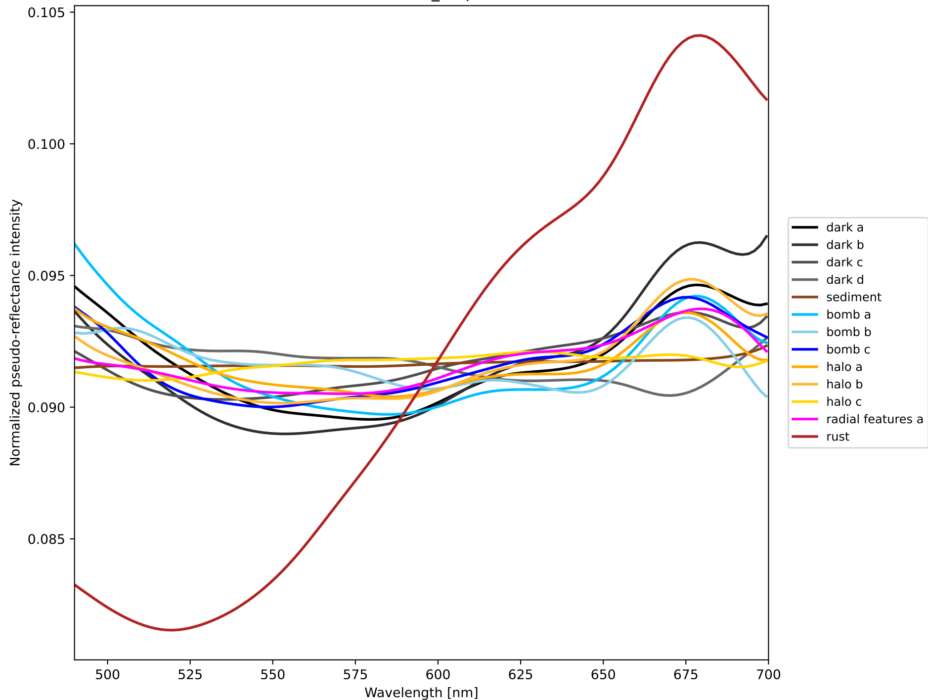
Corrected ROI Spectra (490-700nm) (L2) (MA: 2) (Combined_output)
