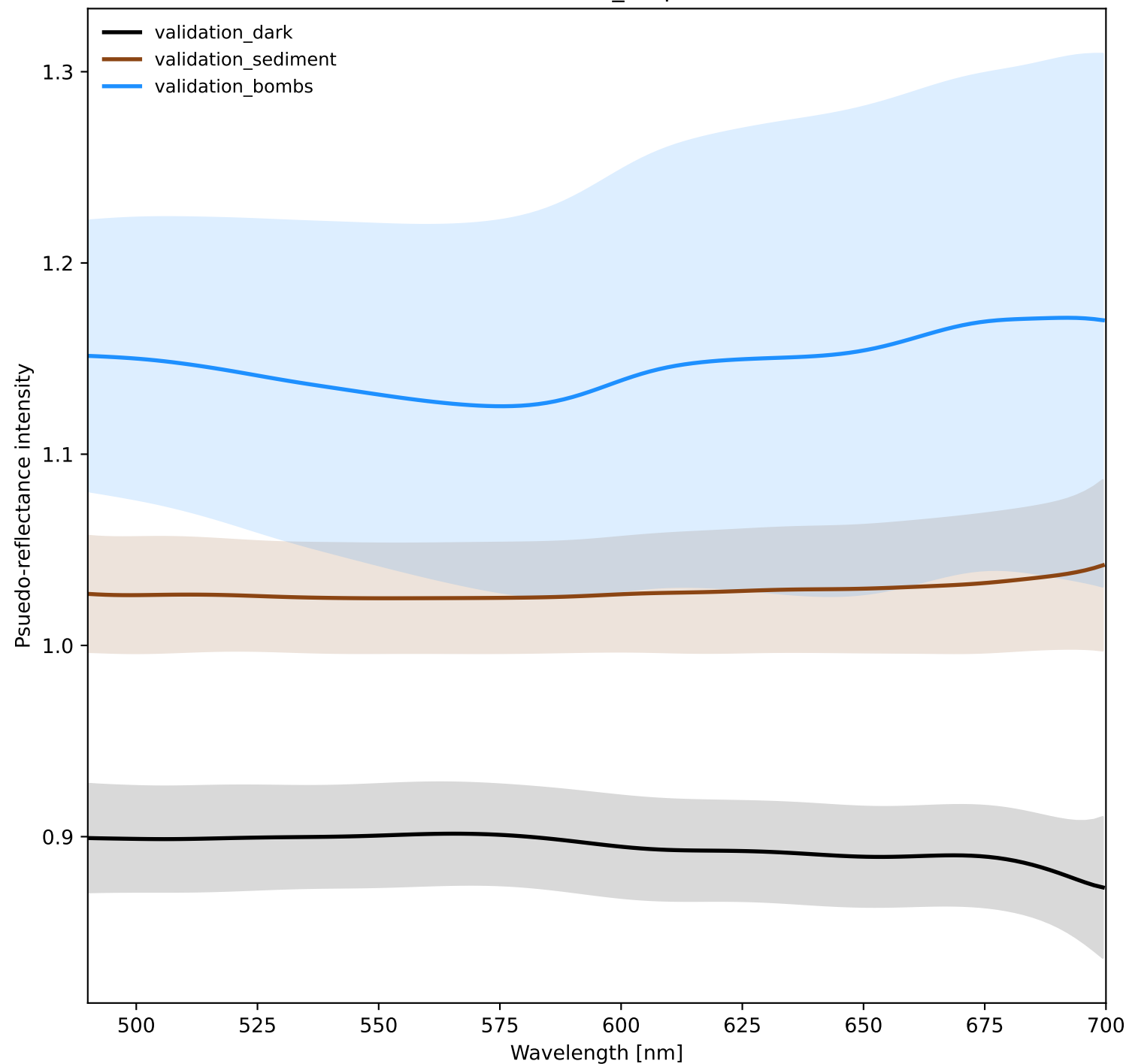
Corrected ROI Spectra (490-700nm) (Combined_output)
