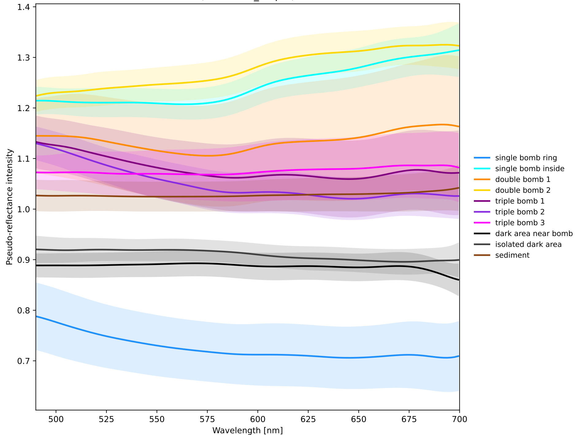
Corrected ROI Spectra (490-700nm) (MA: 2) (Combined_output)
