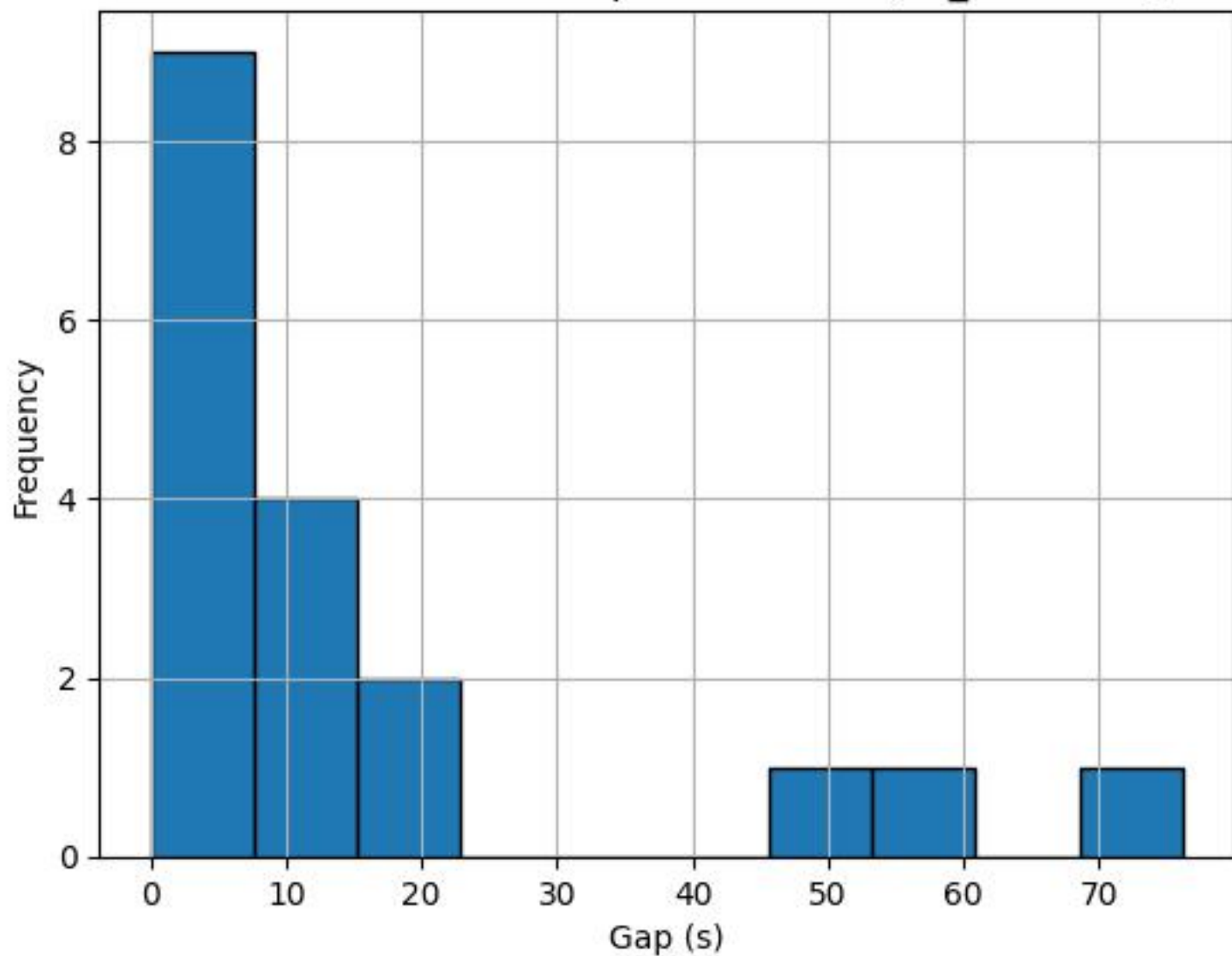
First Retransmission Gap Distribution (4G_Mahimahi)
