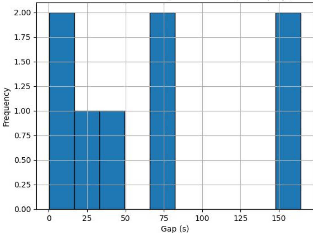
First Retransmission Gap Distribution (CellReplay)
