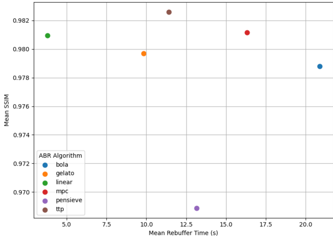
SSIM over Rebuffer for ABRs (VERIZON)
