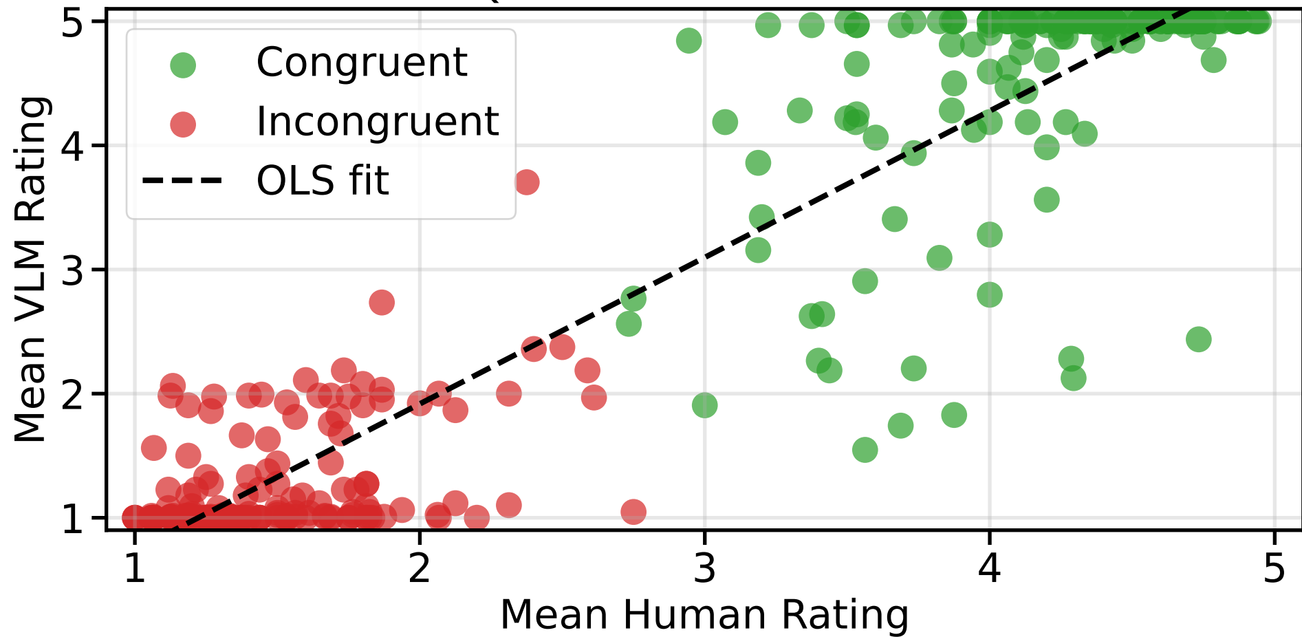
Qwen3-VL-32B-Instruct
