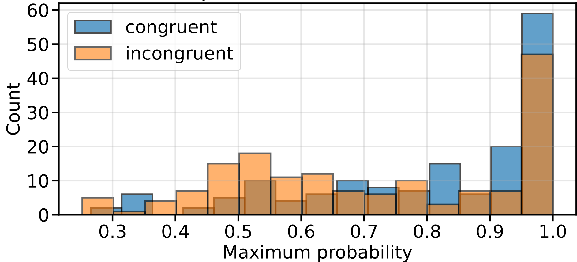
Qwen3-VL-30B-A3B-Instruct
