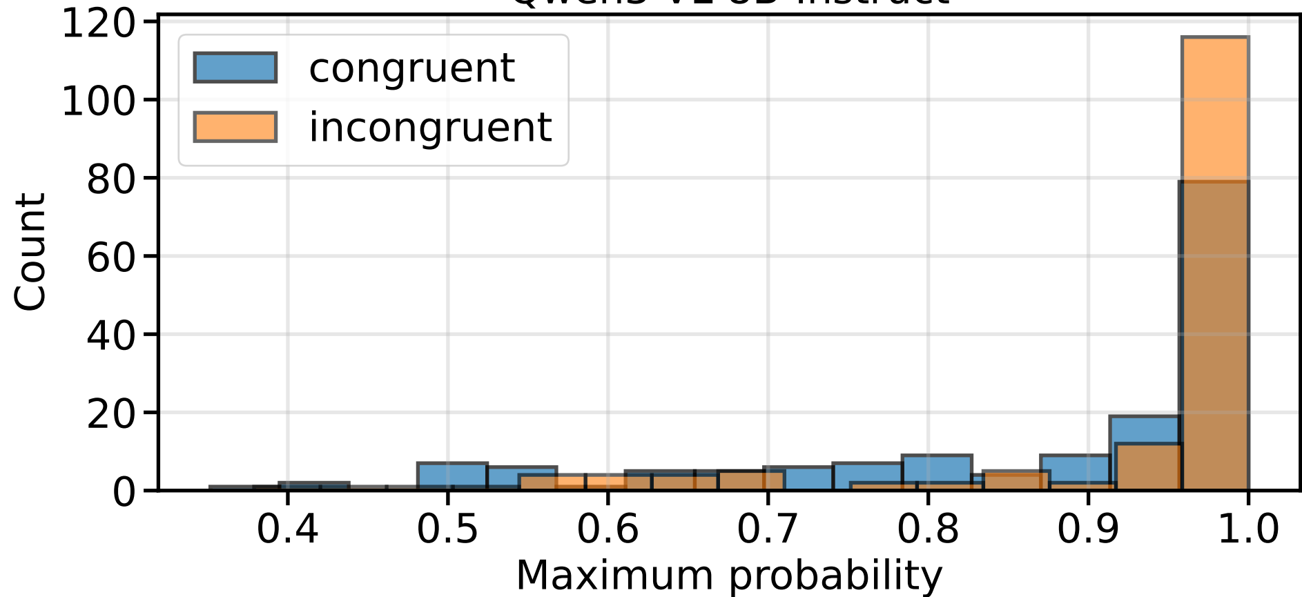
Qwen3-VL-8B-Instruct
