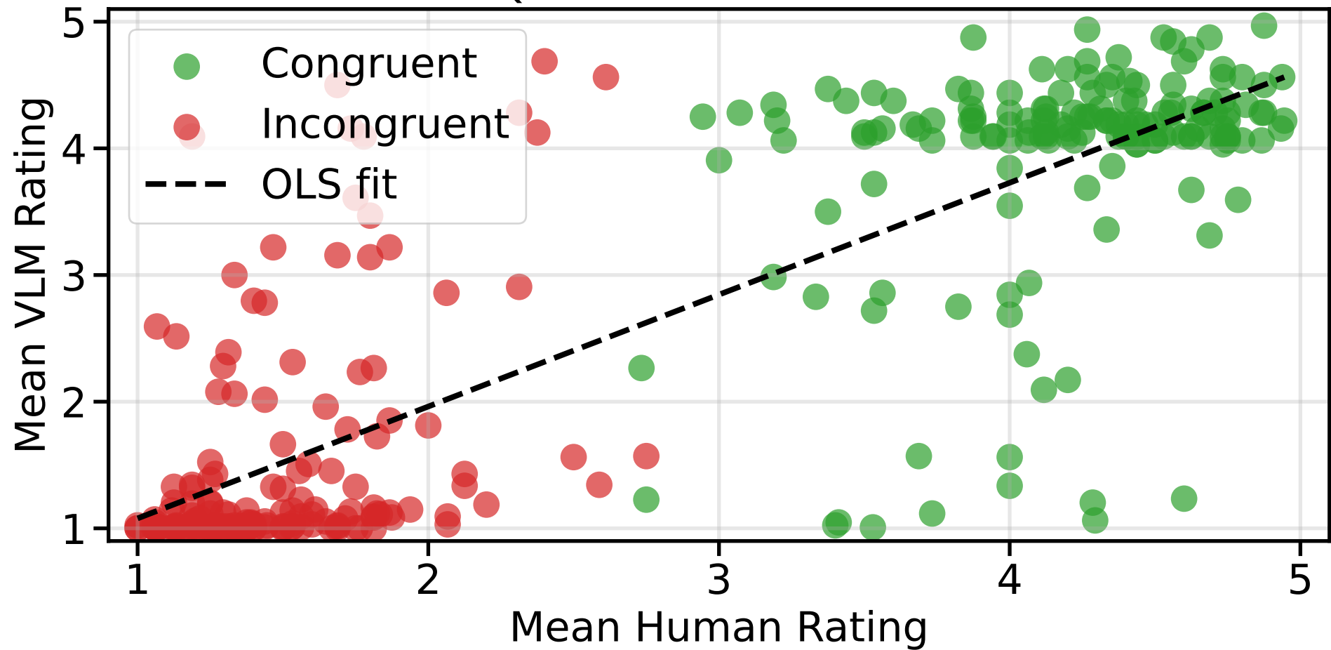
Qwen3-VL-2B-Instruct
