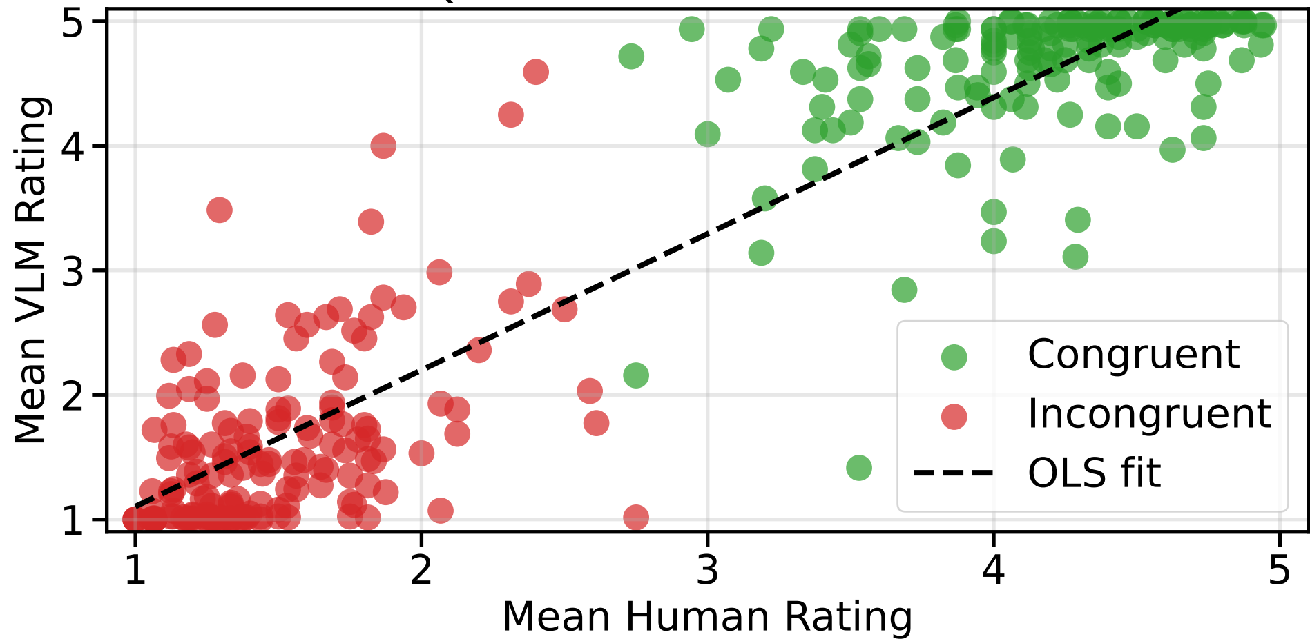
Qwen3-VL-30B-A3B-Instruct
