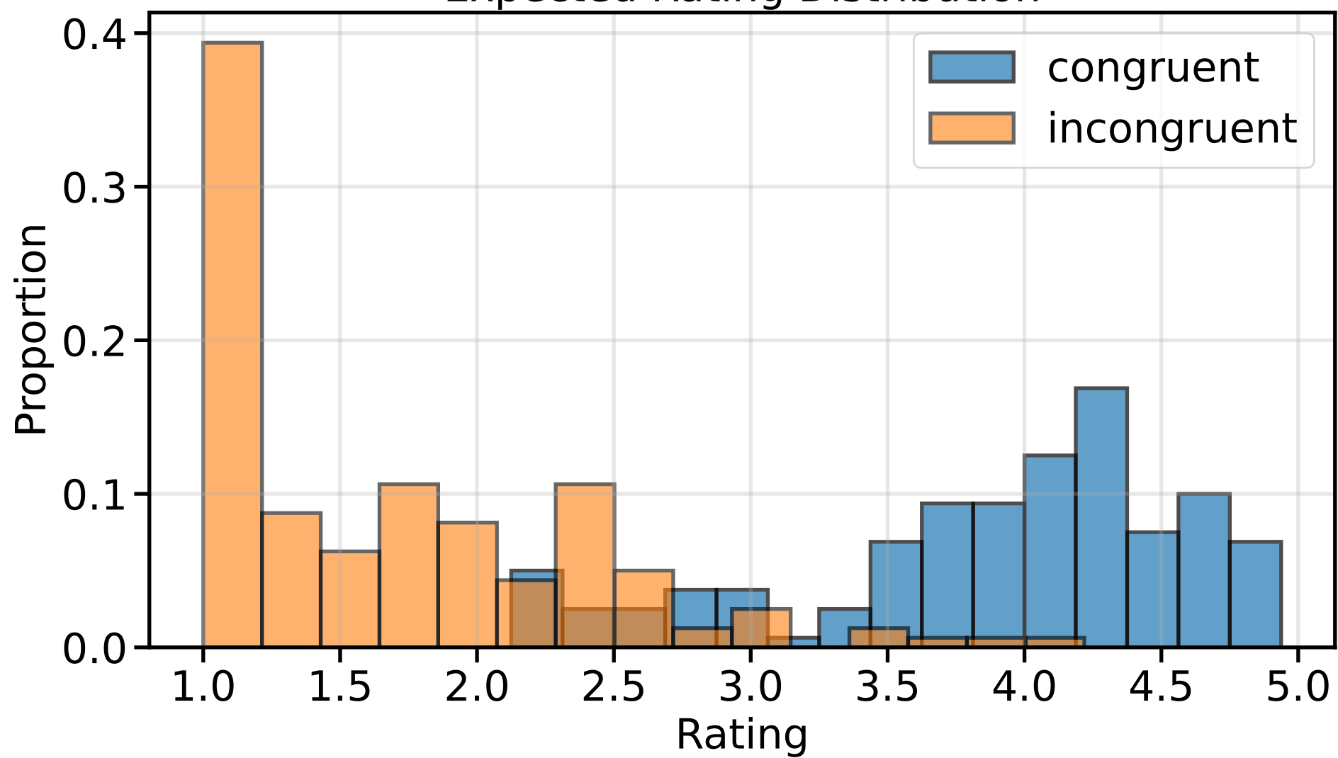
Expected Rating Distribution
