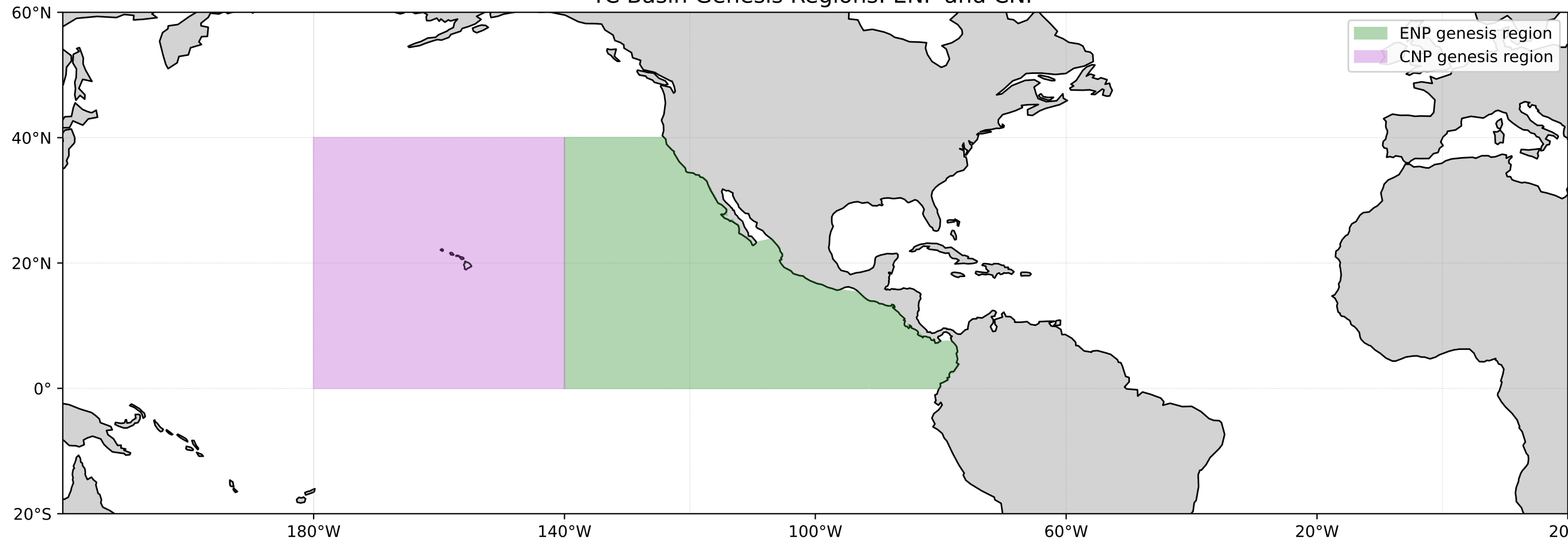
TC Basin Genesis Regions: ENP and CNP
