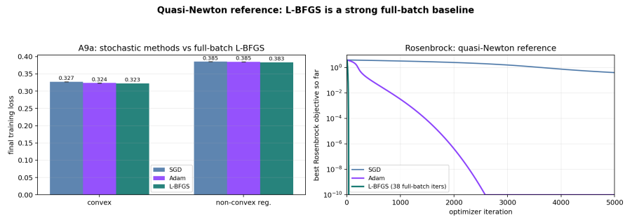
Figure 6: L-BFGS reference. On A9a, L-BFGS reaches comparable final losses. On Rosenbrock, it solves the benchmark in 38 full-batch iterations, illustrating why it should be interpreted as a separate deterministic reference rather than as a mini-batch competitor.
