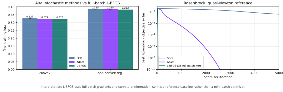
Figure 6: L-BFGS reference. On A9a, L-BFGS reaches comparable final losses. On Rosenbrock, it solves the benchmark in 38 full-batch iterations, illustrating why it should be interpreted as a separate deterministic reference rather than as a mini-batch competitor.
