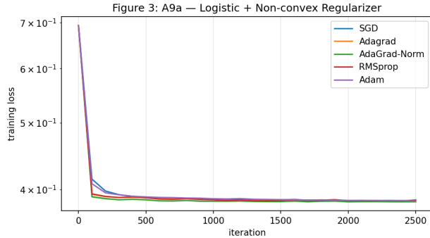
(a) A9a non-convex regularized loss.
