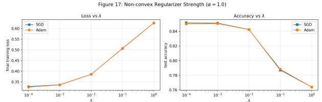
(b) Non-convex regularization strength.
