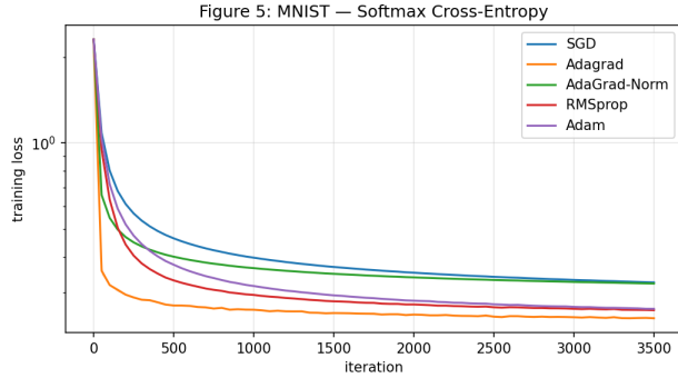
(a) MNIST softmax loss.
