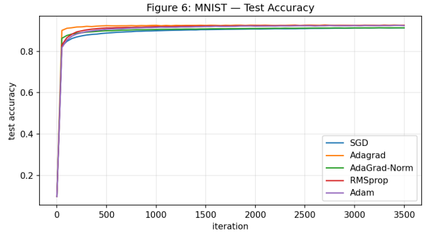
(b) MNIST test accuracy.
