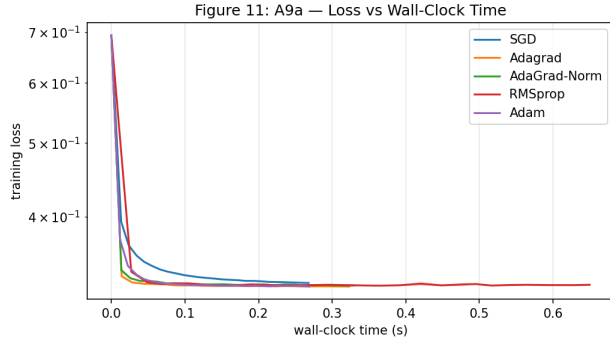
(a) A9a loss against wall-clock time.
