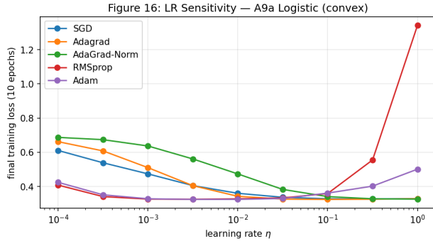
(a) Learning-rate sensitivity on A9a.
