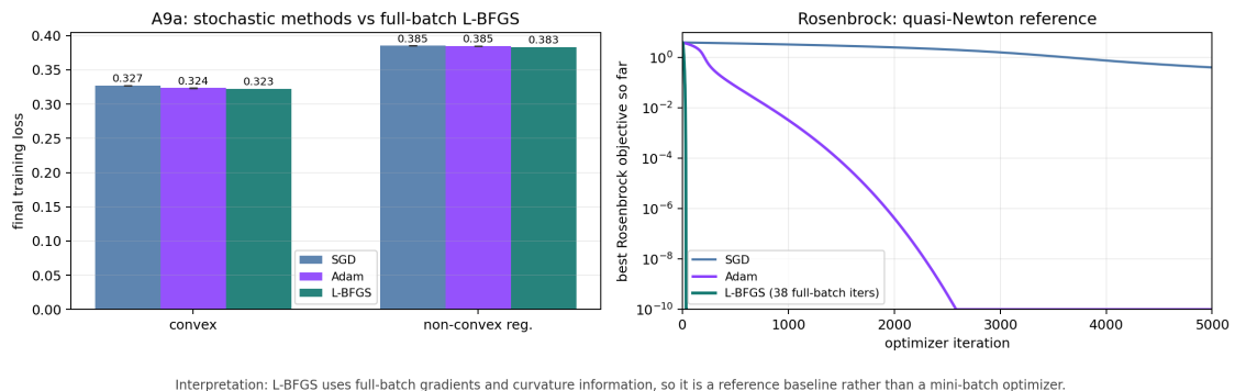
Figure 7: L-BFGS reference. On A9a, L-BFGS reaches comparable final losses. On Rosenbrock, it solves the benchmark in 38 full-batch iterations, illustrating why it should be interpreted as a separate deterministic reference rather than as a mini-batch competitor.
