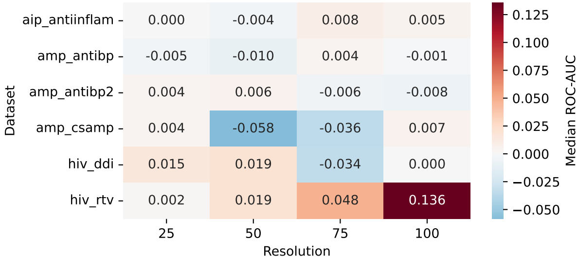
Median ROC-AUC (protein vs 0.5) — CNN
