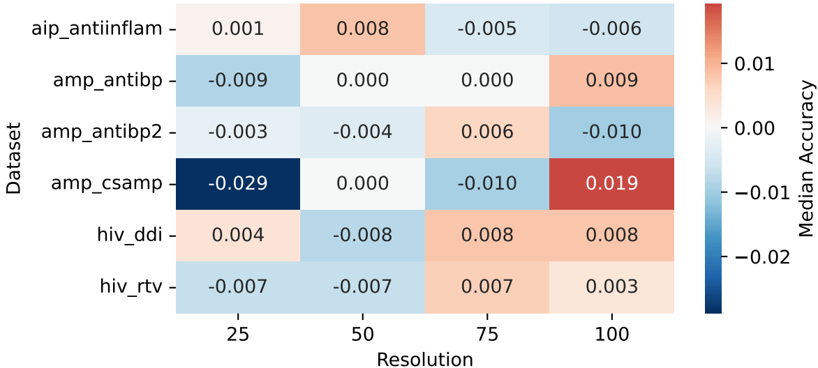
Median Accuracy (protein vs 0.5) — FNN
