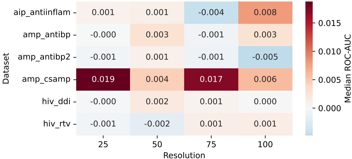
Median ROC-AUC (protein vs 0.5) — FNN
