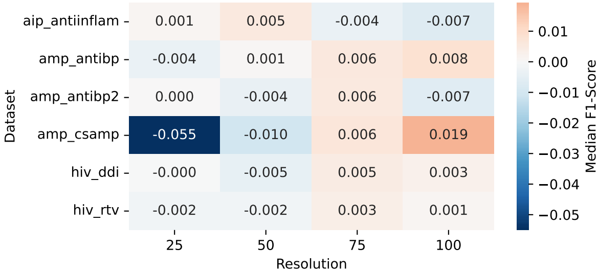
Median F1-Score (protein vs 0.5) — FNN
