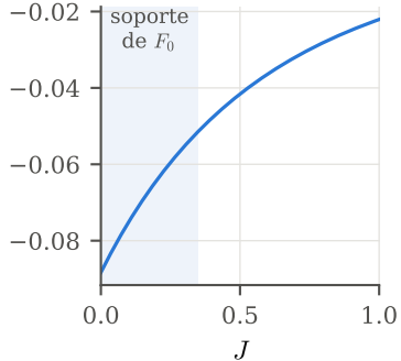
(c) \omega'(J)
