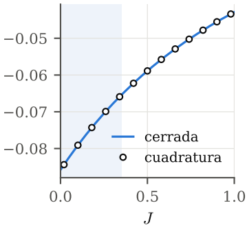
(a) E(J)
